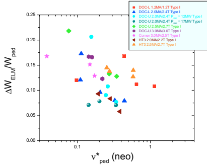
Figure 5. Normalised (to the pedestal energy) Type I ELM energy loss versus pedestal collisionality for the same dataset as Fig. 1.
