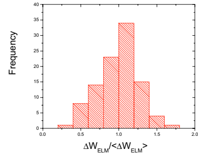
Figure 2. Histogram of the Type I ELM energy loss for a large range of plasma conditions at JET.
