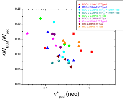
Figure 5. Normalised (to the pedestal energy) Type I ELM energy loss versus pedestal collisionality for the same dataset as Fig. 1.
