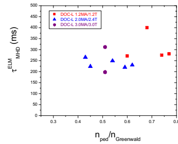
Figure 8. Duration of the ELM (from broadband MHD turbulence analysis) versus pedestal density (normalised to the Greenwald limit) for the some of the discharges in Fig. 1.
