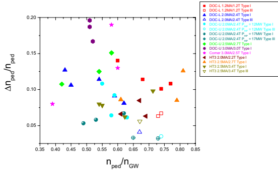
Figure 3. Normalised Type I ELM pedestal density drop versus pedestal density (normalised to the Greenwald limit) for the same dataset as Fig. 1.
