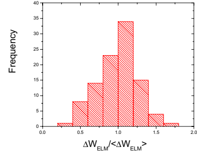
Figure 2. Histogram of the Type I ELM energy loss for a large range of plasma conditions at JET.
