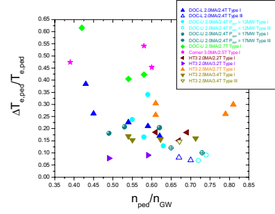
Figure 4. Normalised Type I ELM pedestal temperature drop versus pedestal density (normalised to the Greenwald limit) for the same dataset as Fig. 1.
