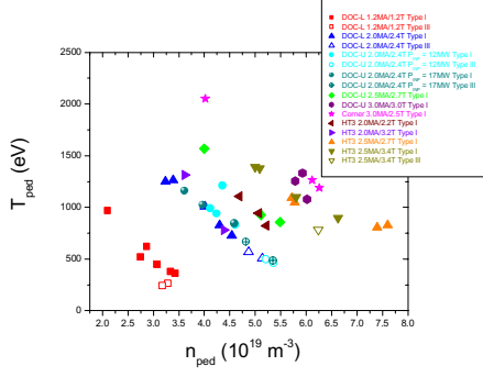
Figure 1. Pedestal plasma parameters before ELMs for the JET experiments described in this paper.
