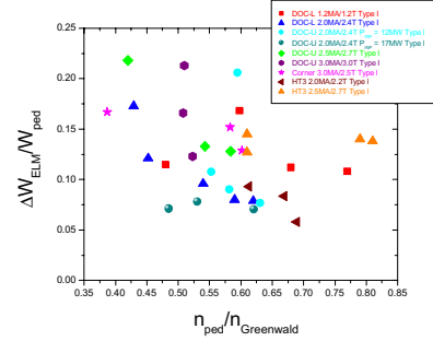
Figure 6. Normalised (to the pedestal energy) Type I ELM energy loss versus pedestal density (normalised to the Greenwald limit) for the same dataset as Fig. 1.
