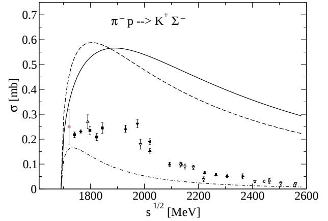
FIG. 6: Reaction \pi^-p \rightarrow K^+\Sigma^- . Theoretical curves as described in Fig. 2. Complete data reference in Ref. [1].
