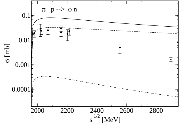
FIG. 2: Reaction \pi^- p \rightarrow \phi n . The solid line shows the result using the full, energy dependent amplitude, while the dashed-dotted line shows the pole approximation. The dashed line shows the result using the full amplitude after a readjustment of the subtraction constants, as described in Sec. III C. The complete data reference can be found in Ref. [1].
