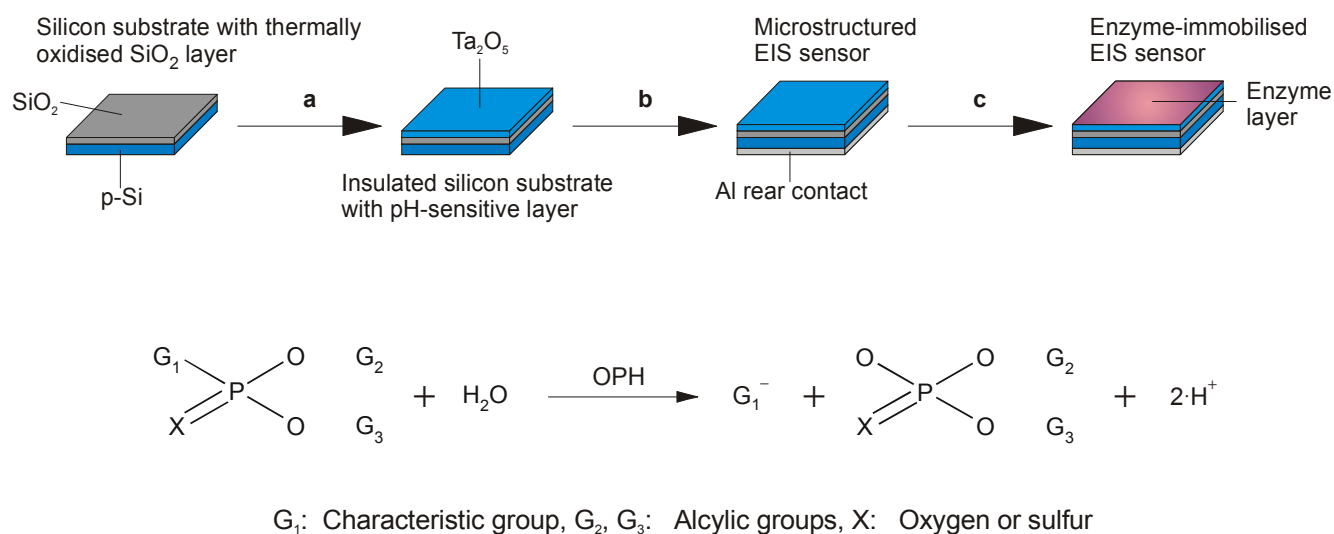
Figure 1. Schematic of fabrication steps (a-c) of the capacitive EIS biosensor (upper part), and hydrolytical reaction of the enzyme OPH releasing H^+ ions that can be detected by means of the pH-sensitive transducer surface (lower part).
