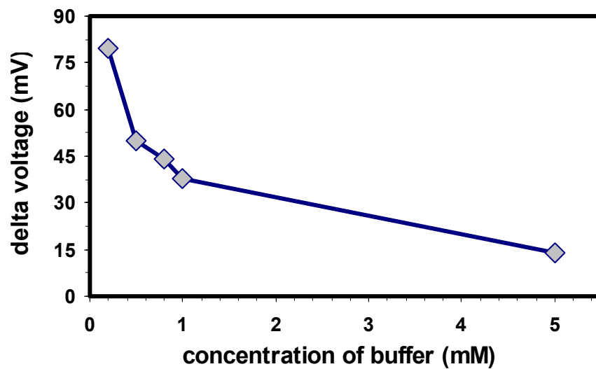
Figure 3. Effect of the HEPES buffer concentration on the response of the EIS biosensor; measuring conditions: pH 9, 50 \mu\text{M} \text{CoCl}_2 , 100 mM NaCl, 100 \mu\text{M} paraoxon.
