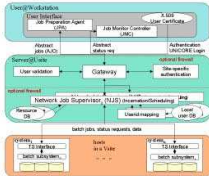
Fig. 2: Detailed Architecture
