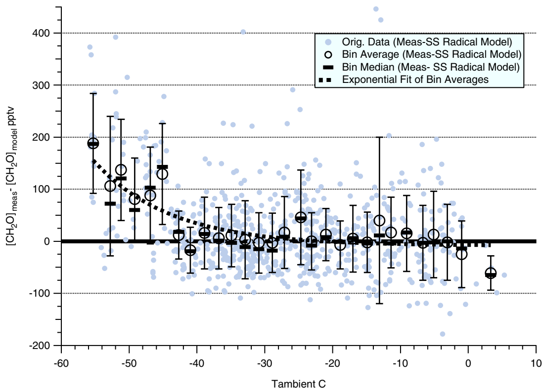
Figure 9. CH 2 O (measurement–model) differences versus ambient sampling temperature for background conditions based on the fast measurements of NO, NO x , NO y , and CNC. The comparisons for both original background data and bin averages (2°C temperature bins) are shown. The dashed line is an exponential fit of the bin averages. The number of points in each bin ranges between an average of 13 for temperatures <−45°C and 28 for warmer temperatures.
