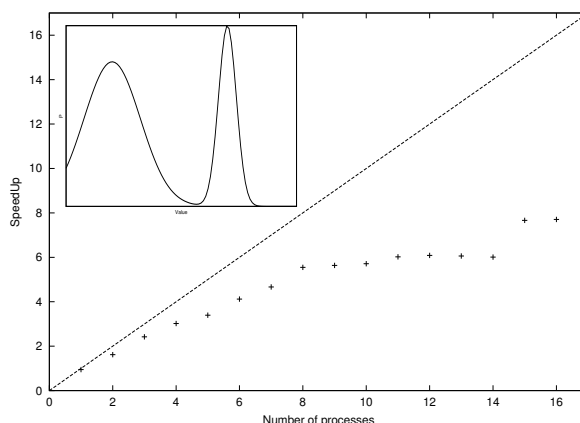
Figure 15: The speedup for the dynamic version of parallel radix sort. It is not that good in comparison to fig. 14 for the static version with a flat distribution but the static version wouldn't produce any good speedup with distributions like this one here. According to interesting cases of charge distribution in the FMM, this distribution is composed of two Gaussian distributions. Measurements are done on a CrayT3E with a maximum number of 2^{23} keys.
