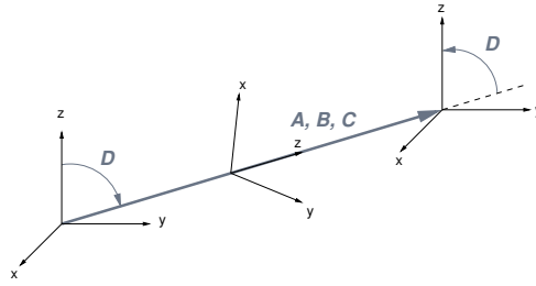
Figure 4: Rotation based FMM: To achieve scaling with O(L^3) expansions are rotated thus the translation transformation can be done along the quantization axis z .
