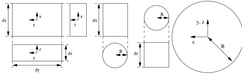
Figure 5: The already implemented containers (left) and the sphere (right) and their parameters. From the left to the right: The cuboid with the parameters dx , dy and dz . The disc with the parameter R for the radius and the length dx . The wire with the radius R and the height dz . The only parameter of the sphere is the radius R .
