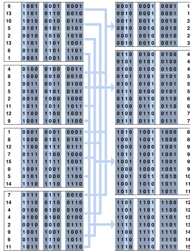
Figure 12: The static version of parallel radix sort. After the first part of presorting till there are as many classes as processes, the reassembled classes can be sorted till the end independently.
