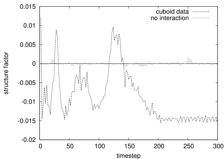
Figure 15: The time evolution of the structure factor of the small cuboid. The impulses come from a system with no interaction again.
