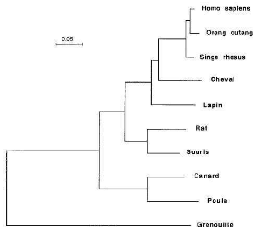
Figure 1: Evolutionary tree: the leaves represent certain species. Parental nodes represent the common ancestor. The branch length represents the time the species need to reach their evolutionary state relative to their ancestors.
