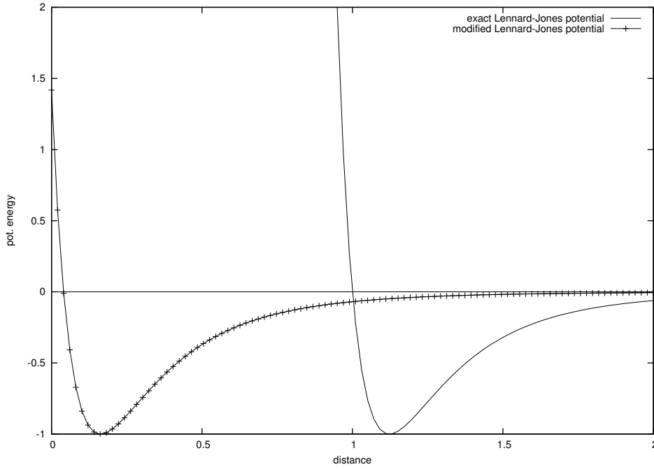
Figure 11: Comparison between the exact LENNARD-JONES potential (3) and the modified version (7) used in our simulations to find static equilibrium configurations.
