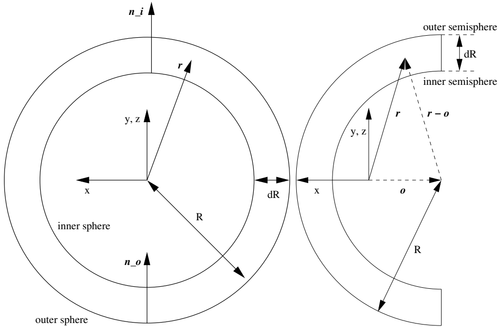
Figure 7: The hollow sphere (left) and the hollow hemisphere (right). The parameters of the hollow sphere are the radius R of the outer sphere and the shell thickness dR . Shown is an arbitrary vector \mathbf{r} which ends within the container; \mathbf{n}_o is a normal vector on the outer sphere and \mathbf{n}_i is one on the inner sphere. They fulfill the requirement of pointing towards the inside of the container. The parameters of the hollow hemisphere are the radius R of the outer sphere and the shell thickness dR . Shown is an arbitrary vector \mathbf{r} which ends within the container. For more explanations see also figure 6 (right).
