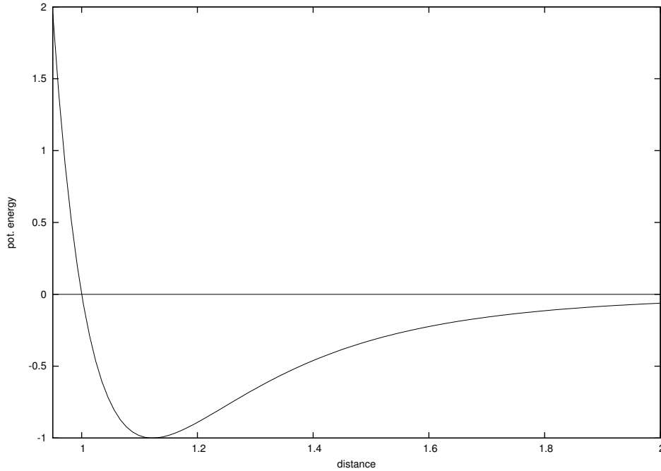
Figure 9: Qualitative form of the Lennard-Jones potential in the range 0.95 < \|\mathbf{r} - \mathbf{r}_0\| < 2 . Here is set \varepsilon = \sigma = 1 .
