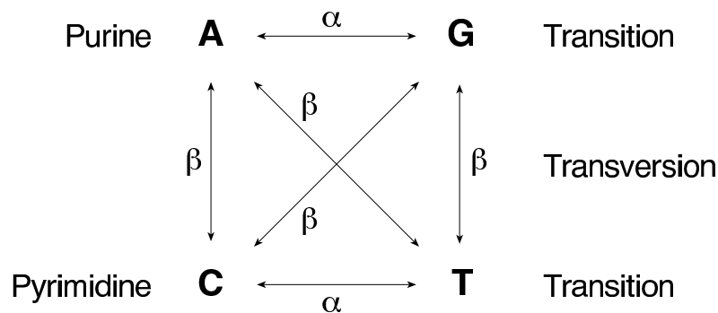
Figure 2: Substitution Model: Kimura Model: A substitution model which differentiates between the substitution rates of transitions and transversions
