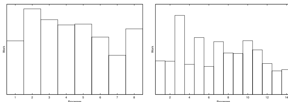
Figure 16: This shows which amount of work every single process had within the whole dynamic parallel radix sort. The load balancing works better for 8 processes than for 14 processes in this case. The 4 parameters of the dynamic radix sort have to be adjusted to avoid that one process needs a lot more time than the others. The data used here is out of the same measurements as for fig. 15.
