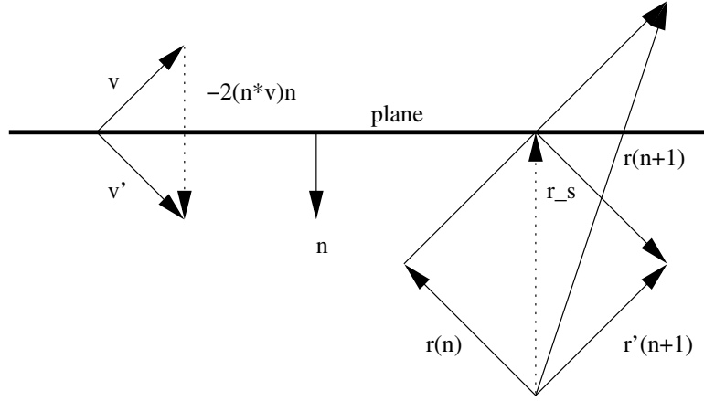
Figure 3: Reflection of a particle on a plane. The horizontal line represents the plane. The normal vector \mathbf{n} points to the inside of the container. Primed vectors label vectors after reflection. On the left hand side the reflection of the velocity \mathbf{v} is shown. Only the normal component has to be modified. On the right hand side the correction of the location \mathbf{r} at time n + 1 is shown. Here is assumed that the particle was inside the container at time n . Note that the stretch \mathbf{r}_s - \mathbf{r}(n) has to be parallel to \mathbf{v} (before reflection) and \mathbf{r}'(n + 1) - \mathbf{r}_s has to be parallel to \mathbf{v}' (after reflection).
