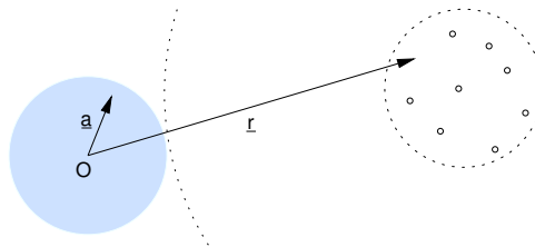
Figure 2: A Taylorlike expansion is used to express of the electrostatic potential around the origin effected by a charge pattern far away from the origin. For this again |\underline{r}| \gg |\underline{a}| must be valid.
