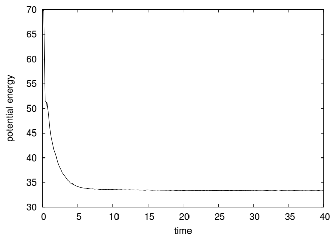
Figure 18: Time evolution of the potential energy of the system in a hollow hemisphere.
