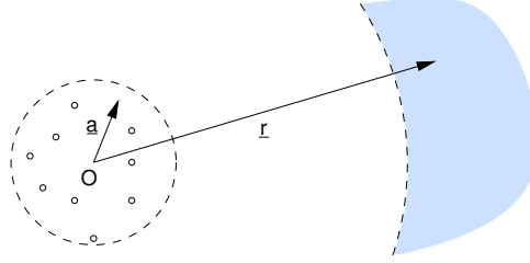
Figure 1: A multipole expansion is used to express the far field of the electrostatic potential of a charge pattern near the origin. For this |\underline{r}| \gg |\underline{a}| must be valid.
