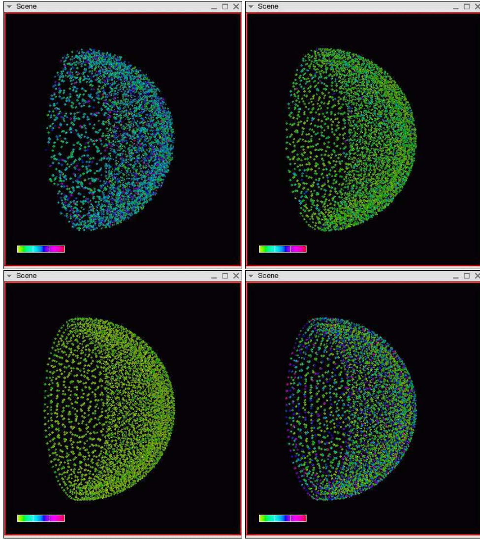
Figure 17: Time evolution of a 5000 particles system inside a hollow hemisphere. Shown are snapshots of the initial configuration (top-left), after 10 timesteps (top-right), after 50 timesteps (bottom-left) and after 200 timesteps (bottom-right).
