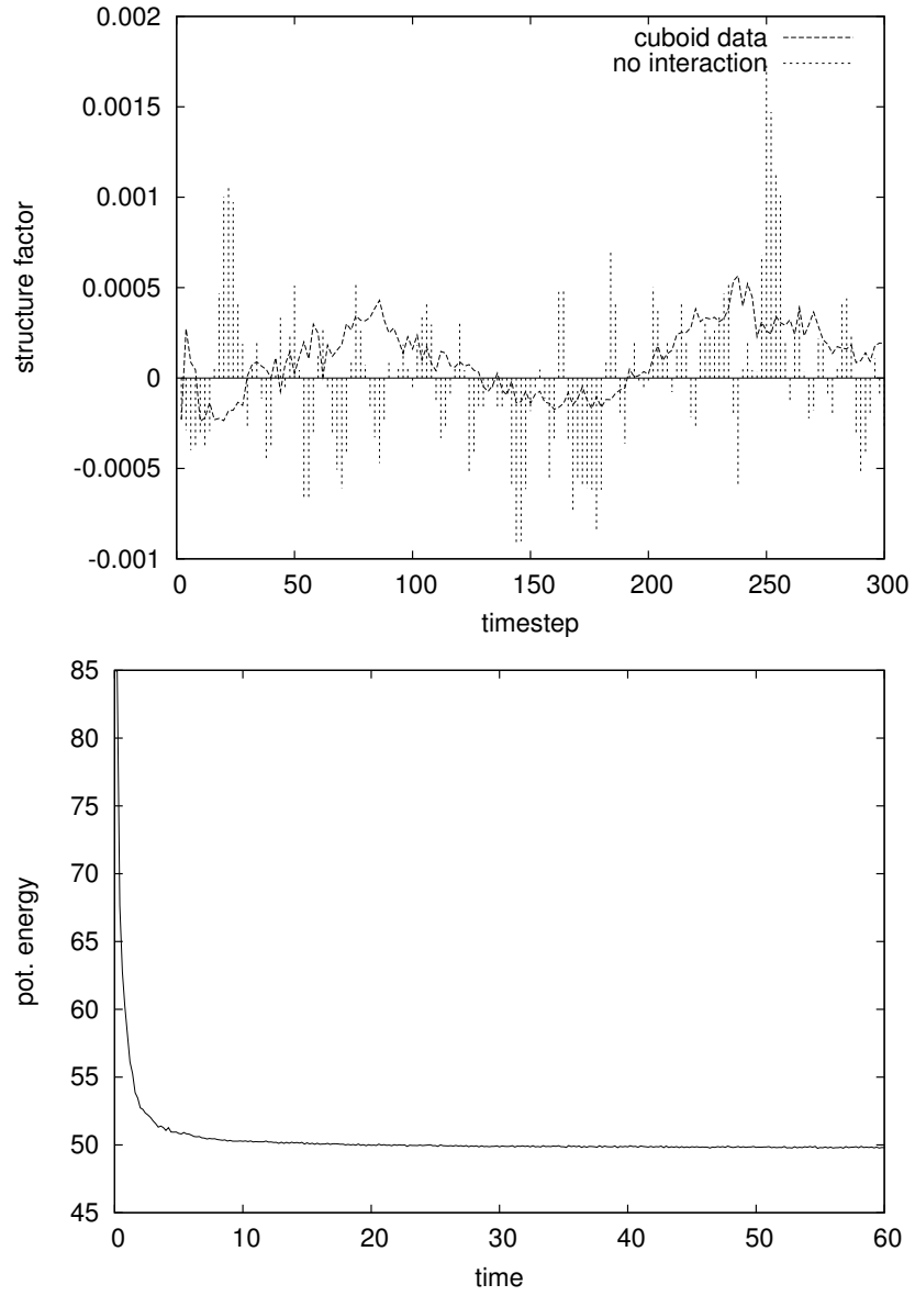
Figure 13: The time evolution of the quality of the big cuboids configuration. Shown is the structure factor (top) (the impulses come from a system with no interaction) and the potential energy (bottom).
