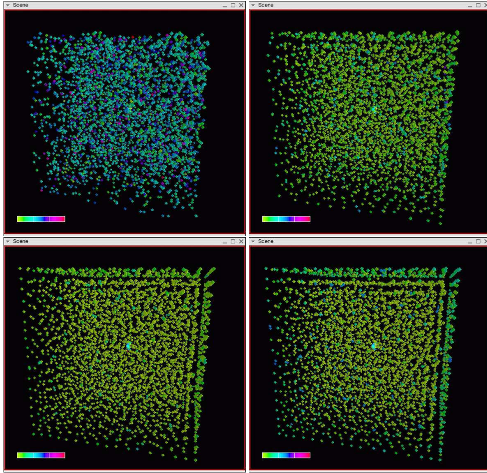
Figure 12: Time evolution of a 4096 particle system in a cuboid. Initial configuration top-left; 10 timesteps top-right; 50 timesteps bottom-left; 200 timesteps bottom-right.
