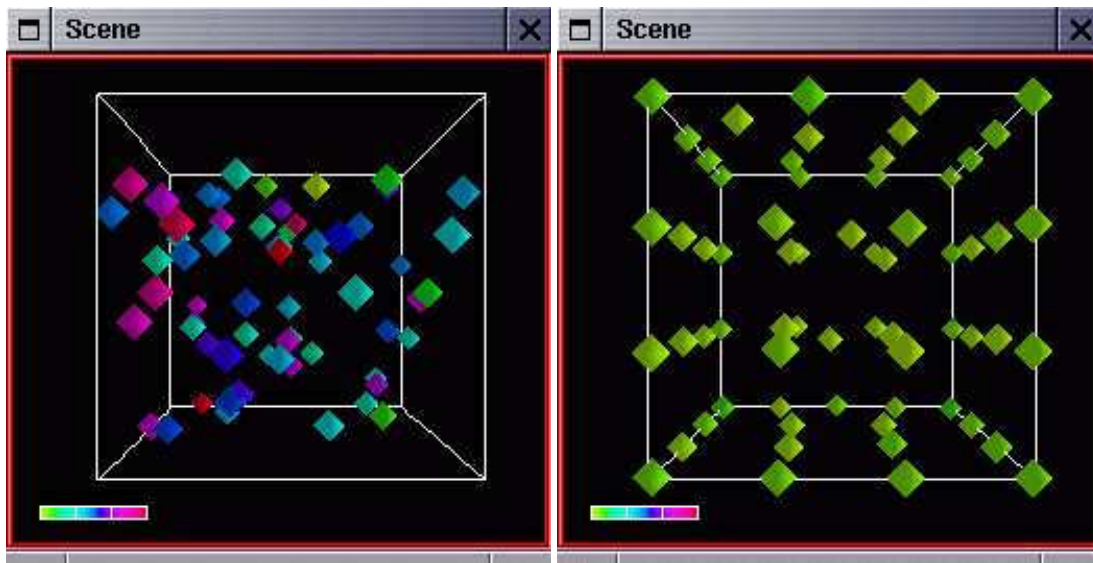
Figure 14: Time evolution of a 64 particle system constrained within a cuboid. On the left hand side is shown the initial configuration. The right hand side shows the system after 200 timesteps.
