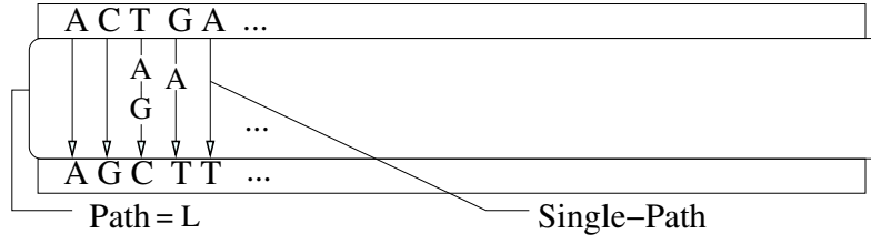
Figure 3: Path and Single-path: A path consists of all interstates a sequence x passes, when it evolves to sequence y . A single-path describes the evolution of one single nucleotide to another.
