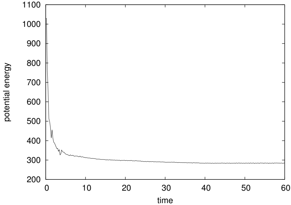
Figure 16: Time evolution of the potential energy of the small cuboid system.
