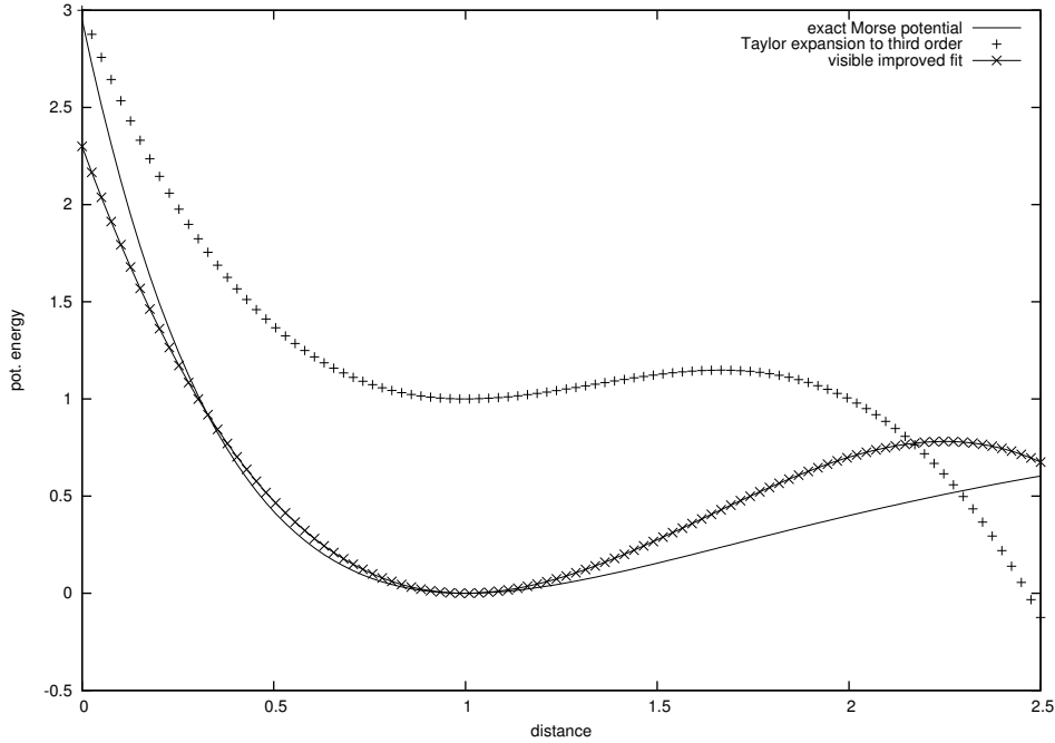
Figure 10: Comparison between the MORSE potential (4) (solid line), its TAYLOR expansion to third order (5) (points) and a visible improved fit using a series potential (6) (points on solid line). The parameters are set to D = a = r_e = 1 .
