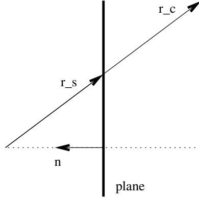
Figure 4: Cutting a root vector \mathbf{r}_c on a plane. We get the equation \frac{\|\mathbf{r}_s\|}{\|\mathbf{r}_c\|} = \frac{|\mathbf{r}_s \cdot \mathbf{n}|}{|\mathbf{r}_c \cdot \mathbf{n}|} from the intersection theorem. This means \|\mathbf{r}_s\| = \frac{|\mathbf{r}_s \cdot \mathbf{n}|}{|\mathbf{r}_c \cdot \mathbf{n}|} \|\mathbf{r}_c\| , so that \mathbf{r}_s = \frac{\|\mathbf{r}_s\|}{\|\mathbf{r}_c\|} \frac{\mathbf{r}_c}{\|\mathbf{r}_c\|} = \frac{|\mathbf{r}_s \cdot \mathbf{n}|}{|\mathbf{r}_c \cdot \mathbf{n}|} \mathbf{r}_c .
