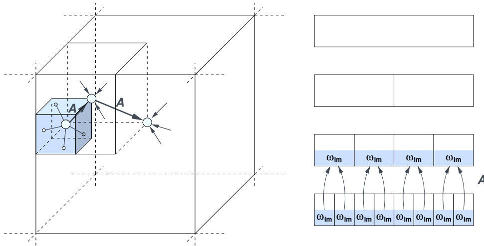
Figure 7: Pass 1 consist of calculating multipole moments in every lowest level box and translate it to the parent box from where the sum of all child expansions is translated again to its parent box in next higher level.
