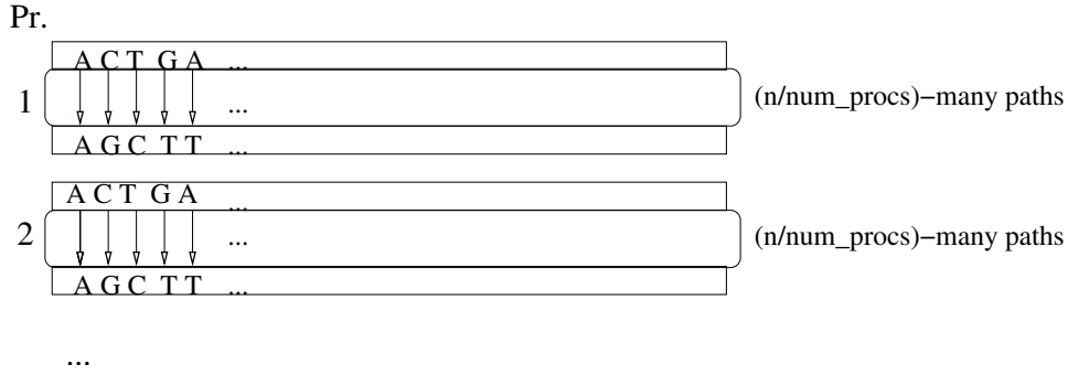
Figure 6: Parallelizing MCMC-Simulation. n = number of paths which have to be sampled; \text{num-procs} = number of processes; n/\text{num-procs} = number of paths sampled by one process
