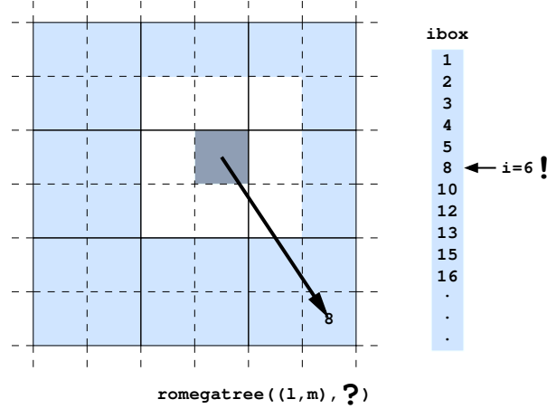
Figure 10: Pass 2 needs to know not only the names of the destination boxes for the transformation but also at which position their \omega_{lm} 's and \mu_{lm} 's in the corresponding arrays are stored.
