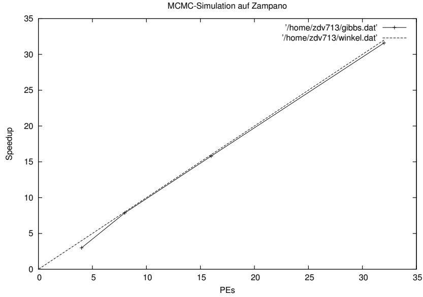
Figure 7: Speedup of the MCMC-Simulation on ZamPaNo;5000 Paths; Sequence length = 2000
