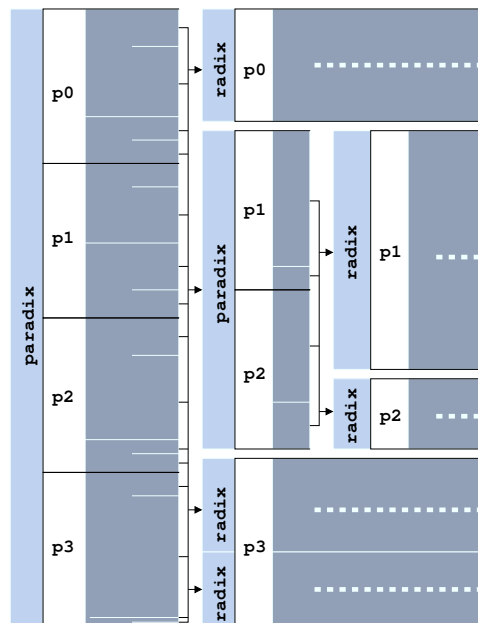
Figure 13: The dynamic version of parallel radix sort. It is the same principle as in the static version but processes can work together on one large class (p1 and p2) by calling paradox again together on the large class or a process can work on more than one smaller classes. It is a more abstract representation but both cases of class distributing can be seen. The lighter grey areas represent the data in the Global Array, the darker areas data in the local buffer.
