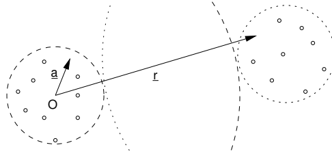
Figure 3: The Coulomb energy of two charge patterns satisfying the conditions of multipole or Taylorlike expansions respectively, can be written in terms of multipole moments and Taylorlike coefficients.
