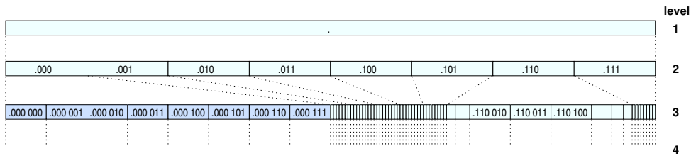
Figure 6: Boxes are enumerated by an integer consisting of tripels of bits. Every tripel contains the information about the box location in a special level. Doing enumeration this way it is always possible to know parent box or all child boxes by shifting the bits 3 positions right or left respectively.
