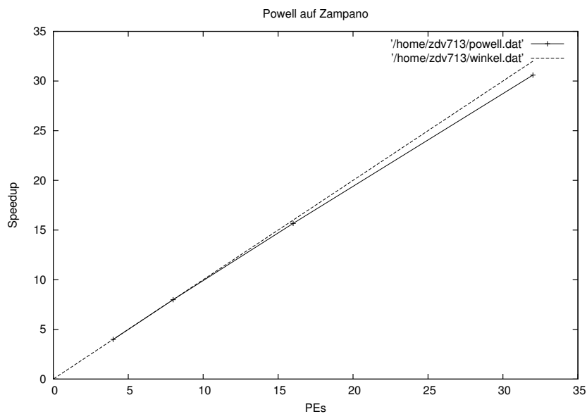
Figure 8: Speedup of the Powell-function on ZamPaNo;5000 Paths; Sequence length = 2000
