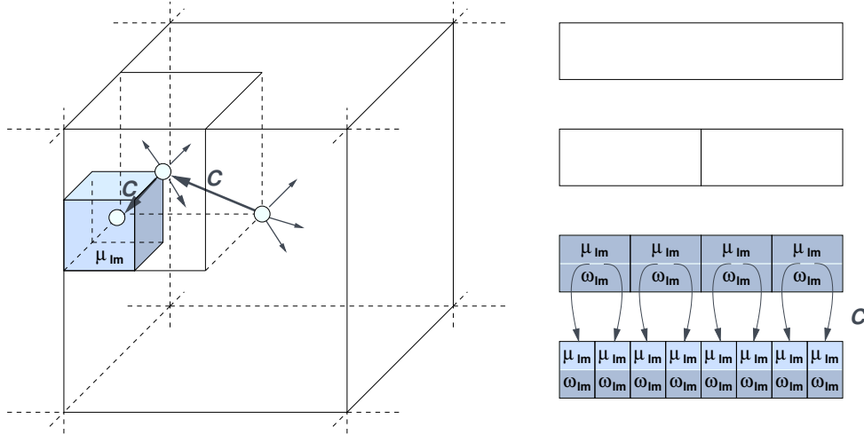
Figure 9: As the counterpart to pass 1 in pass 3 the Taylor expansions in parent boxes are translated to Taylor expansions in all child boxes.
