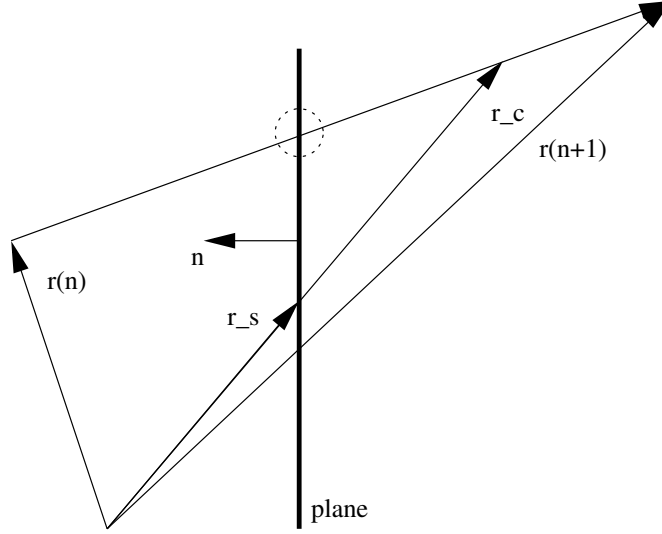
Figure 1: Construction of the position vector \mathbf{r}_s of the tangent plane. Consider a course of one particle. At time n it is inside of the container and at time n + 1 it is outside of the container (the normal vector \mathbf{n} points towards the inside of the container). After a bisection algorithm along the vector \mathbf{r}(n + 1) - \mathbf{r}(n) we end at the vector \mathbf{r}_c . Its length gets corrected to \mathbf{r}_s so that it ends within the surface of the container. Without numerical deviations coming from the bisection algorithm, \mathbf{r}_s (and \mathbf{r}_c ) should end at the centre of the drawn circle.
