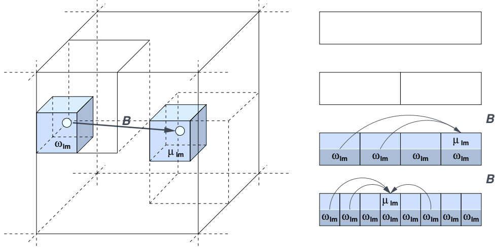
Figure 8: In pass 2 the multipole expansion of every box in every level up to the level where there are still boxes 'well separated' is transformed into local expansions of boxes belonging to a special set of destination boxes. So the information about the own charge pattern is spread.
