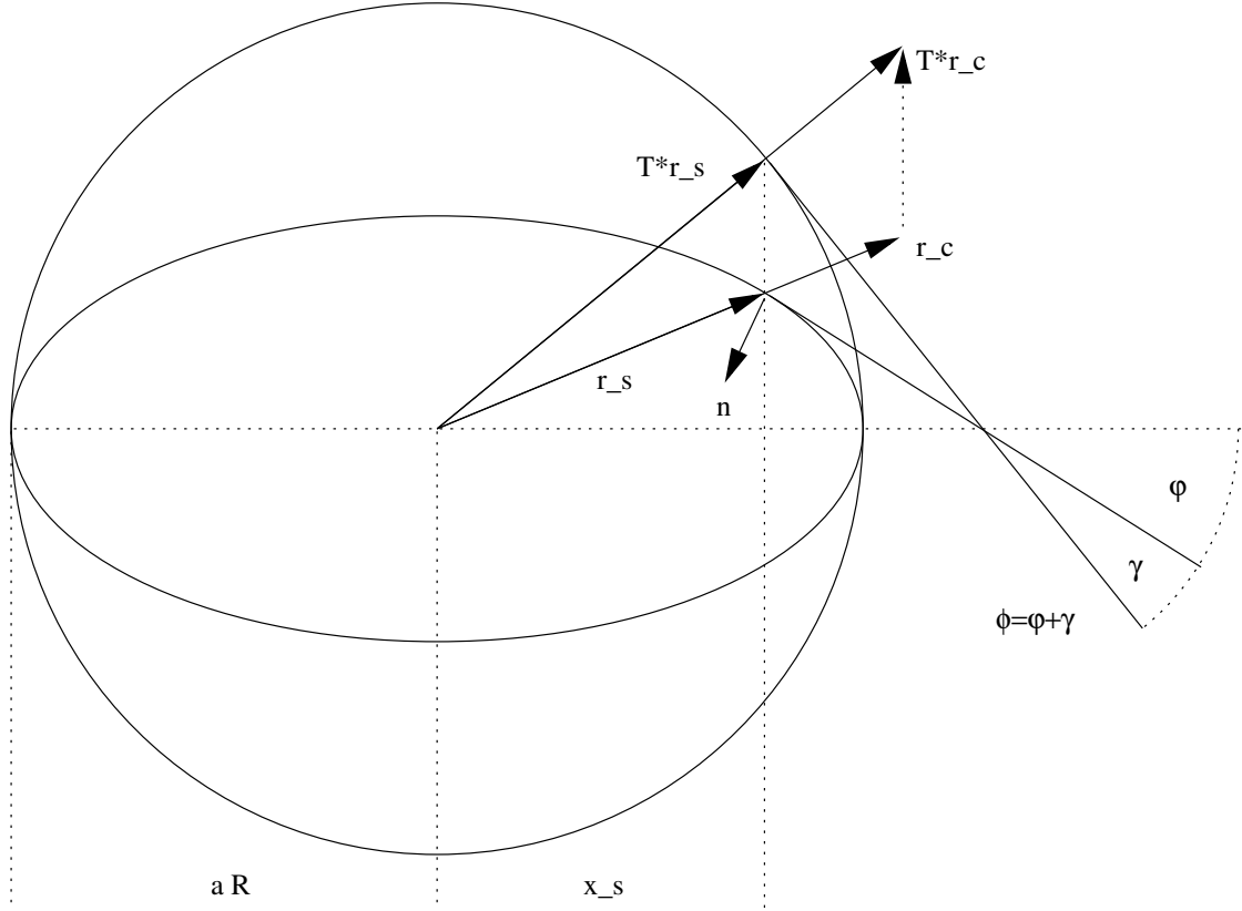
Figure 2: Construction of a normal vector \mathbf{n} on a given point \mathbf{r}_s which is ending within the surface of an ellipsoid. The first step is to transform the ellipsoid with the help of T to a ball so that \mathbf{r}_c becomes to T \cdot \mathbf{r}_c . The next step is to cut this vector down to T \cdot \mathbf{r}_s . This vector has the length Ra . Back transformation with T^{-1} leads to the position vector \mathbf{r}_s . \gamma is the angle between the tangent plane on the ball in T \cdot \mathbf{r}_s and this on the ellipsoid in \mathbf{r}_s . It is needed to calculate the normal vector \mathbf{n} .
