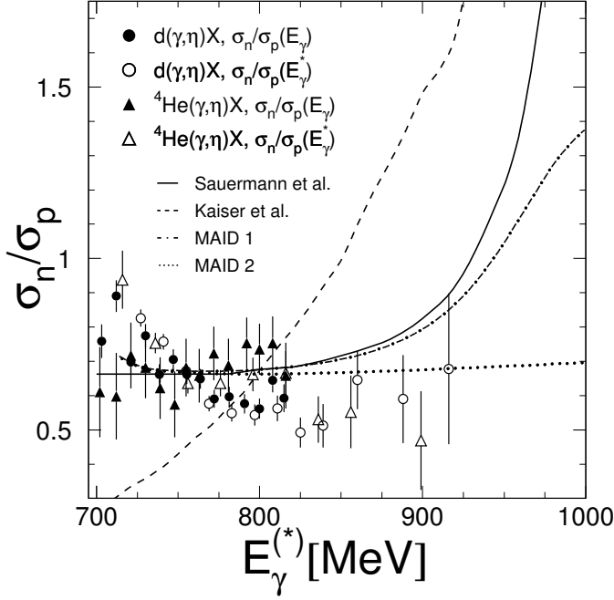
Fig. 9. Ratio of exclusive proton and neutron cross sections in the TAPS acceptance. The deuteron data are compared to the ^4\text{He} -data [17] and to model predictions from Sauermann et al. [29] and Kaiser et al. [3]. The curves labeled MAID [30] are the predictions from the full MAID model (MAID1) and a truncated version restricted to the S_{11}(1535) -resonance, Born terms and vector meson exchange (MAID2).
