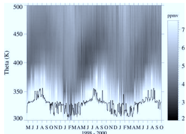
Figure 9. POAM Northern Hemisphere (55°–71°) water vapor measurements as a function of potential temperature. The data are averaged as in Figure 8. See color version of this figure at back of this issue.
