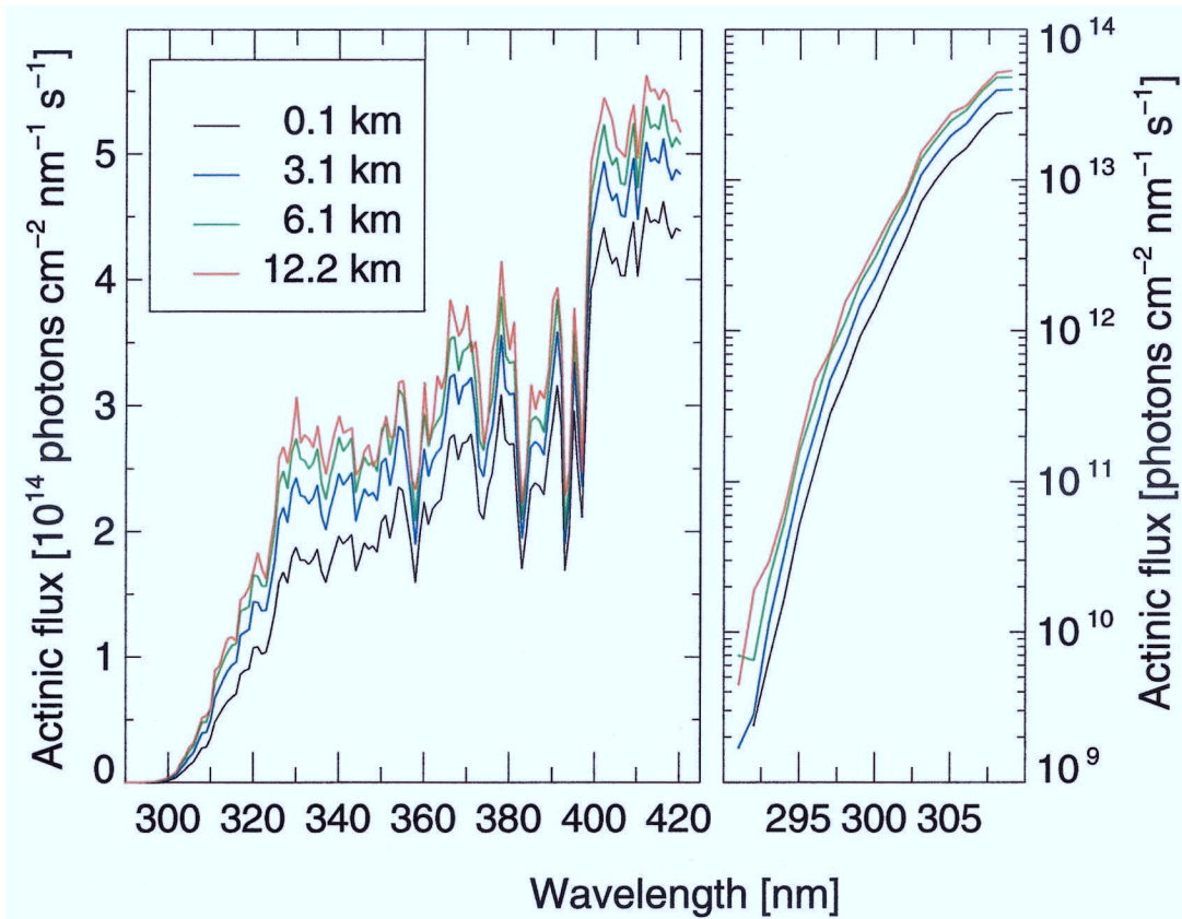
Figure 4. Spectra of the total actinic flux measured at different altitudes and cloud-free conditions over the Aegean Sea on 10 June 1996. The solar zenith angle changed from 17^\circ to 23^\circ from the lowest to the highest flight level. Note the different scaling of the actinic flux in the left (linear) and right (logarithmic) panel.
