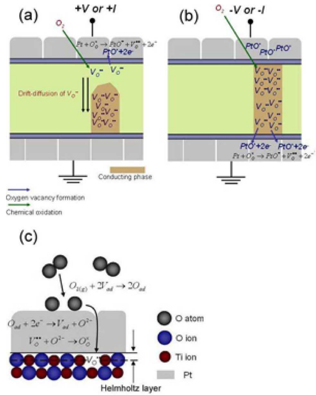
FIG. 11. (Color online) Schematic sketches of the mechanism for electroforming in air. The configuration of a conducting phase resulting from (a) the first electroforming process by applying a positive voltage/current and (b) the second electroforming by applying a negative voltage/current. TiO 2 between the conducting phases, shown in (a), is estimated to include more oxygen vacancies than stoichiometric TiO 2 . PtO* denotes a chemisorbed oxygen at a Pt grain boundary. (c) The detail of the chemical reaction at the TE illustrated in (a) and (b).
