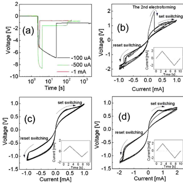
FIG. 8. (Color online) (a) Electroforming performed in vacuum by applying three different negative constant currents, -100\ \mu\text{A} , -500\ \mu\text{A} , and -1\ \text{mA} . The current applications started at 2 s. Under a current of -100\ \mu\text{A} the resistance underwent a single abrupt drop at 26 s. No additional decrease in the resistance occurred under the given current. Under a current of -500\ \mu\text{A} , the resistance underwent two abrupt decreases, the first decrease at 4 s and the second one at 110 s. Afterward, no additional electroforming steps were necessary for the activation of the bipolar switching. A V - I curve under a current of -1\ \text{mA} showed one sudden decrease in the voltage at 2.8 s. The resistance after the single decrease in the resistance was comparable to that after the two drops of the voltage in the resistance under a current of -500\ \mu\text{A} and no additional degradations (electroforming) were necessary for the bipolar switching observation. (b) Bipolar switching curves of the cell electroformed with -100\ \mu\text{A} . The second electroforming occurred during the increase in the current on the positive side. Eventually, the bipolar switching could be measured. Bipolar switching curves of the cell electroformed with (c) -500\ \mu\text{A} , and (d) -1\ \text{mA} .
