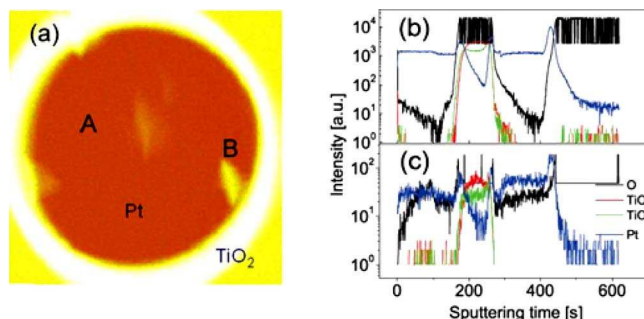
FIG. 9. (Color online) (a) Oxygen signal over the whole 100 \times 100\ \mu\text{m}^2 area, where the circle is the circular-shaped top electrode ( 100\ \mu\text{m} diameter). (b) Depth profile at the point A in the dark area. (c) Depth profile at the bright point indicated by B.
