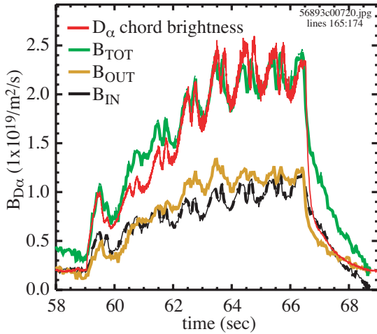
Figure 1: D_\alpha chordal brightness (dah) used to calibrate the simulated camera D_\alpha chord, B_{TOT} . Also shown are the contributions from the inner ( B_{IN} ) and outer edges ( B_{OUT} ) of the plasma.
