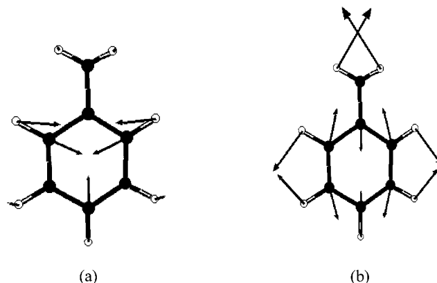
Figure 11. Calculated eigenvectors of the ring-breathing mode (a) and a characteristic ring vibration at 1608 \text{ cm}^{-1} (b) of aniline.
