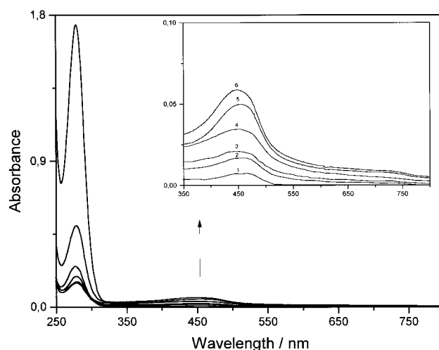
Figure 1. UV-VIS absorption spectra of the supernatants of centrifuged suspensions of Cu(II)-montmorillonite ( 13\ \text{g dm}^{-3} , pH = 6.0) in the presence of increasing concentrations of aniline: (1) 4; (2) 5.3; (3) 6.6; (4) 13; (5) 26; (6) 40\ \text{mmol/dm}^3 .
