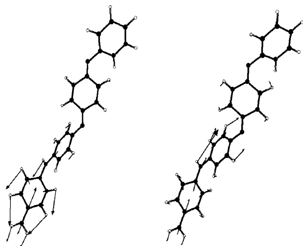
Figure 13. Calculated eigenvectors of the characteristic C–N vibrations at 1246 \text{ cm}^{-1} and 1259 \text{ cm}^{-1} in the \text{NH}-(\text{C}_6\text{H}_4)-\text{NH} unit of EB.
