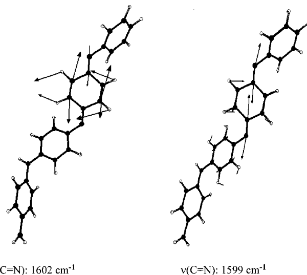
Figure 12. Calculated eigenvectors of the characteristic C=N vibrations of the double bond at 1602 and 1599 \text{ cm}^{-1} in the -\text{N}=(\text{C}_6\text{H}_4)=\text{N}- unit of EB.
