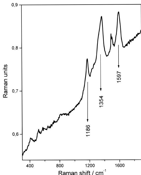
Figure 10. NIR-FT Raman spectrum of aniline ( 2.0 \text{ mmol g}^{-1} ) adsorbed on Cu(II) montmorillonite in the 400\text{--}1700 \text{ cm}^{-1} region: laser power, 250 \text{ mW} ; number of scans, 100.
