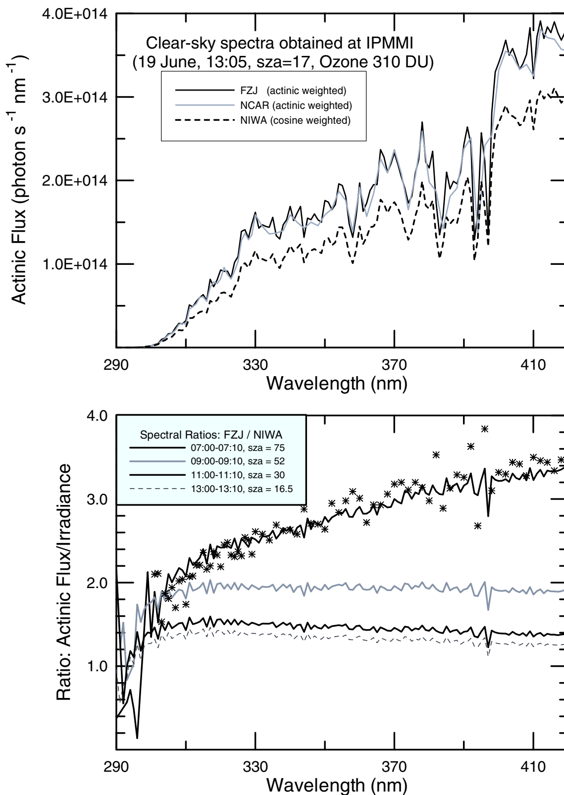
Figure 1. (top) Spectra measured by each instrument near solar noon (SZA = 17°, 13:05 MDT) on 19 June 1998. In this plot the y axis is plotted on a linear scale, and the sampling interval for the x axis is 1 nm, except at \lambda > 300 nm, where the National Center for Atmospheric Research (NCAR) sampling interval was 2 nm. (bottom) Spectral ratios of actinic flux divided by irradiances (Forschungszentrum Jülich/National Institute of Water and Atmosphere (FZJ/NIWA)) for several solar zenith angles (SZA). The asterisks on the upper curve show the ratios for NCAR/NIWA.
