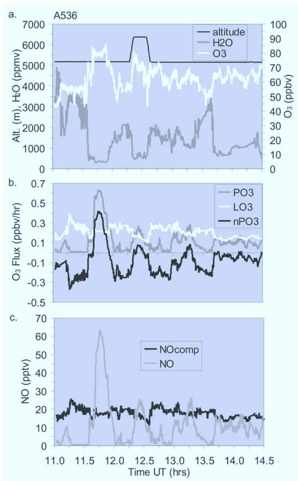
Figure 12. Time series for cases 10a, 10b, and 10c (flight A536 on 10 April 1997): (a) observed H 2 O (gray line) and O 3 (white line) concentrations and altitude (black line), (b) calculated values of L O3 (white line), P O3 (gray line), and nP O3 (black line), and (c) observed concentrations of NO (gray line) and calculated values of NO comp (black line).
