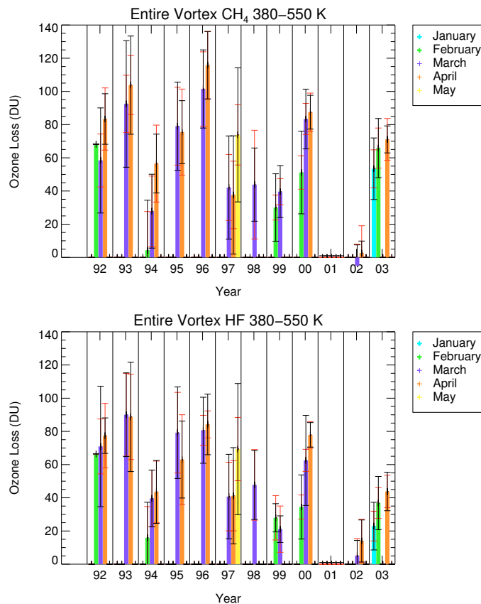
Fig. 9. Monthly averaged column ozone loss derived for profiles inside the entire vortex in 380–550 K, February (green), March (purple), April (orange) and May (yellow) in winters between 1991–1992 and 2002–2003. The red error bar indicates the uncertainty of the early winter reference function, the black error bar the standard deviation. Top panel: CH 4 was used as the long-lived tracer, bottom panel: HF was used as the long-lived tracer. Ozone loss was derived from profiles inside the entire vortex.
