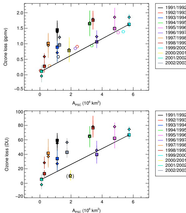
Fig. 13. Top panel: relation between the accumulated ozone loss in mixing ratio and A_{PSC} in the Arctic polar vortex for the years 1991–1992 to 2002–2003 in different colours. Monthly averaged ozone loss inside the vortex core in March (February in 2000–2001 and 2002–2003) between 400–500 K (between 450–500 K inside the entire vortex in winter 2000–2001), using the TRAC method, coloured solid squares (HF is used as the long-lived tracer) and solid diamonds ( \text{CH}_4 is used as the long-lived tracer). A_{PSC} was averaged between January to March of each year and between 400–500 K derived from UKMO data. Ozone loss derived with the average approach (Rex et al., 2002) is shown in coloured open circles and A_{PSC} using ECMWF data. Black line indicates a linear relation between A_{PSC} and ozone loss. Bottom panel: as top panel, but for the column ozone loss (DU) in the altitude range 400–500 K derived only from HALOE observations is apparent.
