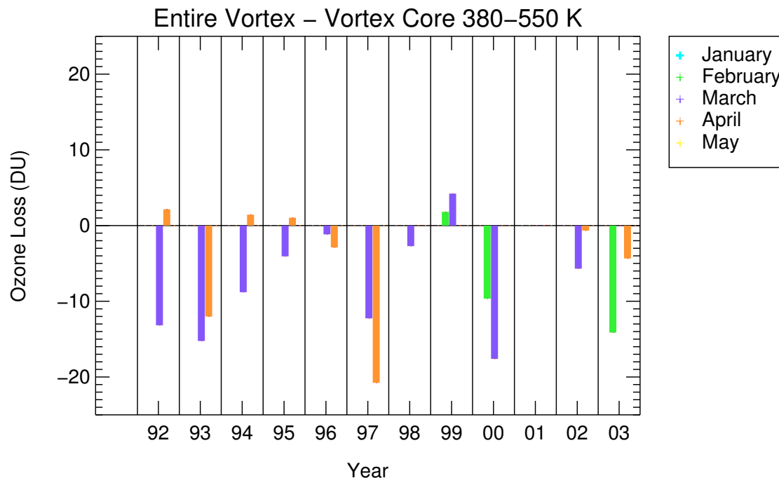
Fig. 11. Difference of monthly averaged column ozone loss between the entire vortex and the vortex core for all winters between 1991–1992 and 2002–2003, using both \text{CH}_4 and HF as the long-lived tracers. Results were derived in an altitude range of 380–550 K.
