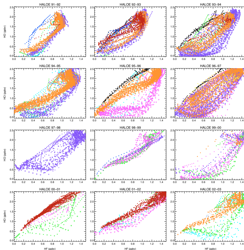
Fig. 4. HCl/HF relations for the twelve winters between 1991–1992 and 2002–2003 as measured from profiles inside the vortex core (diamonds), inside the outer vortex (large plus signs), inside an outer part of the outer vortex (small crosses) by HALOE are shown. Different colours of profiles indicate the different time intervals when profiles were observed: November (black), December (blue), January (cyan), February (green), first part of March (magenta), second part of March (purple), first part of April (orange), second part of April (dark red).
