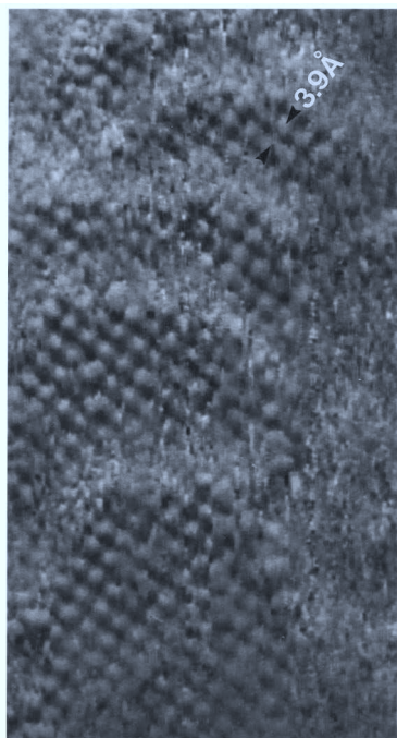
FIG. 8. STM image of a growth spiral taken on top of a ridge of the canyonlike structure of Fig. 6.
