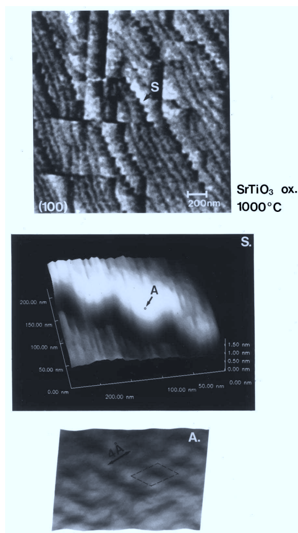
FIG. 4. Detailed pseudo-three-dimensional presentation of a (100) surface oxidized at 1000 °C [compare the upper picture also with Fig. 3(a)]. The topography has a pronounced zigzag-type structure [see details of segment S in the middle picture, (b)] and is governed by a step height of 11.8 Å. This is related to the lattice constant in the c direction of a Ruddlesden-Popper phase ( Sr_2TiO_4 ) which is perpendicular to the surface. Enlargement (segment A indicated in the middle figure) reveals the perovskite unit cell ( a = b = 3.9 Å) with atomic resolution [lower picture, (c)].
