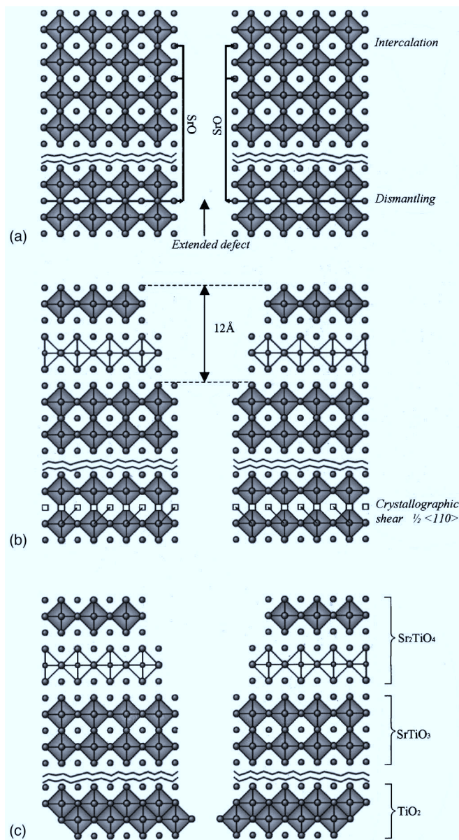
FIG. 11. Schematic illustration of the possible restructuring of the near-surface region of \text{SrTiO}_3 at elevated temperatures for oxidizing conditions. The figure depicts in a simplified manner the interplay of basic processes, such as dismantling, transport, and intercalation of \text{SrO} layers (a) as well as corresponding shearing mechanisms [see (b)], which result in the chemical modification of the near-surface region (c) with the formation of Ruddlesden-Popper phases (here only \text{Sr}_2\text{TiO}_4 ) and \text{Ti} -rich phase (here only \text{TiO}_2 ). The presented scheme combines information from a range of available experimental data, mainly by x-ray diffraction (Refs. 17 and 42), microanalysis (Ref. 17), high-resolution transmission electron microscopy (Refs. 50 and 79) and atomic force microscopy (this work). But note, the illustration does not reflect the full complexity of the processes (see text). For reducing conditions basically the same kind of basic processes are involved in the restructuring of the near-surface region taking into account, in particular, the continuous loss of oxygen from the surface.
