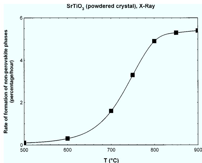
FIG. 9. Rate of formation of nonperovskite phases in SrTiO 3 for oxidizing conditions at different temperatures (adapted in parts from Ref. 42).
