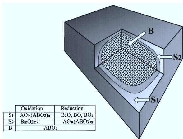
FIG. 10. Schematic illustration of the chemical heterogeneity in the surface region of a \text{SrTiO}_3 crystal induced by oxidation or reduction at elevated temperatures.
