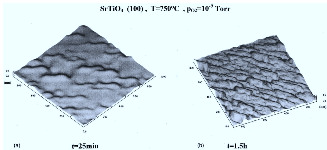
FIG. 7. AFM images taken in situ of a (100) surface after slow cooling of samples heated in reducing conditions to 750 °C for 25 min (a) and then reheated for 1.5 h (b).
