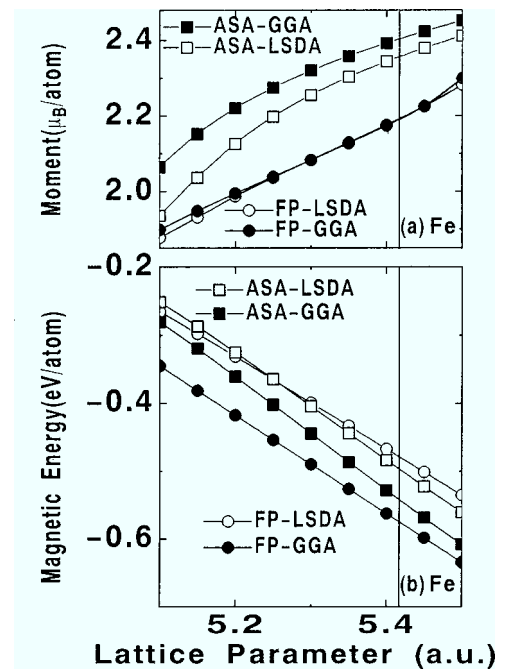
FIG. 3. Lattice parameter dependence of magnetic moment (a) and magnetic energy (b) for Fe.
