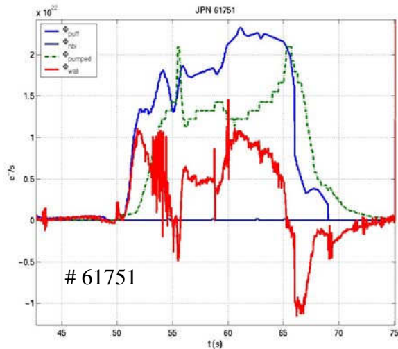
Figure 5: Time evolution of particle fluxes \Gamma_{puff} , \Gamma_{exhausted} , and resulting wall particle retention \Gamma_{wall} .
