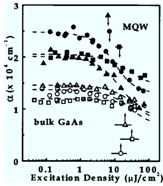
FIG. 3. Excitation density dependence of the apparent optical absorption coefficient \alpha in Be-doped ( 7.8 \times 10^{17} \text{ cm}^{-3} ) bulk GaAs (open symbols) and GaAs/AlAs MQWs (closed symbols) grown at 600 ( \Delta ), 360 ( \circ ), and 310 ( \square ) °C. Dashed curves are fits to the data. Arrows show the saturation density F_{\text{sat}} for each sample, and error ranges are indicated by bars.
