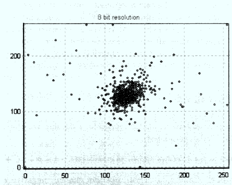
Figure 1: Typical scatter plot of the first two MAD components for bitemporal LANDSAT imagery.
