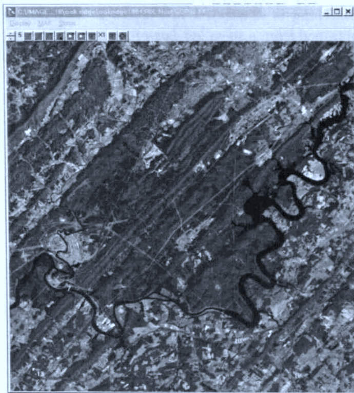
Figure 4: Matched ground control points.
