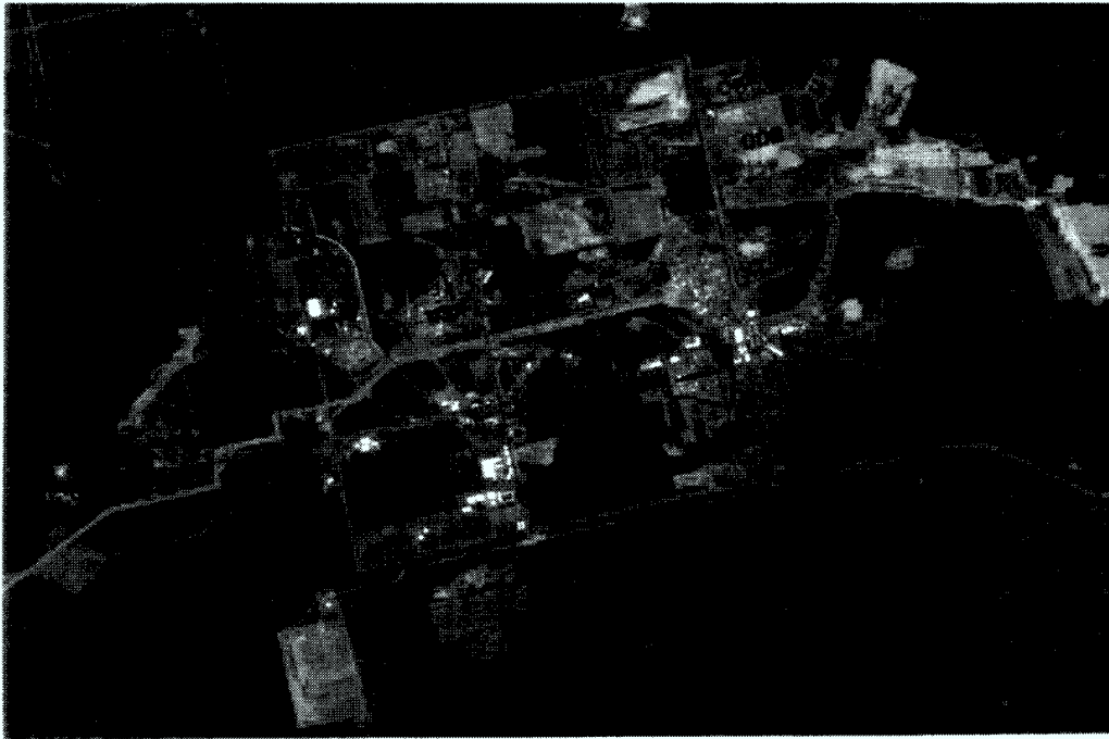
Figure 23: Close up of a service area at Hanford. MAD components as in Fig. 15, registered and fused to the IRS-1C panchromatic image from 7.7.1987 having a spatial resolution of 5m.
