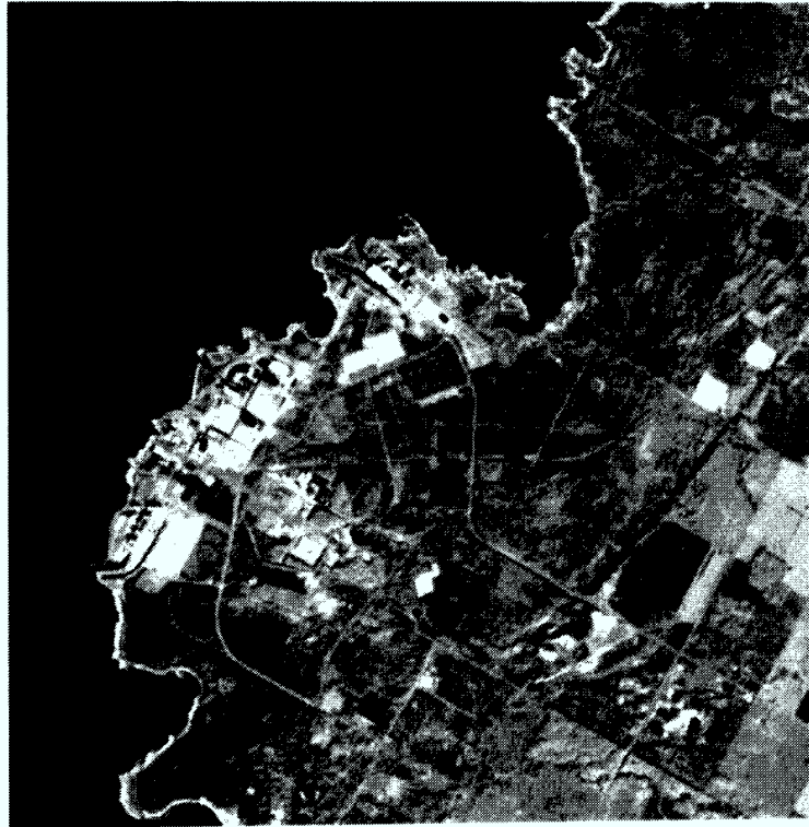
Figure 18: MAD change detection for BMS4 (August 1996 – September 1999). The first component exceeding 1.5 standard deviations is shown green. It is fused via the IHS (intensity-hue-saturation) transformation to the 15m resolution panchromatic channel of the 1999 image.
