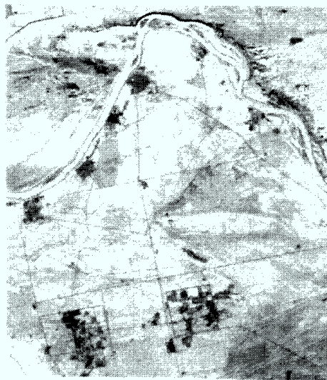
Figure 22: MAD change detection for LANDSAT images of Hanford from 12.8.1983 and 28.6.1987. Components 1 and 2 are shown in red and green, respectively. The thresholds are set at approximately 2 standard deviations. The background image is band 5 of the 1987 scene.
