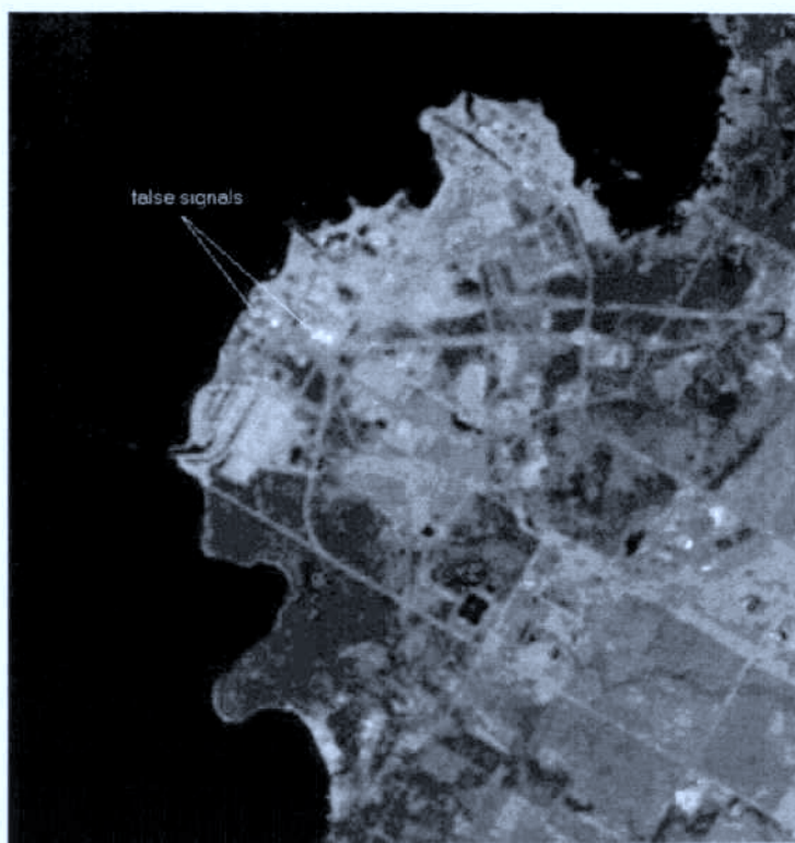
Figure 16: MAD change detection for BMS2 (August 1996 – May 1997). The first two MAD components exceeding approximately 2.2 standard deviations are in red and green. They are fused via the IHS (intensity-hue-saturation) transformation to channel 5 of the May 1997 image for better reference.
