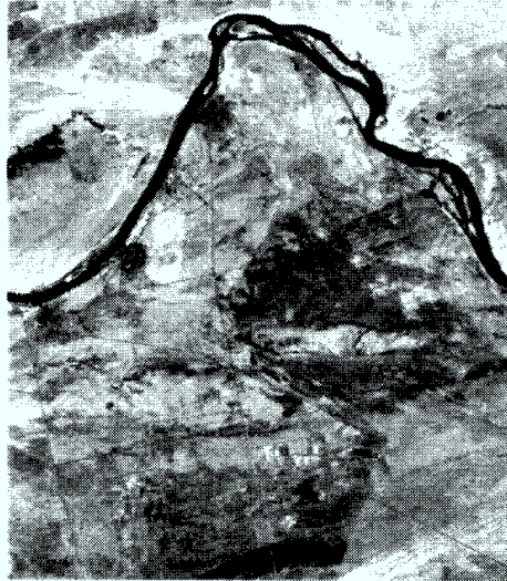
Figure 21: False color composite of the LANDSAT image of the Hanford site from 28.6.1987, bands 3 (blue), 4 (green) and 5 (red).
