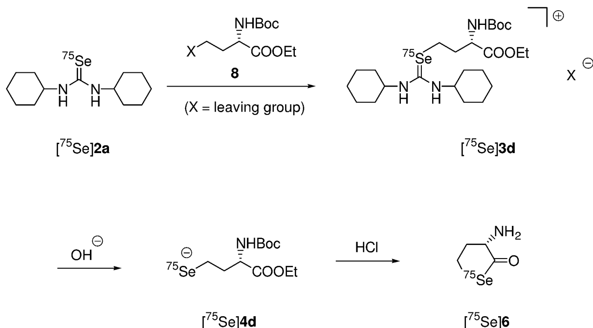
Sch. 3.13: Homocysteine [^{75}\text{Se}] selenolactone ( [^{75}\text{Se}]\mathbf{6} ) via the corresponding [^{75}\text{Se}] selenouronium salt ( [^{75}\text{Se}]\mathbf{3d} )
