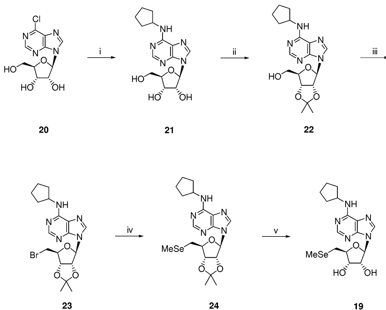
Sch. 3.20: Synthesis of 5'-(methylseleno)-CPA ( 19 )
