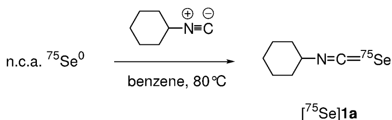
Sch. 3.3: Synthesis of cyclohexyl iso[ 75 Se]selenocyanate ([ 75 Se] 1a )
