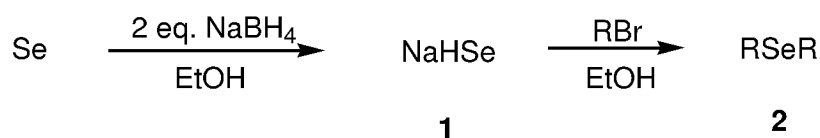
Sch. 1.2: Preparation of symmetric selenoethers ( 2 )
