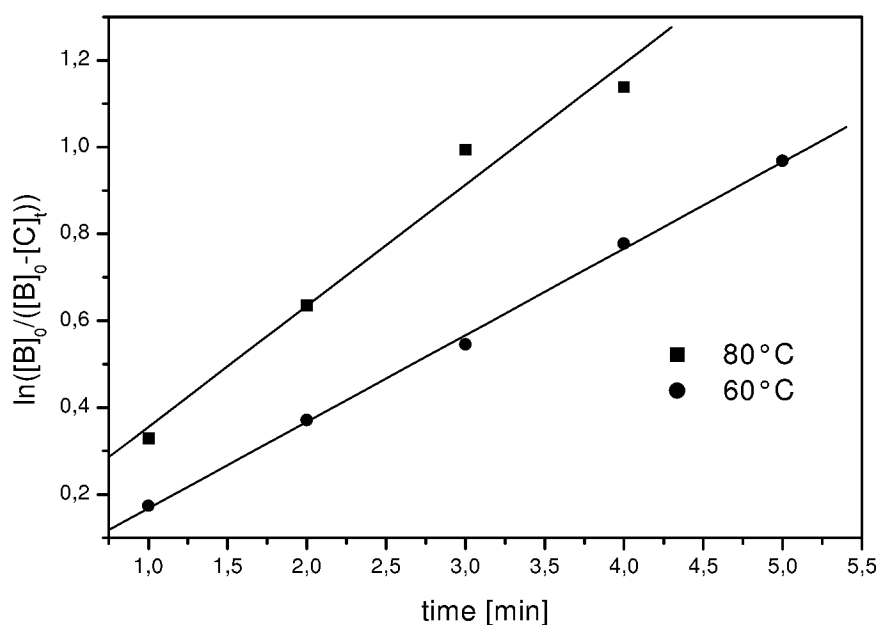
Fig. 3.11: Plot of \ln([B]_0/([B]_0 - [C]_t)) as a function of time for the determination of the relative rate constants k for the synthesis of [^{75}\text{Se}]\mathbf{10a} at 80 °C and 60 °C
