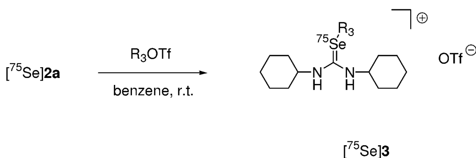
Sch. 3.6: Synthesis of [ 75 Se]selenouronium salts ([ 75 Se] 3 ) (R 3 = methyl ([ 75 Se] 3a ), ethyl ([ 75 Se] 3b ) and propyl ([ 75 Se] 3c ))
