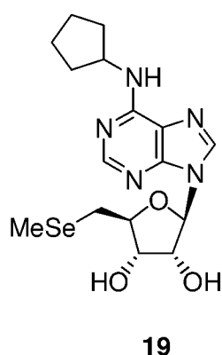
Sch. 3.19: 5'-(Methylseleno)-N 6 -cyclopentyladenosine ( 19 )
