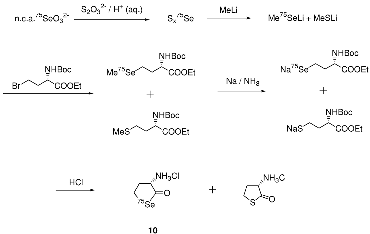
Sch. 1.12: Radiosynthesis of n.c.a. L-homocysteine [ ^{75}\text{Se} ]selenolactone hydrochloride ( 10 ) with sulfur as non-isotopic carrier
