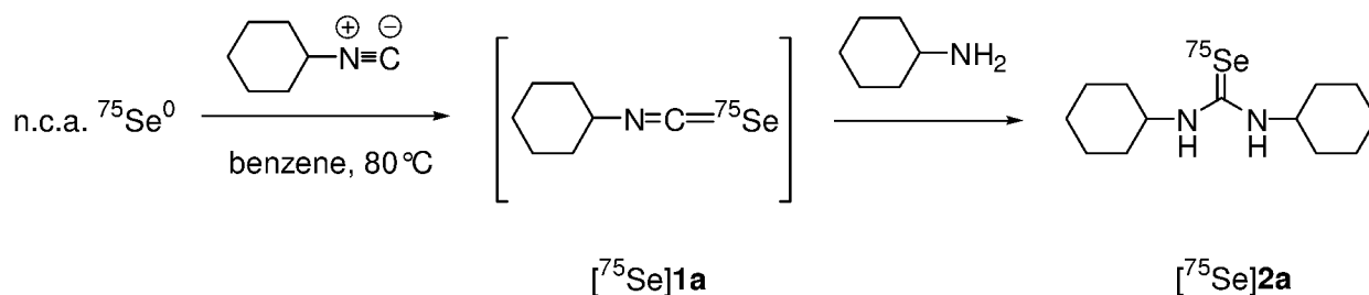
Sch. 3.4: One-pot synthesis of 1,3-dicyclohexyl [ ^{75}\text{Se} ]selenourea ( [^{75}\text{Se}]\mathbf{2a} )
