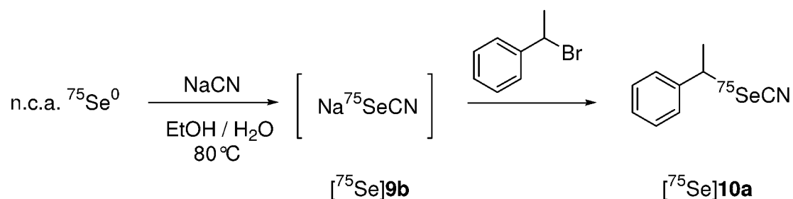
Sch. 3.15: Synthesis of 1-phenylethyl-1- ^{75}\text{Se} selenocyanate ( ^{75}\text{Se} 10a )
