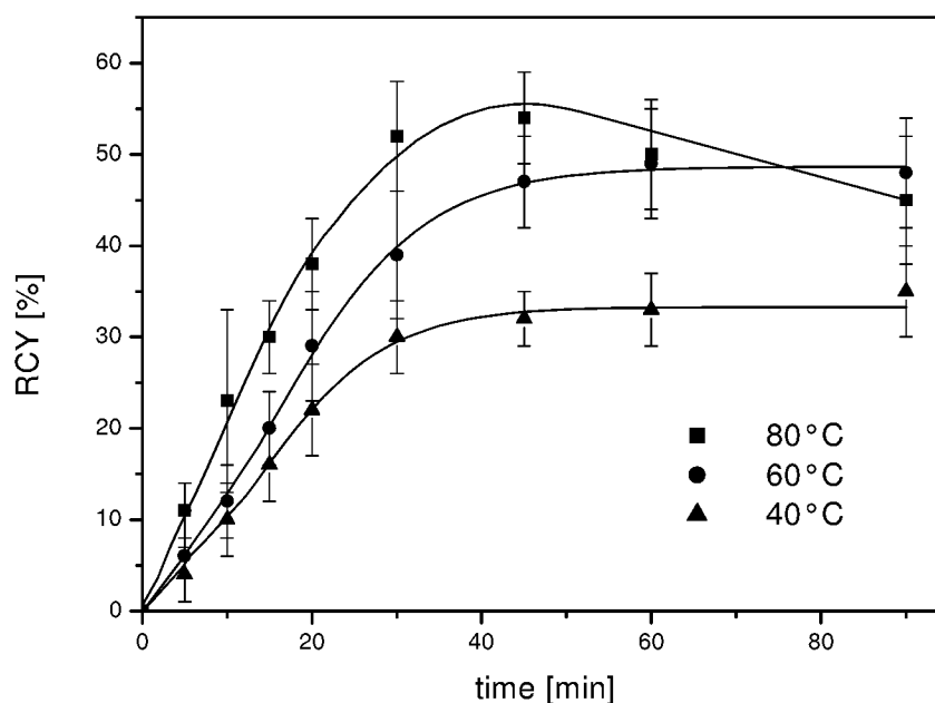
Fig. 3.2: Radiochemical yield of cyclohexyl iso[ ^{75}\text{Se} ]selenocyanate ([ ^{75}\text{Se} ]1a) as a function of time and temperature
