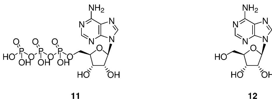
Sch. 1.14: ATP (11) and adenosine (12)
