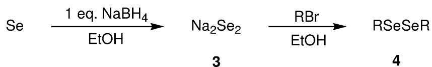
Sch. 1.3: Preparation of diselenides ( 4 )
