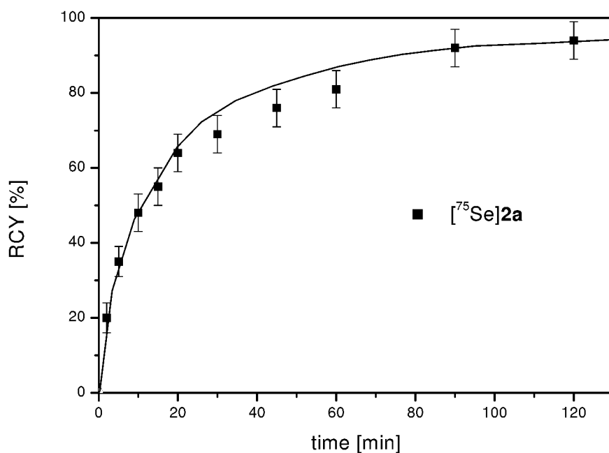
Fig. 3.3: Radiochemical yield of 1,3-dicyclohexyl [ ^{75}\text{Se} ]selenourea ( [^{75}\text{Se}]\mathbf{2a} ) as a function of time
