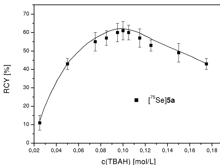
Fig. 3.7: Radiochemical yield of benzylmethyl[ ^{75}\text{Se} ]selenide ([ ^{75}\text{Se} ] 5a ) as a function of concentration of TBAH
