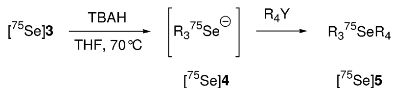
Sch. 3.8: Synthesis of asymmetric [ 75 Se]selenoethers ([ 75 Se]5) via one-pot procedure starting from [ 75 Se]3
