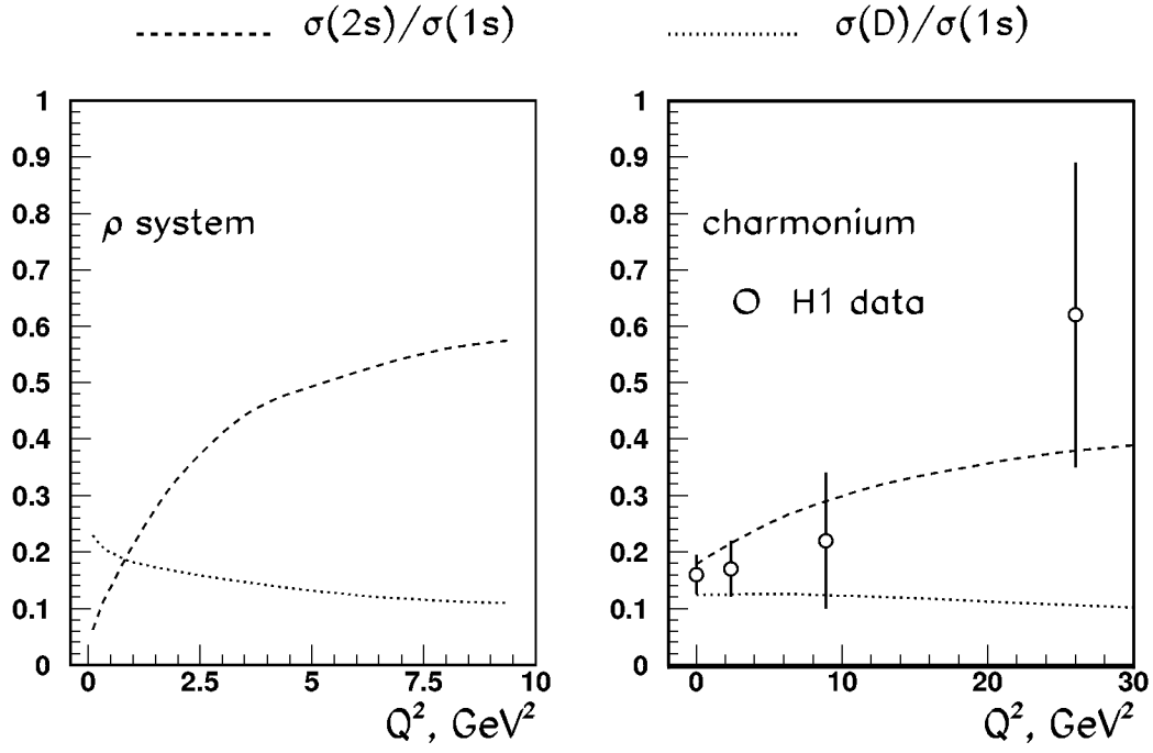
Figure 10.26: The Q^2 behavior of the ratio of excited to ground state vector meson production cross sections for \rho and charmonium systems. Dashed and dotted lines represent \sigma(2S)/\sigma(1S) and \sigma(D)/\sigma(1S) ratios, respectively. In all calculations, the oscillator wave function was used.
