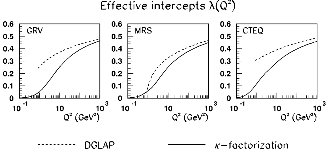
Figure 8.11: Comparison of the intercept \lambda_{eff}^{(pt)}(Q^2) of the x -dependence of the GRV98L0, CTEQ4L(v.4.6) and MRS-LQ-1998 gluon structure functions G_{pt}(x, Q^2) with their counterpart \lambda_{eff}(Q^2) for integrated G_D(x, Q^2) evaluated with D-GRV, D-CTEQ and D-MRS parameterizations for differential gluon structure function \mathcal{F}(x, Q^2) .
