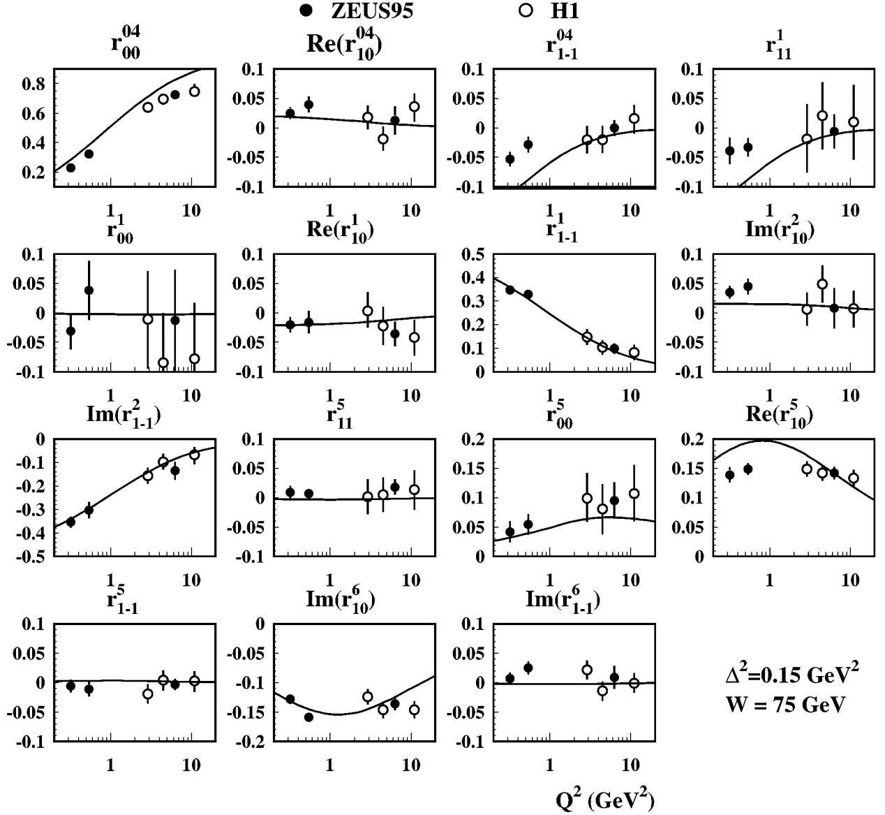
Figure 10.17: Experimental data on spin density matrix for \rho meson production as function of Q^2 compared with k_t -factorization predictions based on the oscillator wave function.
