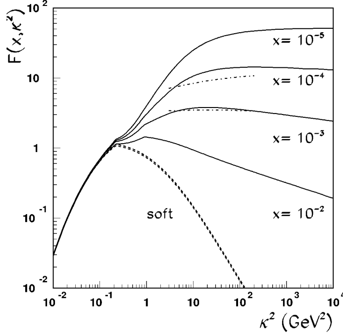
Figure 8.2: The same as in Fig. 8.1 but overlaid onto one graph for illustration of the x -dependence of \mathcal{F}(x, \vec{\kappa}^2) . The dashed lines shows the soft component \mathcal{F}_{soft}(x, \vec{\kappa}^2) and its slight variation with x due to the finite- x factor (1-x)^5 . The dot-dashed curves show the Kwiecinski et al. [68] results for DGSF from a \vec{\kappa} -factorization phenomenology of F_{2p}(x, Q^2) based on the solution of the unified BFKL/DGLAP equation.
