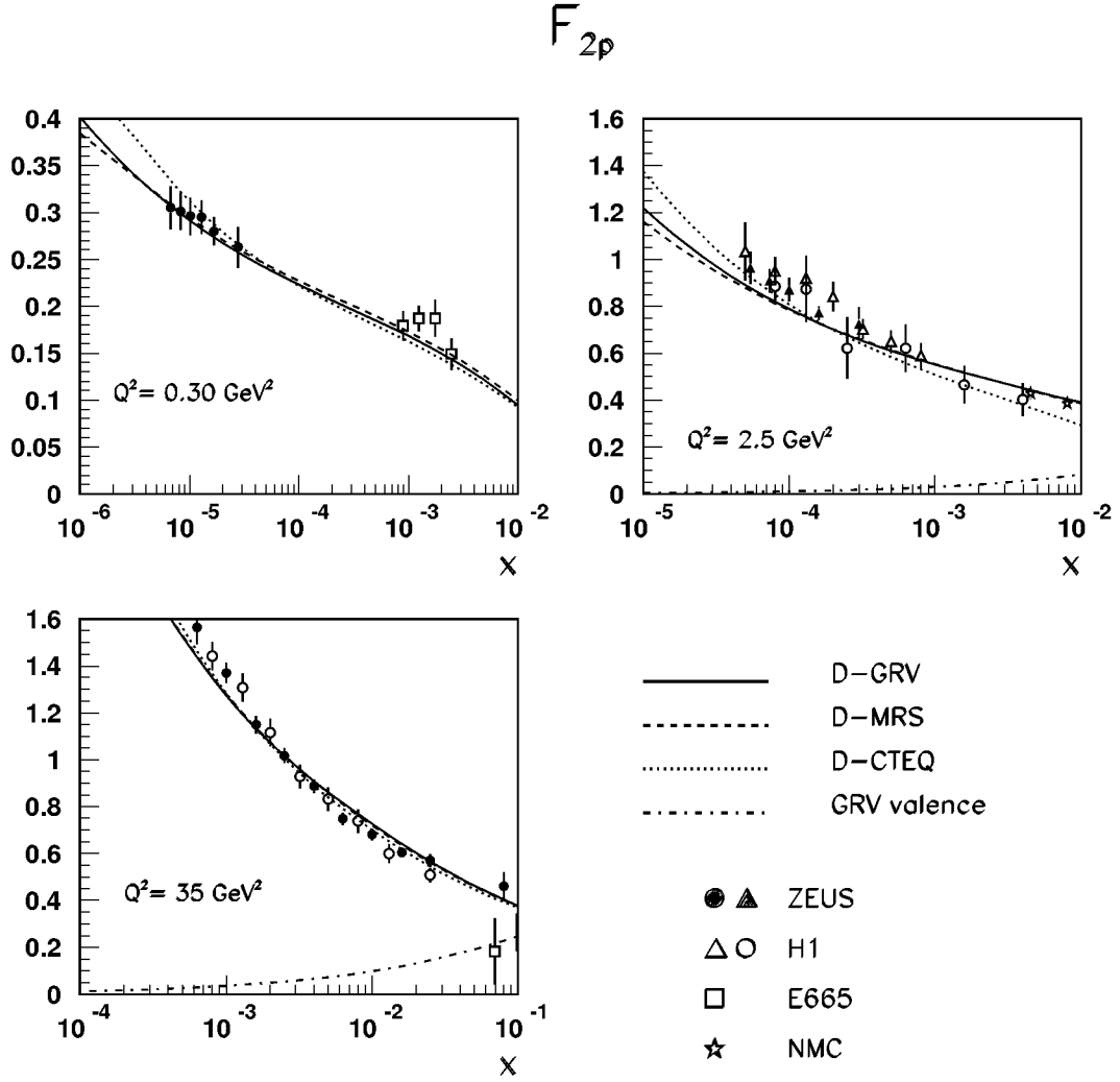
Figure 7.3: A comparison of the \vec{k} -factorization description of the experimental data on F_{2p}(x, Q^2) for several values of Q^2 with the D-GRV, D-CTEQ and D-MRS parameterizations of the differential gluon structure function \mathcal{F}(x, \vec{k}^2) . The contribution to F_{2p}(x, Q^2) from DIS off valence quarks is shown separately for larger Q^2 .
