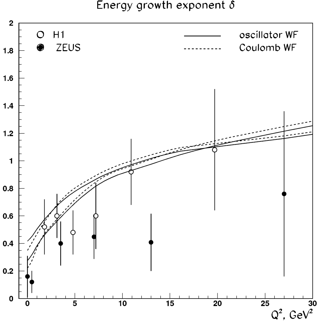
Figure 10.11: Effective exponents \delta of energy growth for the \rho meson production cross sections. Solid and dashed lines correspond to oscillator and suppressed Coulomb wave functions, respectively. The upper pair of curves (at low Q^2 ) corresponds to \delta calculated between 50 and 75 GeV, while the lower pair is the result for \delta calculated between 110 and 150 GeV.
