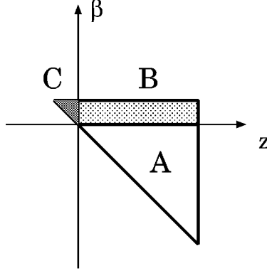
Figure A.2: The three subregions of (z, \beta) plane that contribute to the overall integral.
