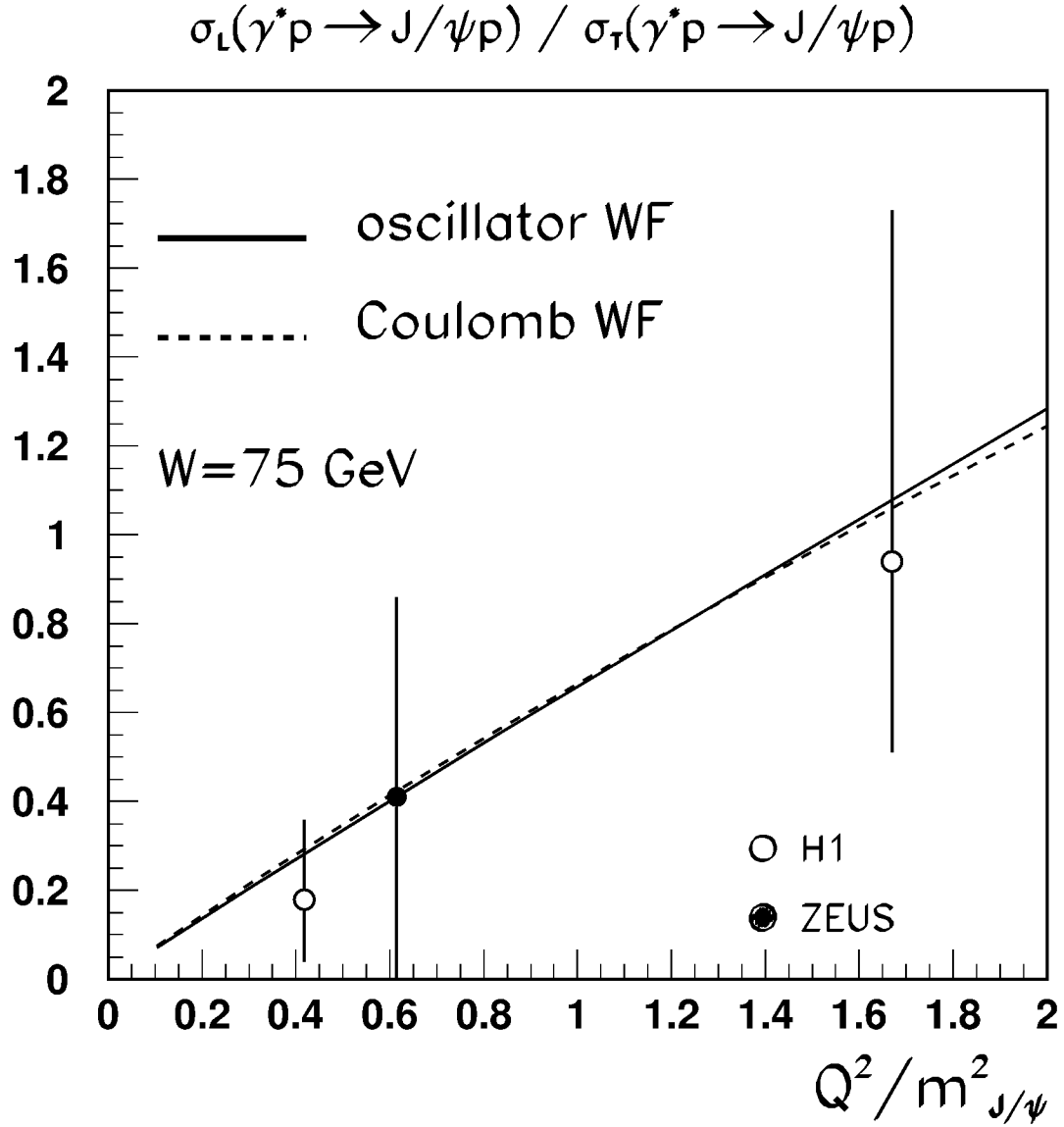
Figure 10.24: The ratio R = \sigma_L / \sigma_T as a function of Q^2 for J/\psi meson production as a function of Q^2 . Solid and dashed lines correspond to oscillator and suppressed Coulomb wave functions, respectively.
