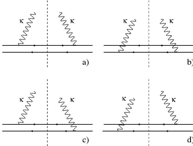
Figure 2.4: The Fermi-Weizsäcker-Williams diagrams for calculation of the flux of equivalent photons in positronium.
