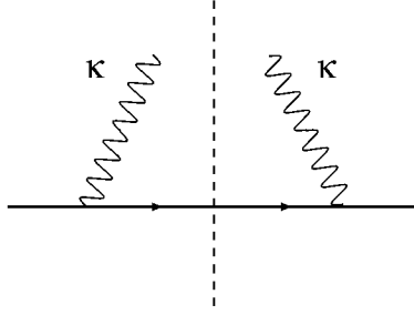
Figure 2.3: The Fermi-Weizsäcker-Williams diagram for calculation of the flux of equivalent photons
