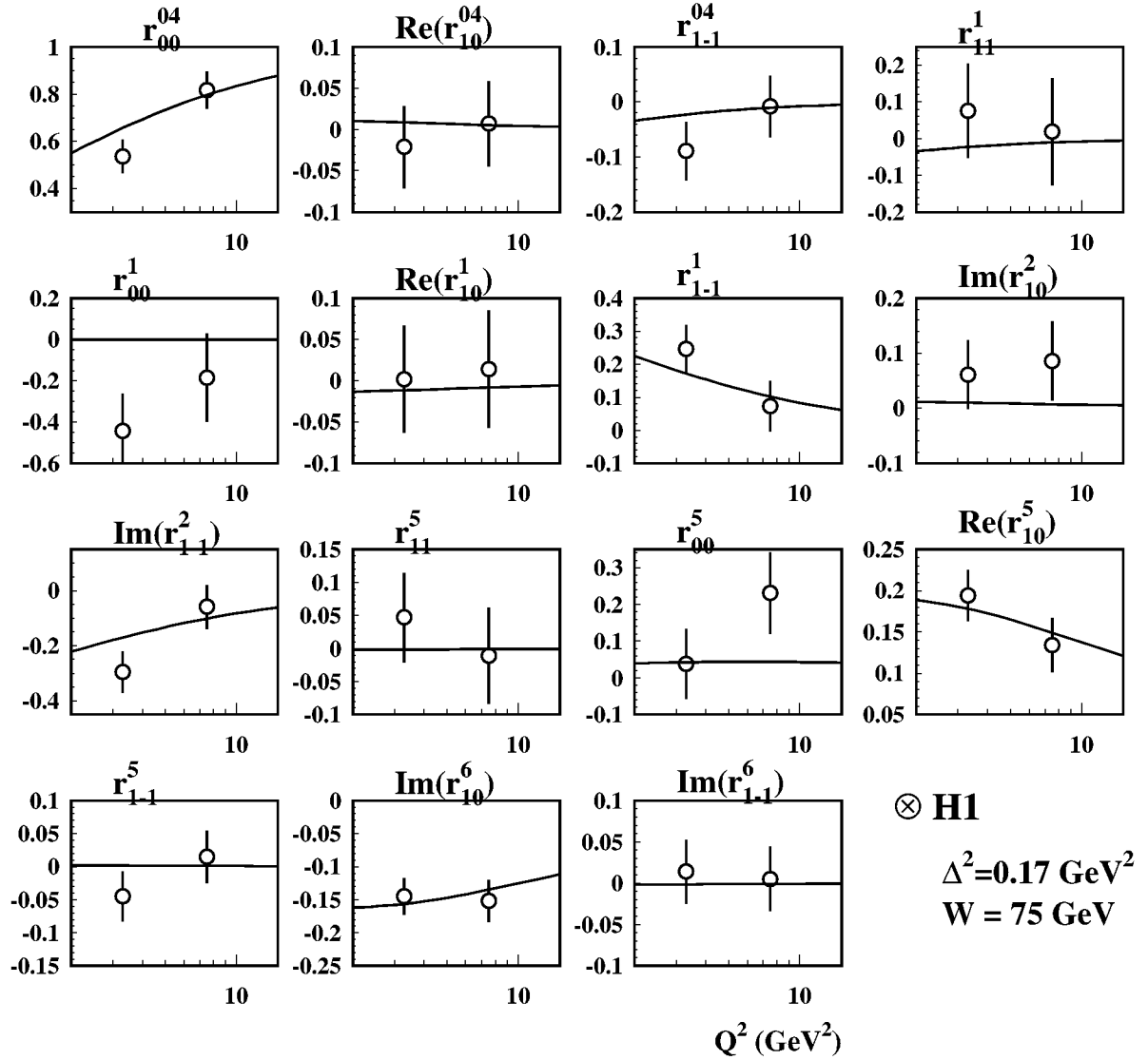
Figure 10.20: Experimental data on spin density matrix for the \phi meson production as functions of Q^2 , compared with k_t -factorization predictions based on the oscillator wave function.
