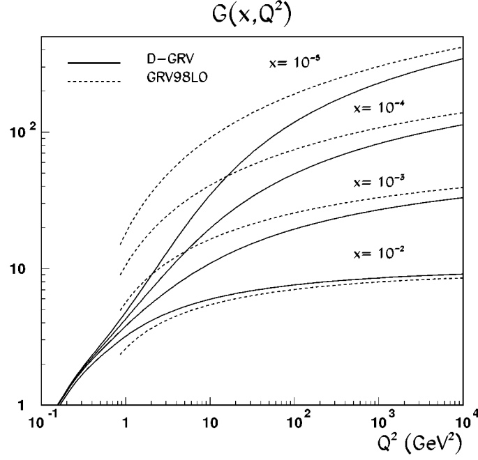
Figure 8.9: Comparison of our results for integrated gluon density G_D(x, Q^2) evaluated with the D-GRV parameterization of the differential gluon structure function \mathcal{F}(x, \vec{k}^2) with the GRV98LO DGLAP input parameterization G_{pt}(x, Q^2) .
