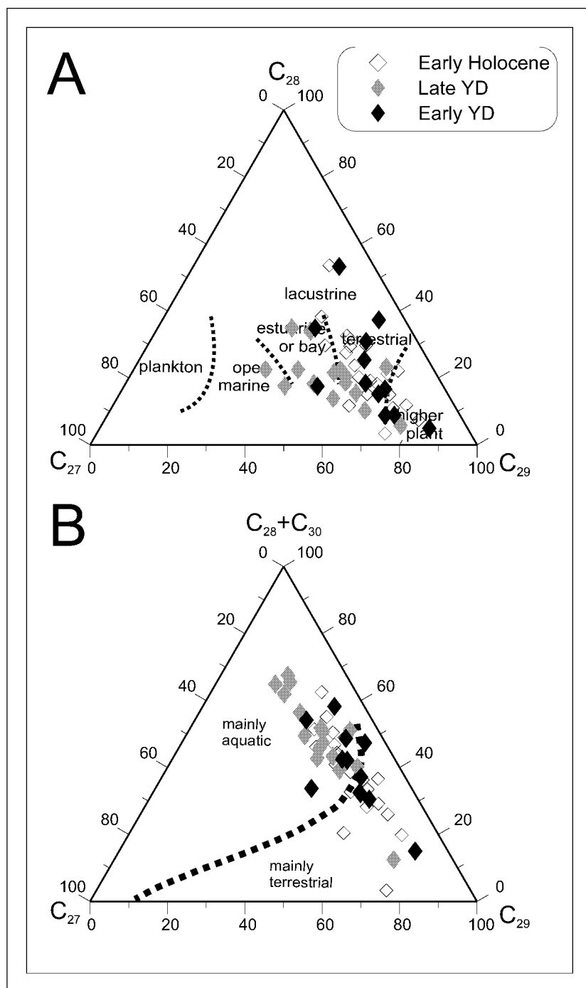
Figure 6.19: Ternary plots of sterols after Huang and Meinschein (1979) (A) and Schulte (1997) (B) for Lake Meerfelder Maar (high resolution sequence)
