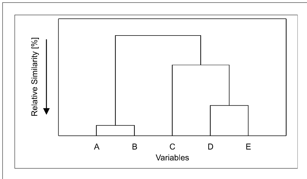
Figure 4.4: Exemplary dendrogram
