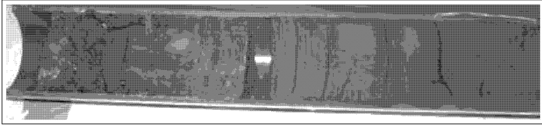
Figure 1.4: Sampled half-core section
