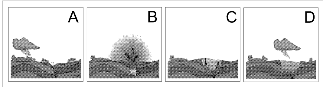
Figure 1.3: Formation of maar lake basins
