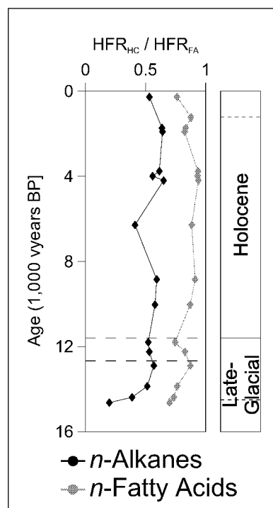
Figure 6.10: Downcore variations of HFR_{HC} (black symbols) and HFR_{FA} (grey symbols) for Lake Meerfelder Maar sedimentary sequence
