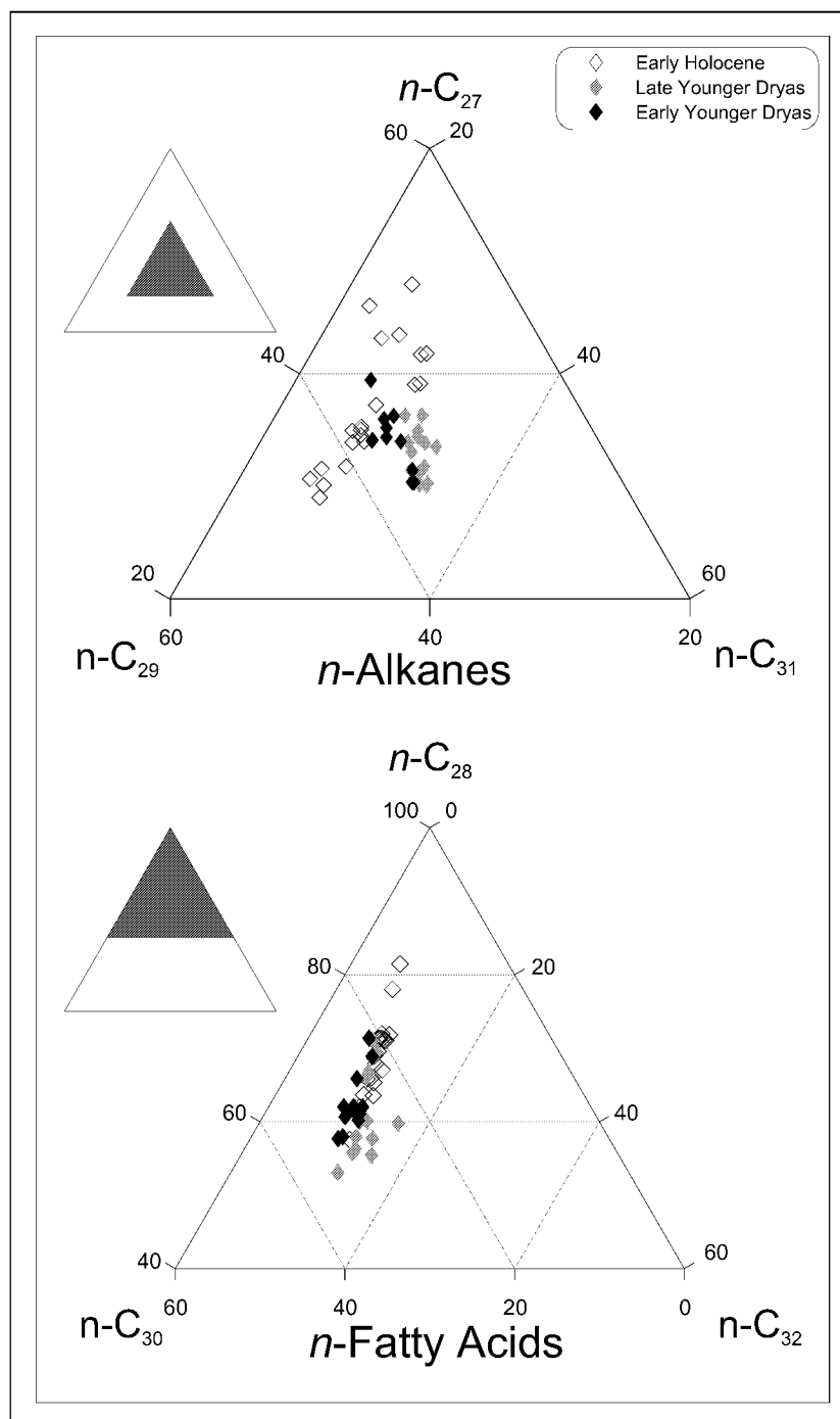
Figure 6.13: Ternary diagrams of long chain n -alkanes and n -fatty acids for the high resolution sequence of Lake Meerfelder Maar; open symbols: early Holocene; grey symbols: late Younger Dryas; black symbols: early Younger Dryas; the upper left schematics illustrate the plot areas selected for magnification out of an usual ternary plot with axes on a 0-100 scale; note, that one n -alkane data point was omitted from illustration due to plotting outside the magnification area
