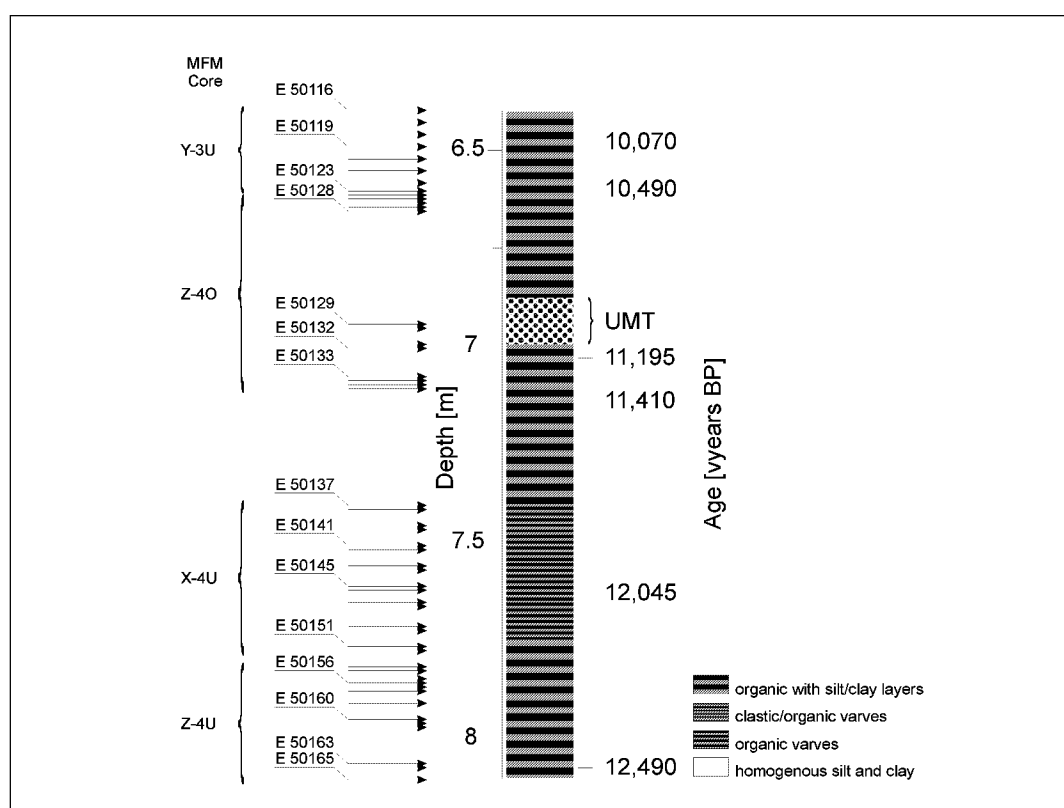
Figure 3.7: Stratigraphy of Lake Meerfelder Maars high resolved core section after Brauer (unpublished); UMT: Lake Ulmener Maar Tephra; LST: Lake Lacher See Tephra; positions of individual samples in relation to profile depth and affiliation to core sections are indicated by arrows (bulk geochemical and lipid characterisation are available for all samples)
