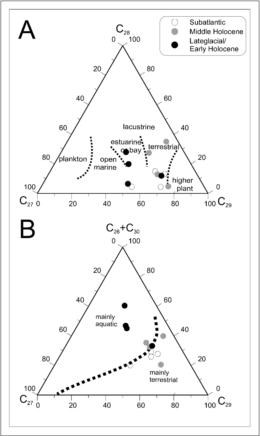
Figure 6.17: Ternary plots of sterols after Huang and Meinschein (1979) (A) and Schulte (1997) (B) for Lake Holzmaar
