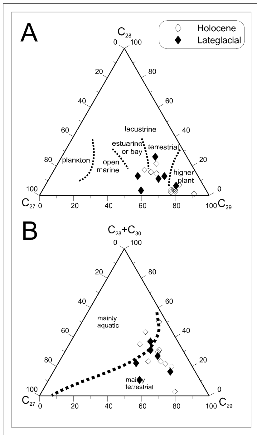
Figure 6.18: Ternary plots of sterols after Huang and Meinschein (1979) (A) and Schulte (1997) (B) for Lake Meerfelder Maar
