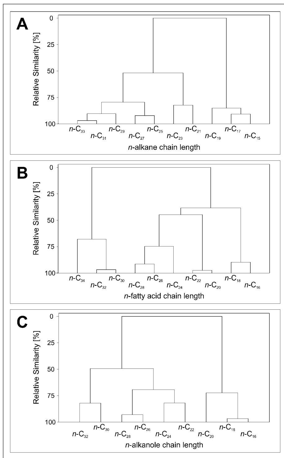
Figure 6.4: Cluster diagram for saturated n -alkanes (A), n -fatty acids (B) and n -alcohols (C), clusters for chain length using data from all investigated archives
