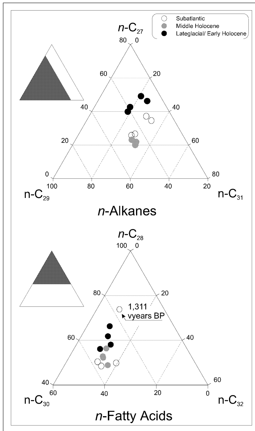
Figure 6.9: Ternary diagrams of long chain n -alkanes and n -fatty acids of Lake Holzmaar; open symbols: Subatlantic; grey symbols: middle Holocene; black symbols: Lateglacial to early Holocene; the upper left schematics illustrate the plot areas selected for magnification out of an usual ternary plot with axes on a 0-100 scale
