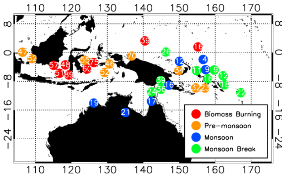
Fig. 4. Map showing the location where back trajectories that experienced rapid uplift crossed the 500 hPa surface, colour-coded to meteorological phase. The values represent the concentration of ozone recorded by ozonesonde measurements at the beginning of the back-trajectory.
