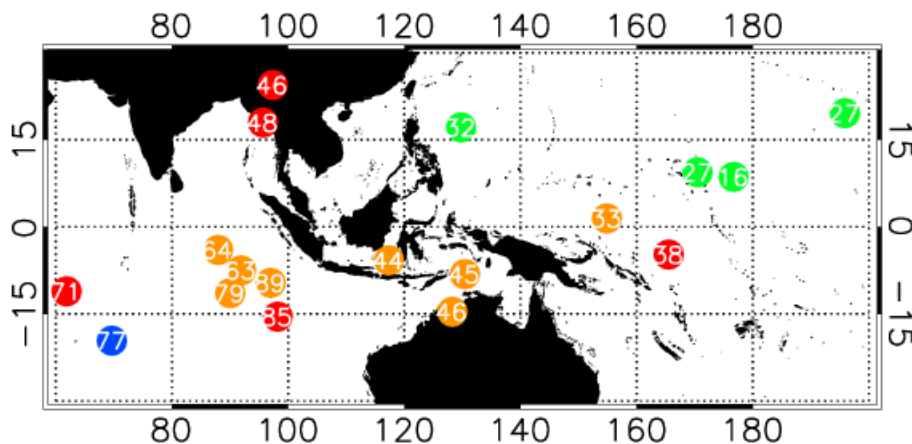
Fig. 7. Map showing the origin of 10-day back-trajectories which did not ascend from below 500 hPa, colour-coded to meteorological period, as in Fig. 4. The values represent the concentration of ozone recorded by ozonesonde measurements at the beginning of the back-trajectory.
