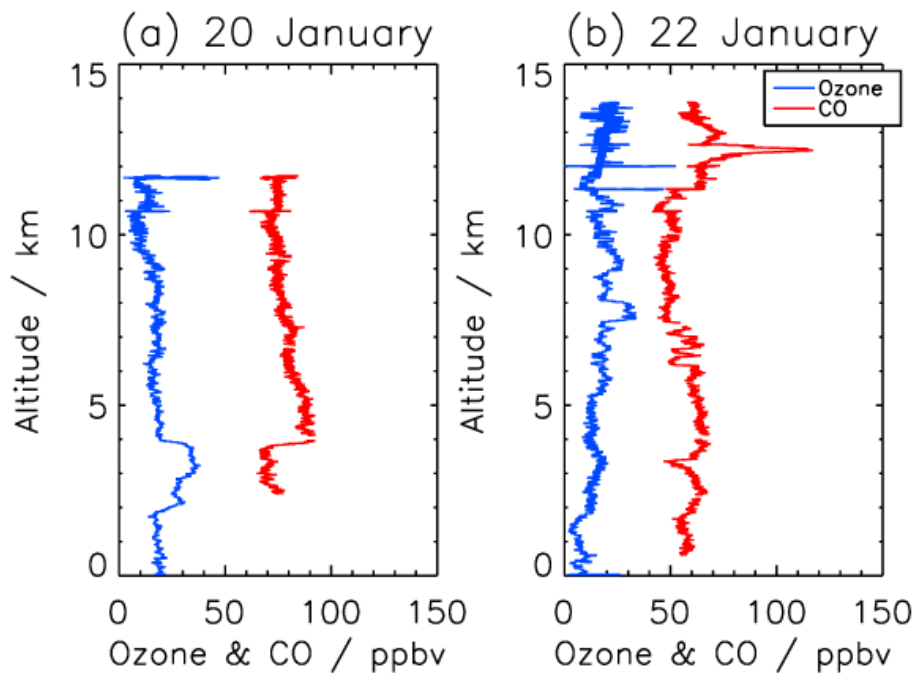
Fig. 12. Ozone and carbon monoxide vertical profiles recorded onboard the Egrett during the monsoon flight (a) AE17 on 20 January 2006 and (b) AE18 on 22 January 2006.
