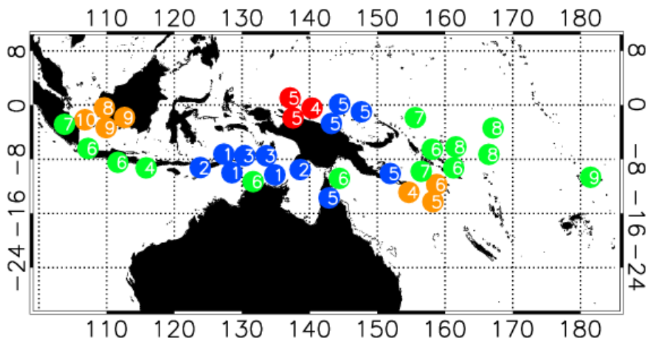
Fig. 11. As Fig. 10 where the values represent the integer number of days that the trajectories travelled before crossing the 500 hPa surface.
