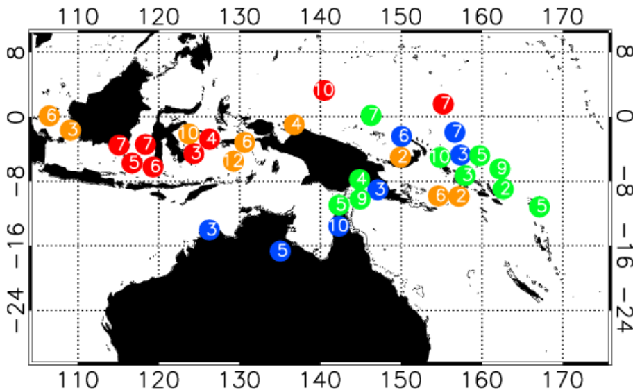
Fig. 5. As Fig. 4, where the values indicate the number of back-trajectories represented by the corresponding location.
