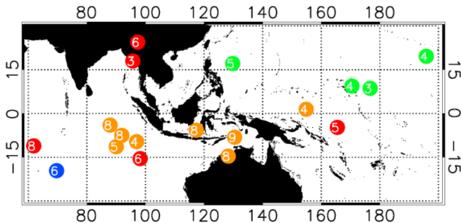
Fig. 8. As Fig. 7 where the values indicate the number of trajectories represented by the general origin location.
