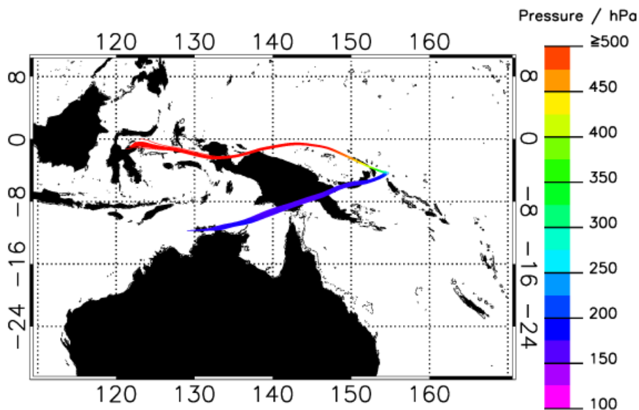
Fig. 9. An example of back-trajectories performed every 30-s from Egrett aircraft location for the transect between 09.07–09.64 UTC for flight AE27 on 10 February 2006.
