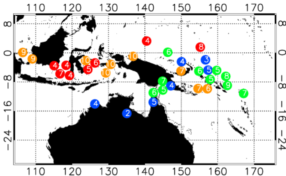
Fig. 6. As Fig. 4, where the values represent the number of integer days the associated trajectories travelled back before crossing the 500 hPa surface.
