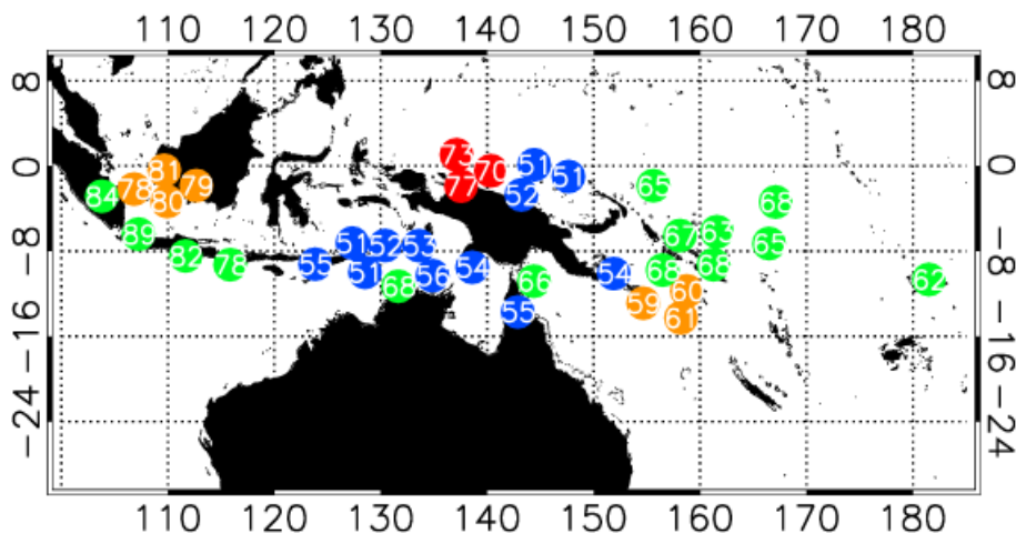
Fig. 10. Map showing the location where back trajectories that experienced rapid uplift crossed the 500 hPa surface, colour-coded to meteorological period as in Fig. 4. The values represent the average background, out-of-cloud concentration of carbon monoxide recorded on the Egrett aircraft at the beginning of the back-trajectory.
