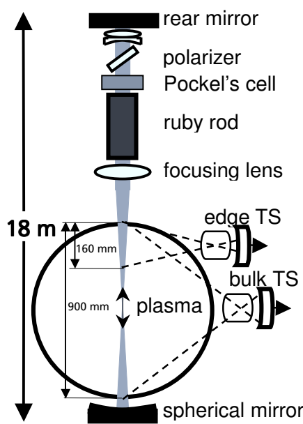
Fig 1. Schematic of the intra-cavity ruby laser at TEXTOR. The viewing lenses for bulk and edge measuring chords are also shown.
