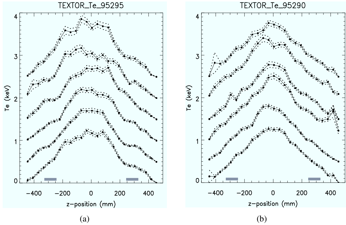
Fig 3. (a) Six T_e profiles recorded every 200 \mu s in AC DED operation. Error in the T_e measurements is plotted with dashed lines for each curve. The energy in the pulse train varied from 15 to 4 J. T_e profiles are plotted with an offset of 0.5 keV. In this case co-ECCD is applied in the plasma core ( \rho < \rho_{mode} ), leading to an enlargement of the island. The dynamic behaviour in the evolution of profile with islands is visible which repeats after one cycle of the islands rotation (b) Similar measurements at the time of co-ECCD injection inside the island to suppress the rotating islands, indicating the suppression of the islands.
