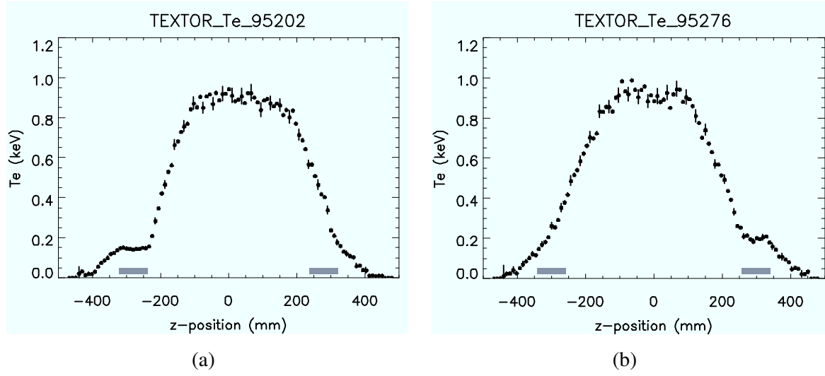
Fig 2. (a, b) Temperature profiles through different positions of a large island, measured in two different DC-DED shots. The m=2 island structures positioned around \pm 30 cm having size of \sim 8 cm (depicted by grey areas) are clearly seen in both shots. The profile perturbation by the islands is asymmetric and is consistent with the DED coil settings.
