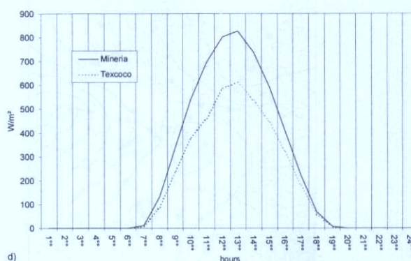
Fig. 5d: Mean diurnal range of radiation at the Mineria and Texcoco stations for the dry season months of April, October, November and December 1995
