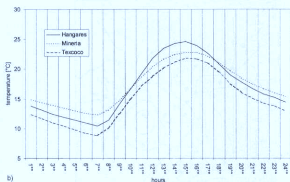
Fig. 5b: Mean diurnal range of temperature at the Hangares, Mineria and Texcoco stations for the dry season months of April, October, November and December 1995
