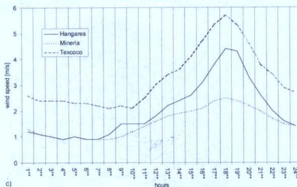
Fig. 5c: Mean diurnal range of windspeed at the Hangares, Mineria and Texcoco stations for the dry season months of April, October, November and December 1995
