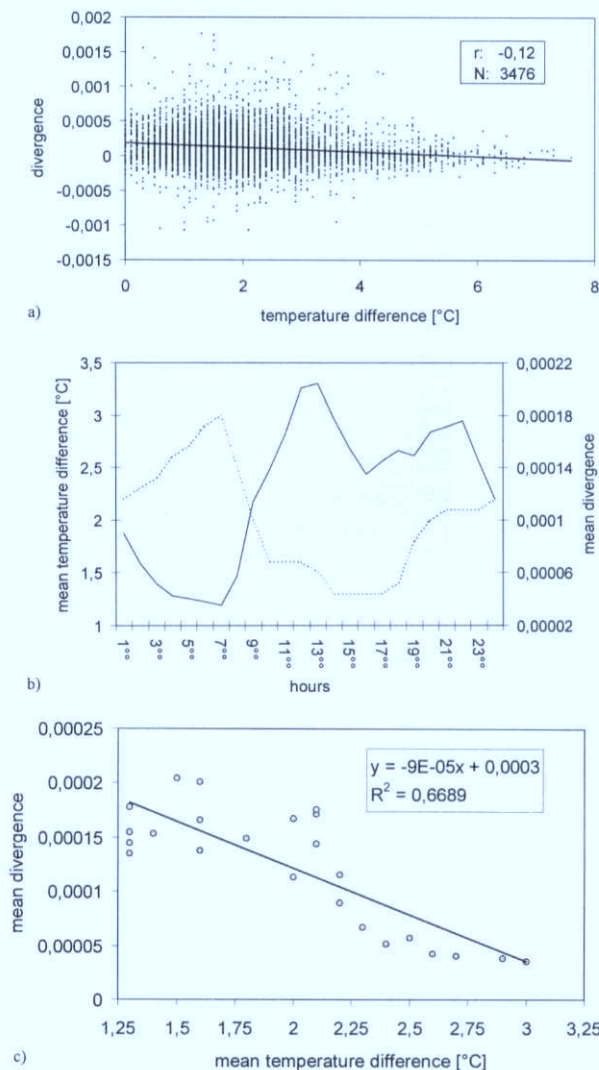
Fig. 12: Relation between the hourly temperature difference in 1995 between the city centre and surrounding area (Mineria and Texcoco) and the simultaneously occurring divergence (a). Mean diurnal range of temperature differences between the city centre and surrounding area (dashed line) and the mean diurnal range of divergences (solid line) for 1995 (b). Regression and correlation analysis of the relation between the temperature differences of the city centre/surrounding area and the simultaneously occurring average divergence values (c)
