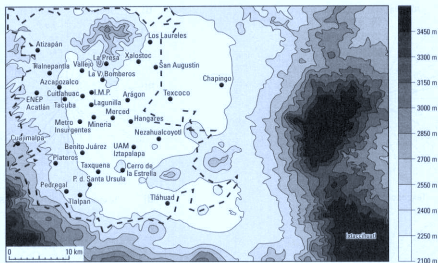
Fig. 1b: Position of Mexico City and the monitoring network in the basin of Mexico
