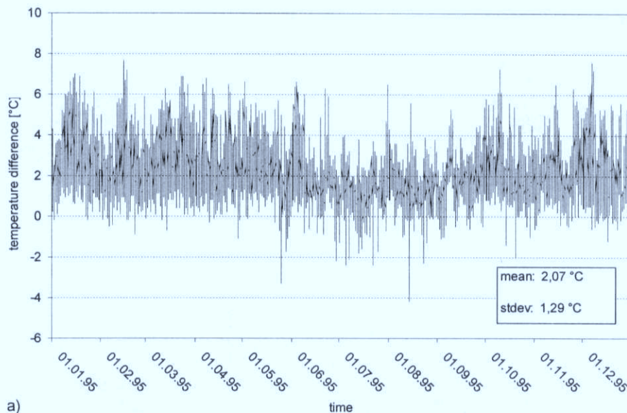
Fig. 5a: Hourly values of the temperature difference between the inner-city station at Mineria and the Texcoco station in the surrounding area in 1995
