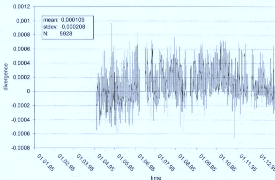
Fig. 11: Hourly values of the divergences in 1995. The values were determined according to BELLAMY's method (1949) for a triangle whose corners are occupied by the stations of Enep Acatlan (EAC), Plateros (PLA) and Texcoco (TEX)
