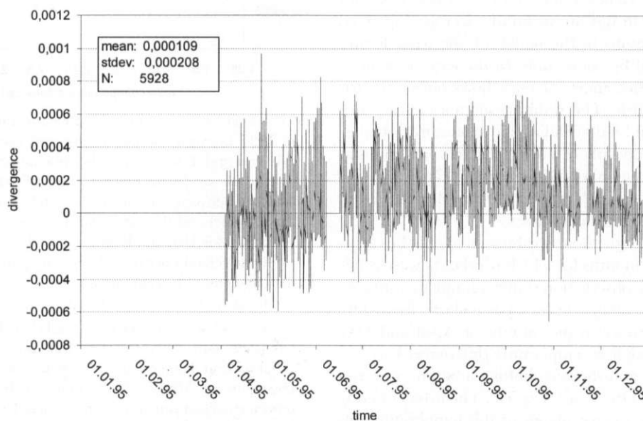
Fig 11: Hourly values of the divergences in 1995. The values were determined according to BELLAMY's method (1949) for a triangle whose corners are occupied by the stations of Enep Acatlan (EAC), Plateros (PLA) and Texcoco (TEX)
