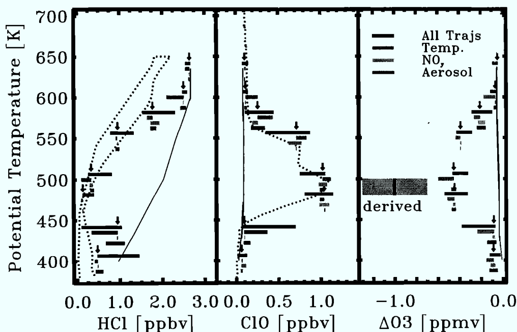
Figure 5. Results of the sensitivity study: Shown is the range of the simulated HCl and ClO mixing ratios and the simulated ozone loss induced by the variation of input parameters (temperature, -1\text{ K} , -2\text{ K} ; \text{NO}_y , \pm 2 ppbv; aerosol, \times 2 , \times \frac{1}{2} ) compared to the range of results for model runs using the set of trajectories ending around the location of the descent measurement (dotted line). The arrows mark the results of the one trajectory set used for the sensitivity study with input parameters unchanged. The runs were performed assuming a liquid PSC scheme. Results of a pure gas phase chemistry run are shown by the thin solid line.
