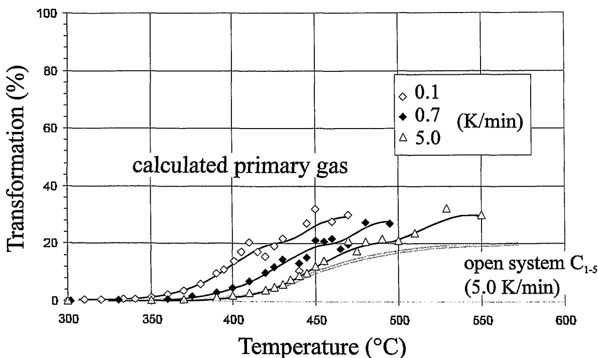
Fig. 22: Primary gas C_{1-5} generation cumulative curves. Calculated curves for MSSV pyrolysis at three heating rates and measured open system gas generation at 5.0 \text{ Kmin}^{-1} .
