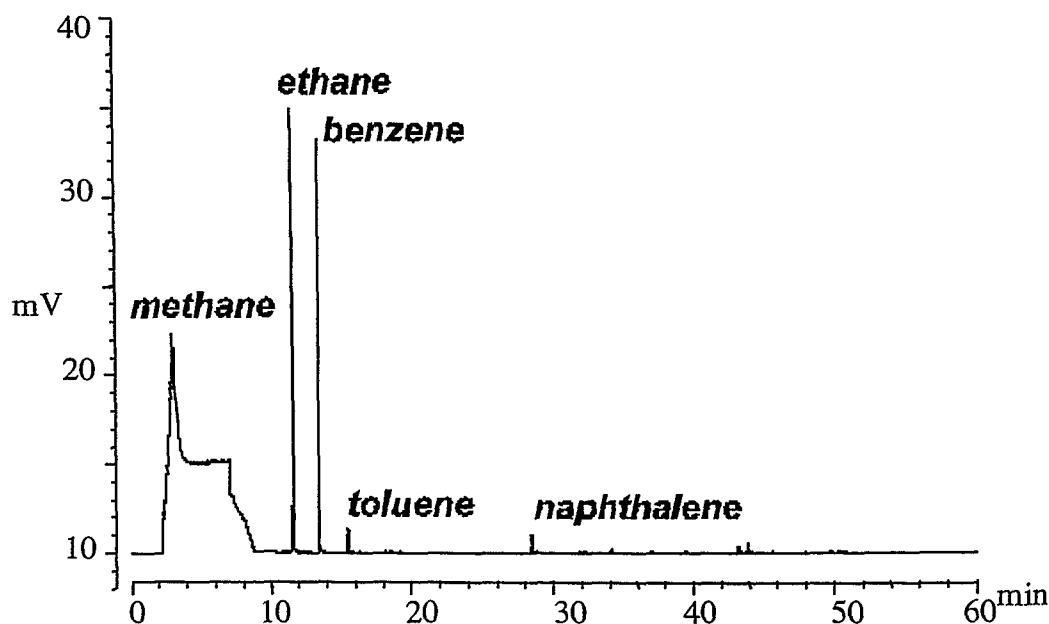
Fig. 17: Terminal MSSV pyrolysis products. Exemplified by the Draupne Formation sample (well B, E43254) at 620°C, heating rate 0.7 Kmin -1 . The presence of ethane and toluene indicates that secondary cracking is still in progress.
