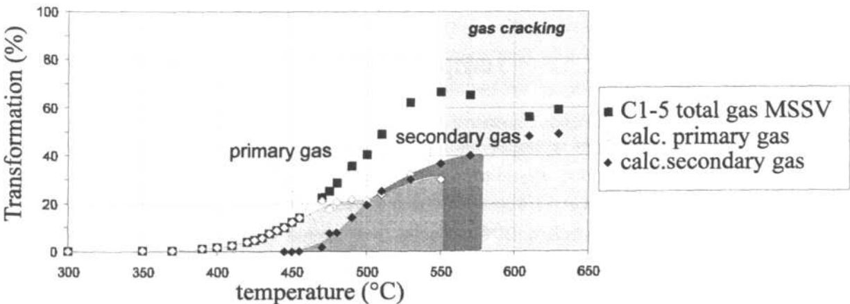
Fig. 21: Example for the results of primary and secondary gas generation evaluation using the refined mode. The sum of both curves equals the measured C 1-5 total gas curve as derived from MSSV pyrolysis at 5.0 Kmin -1 heating rate.
