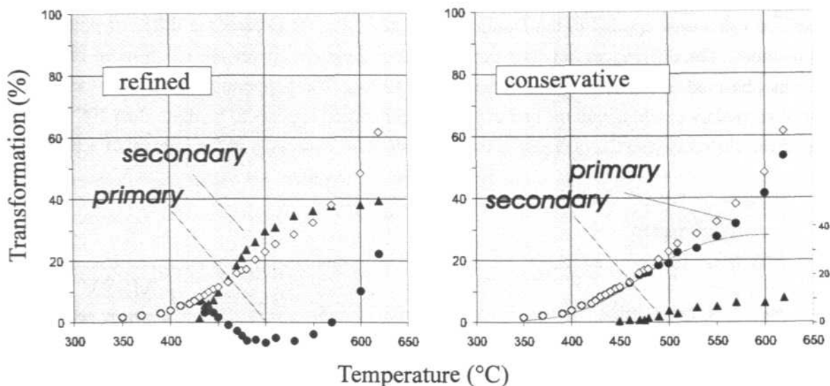
Fig. 26: Primary and secondary gas generation scenarios using the refined or the conservative evaluation method, the former was applied successfully to Draupne Formation (white rhombus total measured gas). In the right diagram the open system gas C_{1-5} generation curve shape is superimposed (thin line, different scale see Fig. 15).
