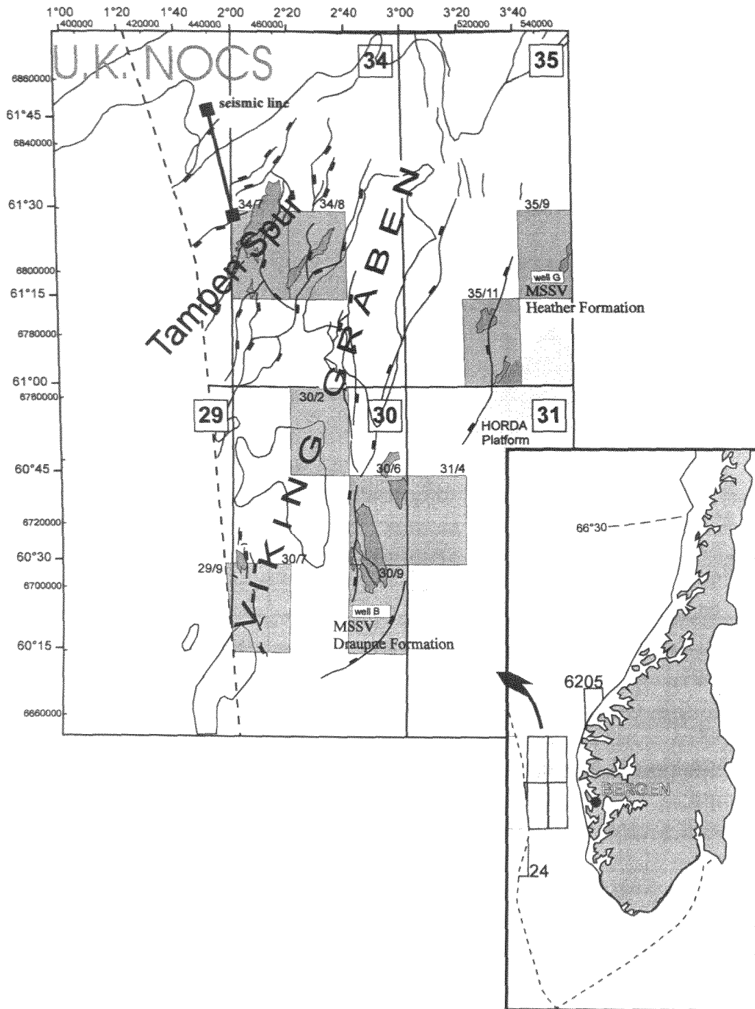
Fig. 2: Norwegian Northern North Sea quadrants. Highlighted are blocks where wells are located, major structural elements and petroleum accumulations. Locations inscribed MSSV will be referred to later. Gas kitchens (see Fig. 1) along the Graben axis are included as light grey areas. The stippled line indicates the border between the U.K. and Norwegian continental shelf.
