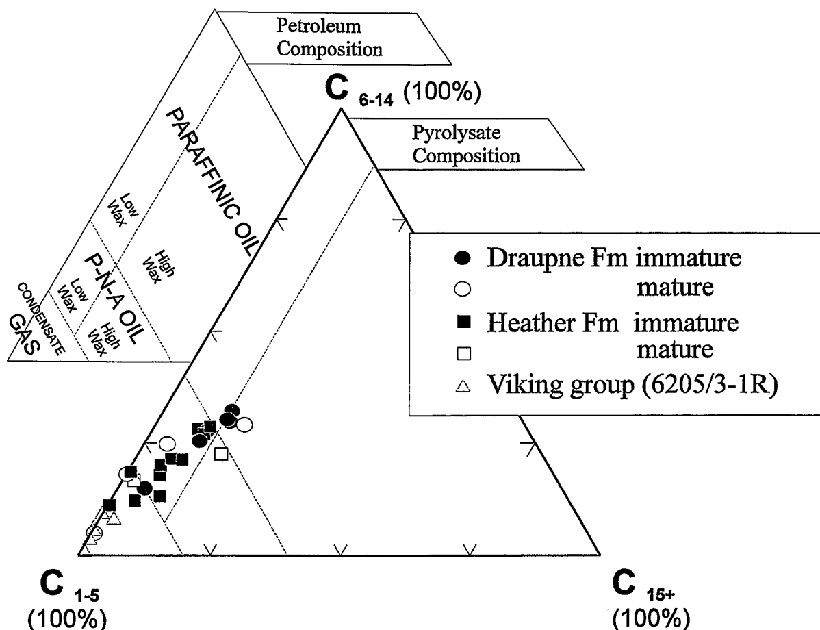
Fig. 6: Kerogen typing on the basis of alkyl-moiety distributions derived from open system pyrolysis gc (300-600°C, at 60 Kmin -1 ) modified from Horsfield (1989). For data see Table 8 in the Appendix.
