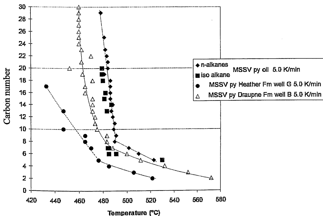
Fig. 52: Alkane inflexion-points in MSSV pyrolysis (maximum amounts, or onset of decrease) as an indicator for secondary cracking?
