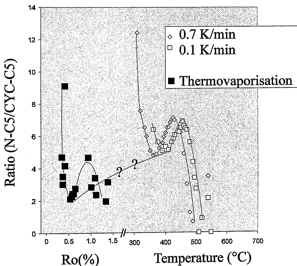
Fig. 62: Molecular ratio of n-C5 versus cyc-C5 (paraffinicity) for two heating rates of MSSV pyrolysis (Draupne Formation well B, 2764.7m) and thermal extract data of selected samples, note the different x-axis scales. Thermal extract data of the wells F and G were excluded because the suspicion of impregnation (see Figure 65).
