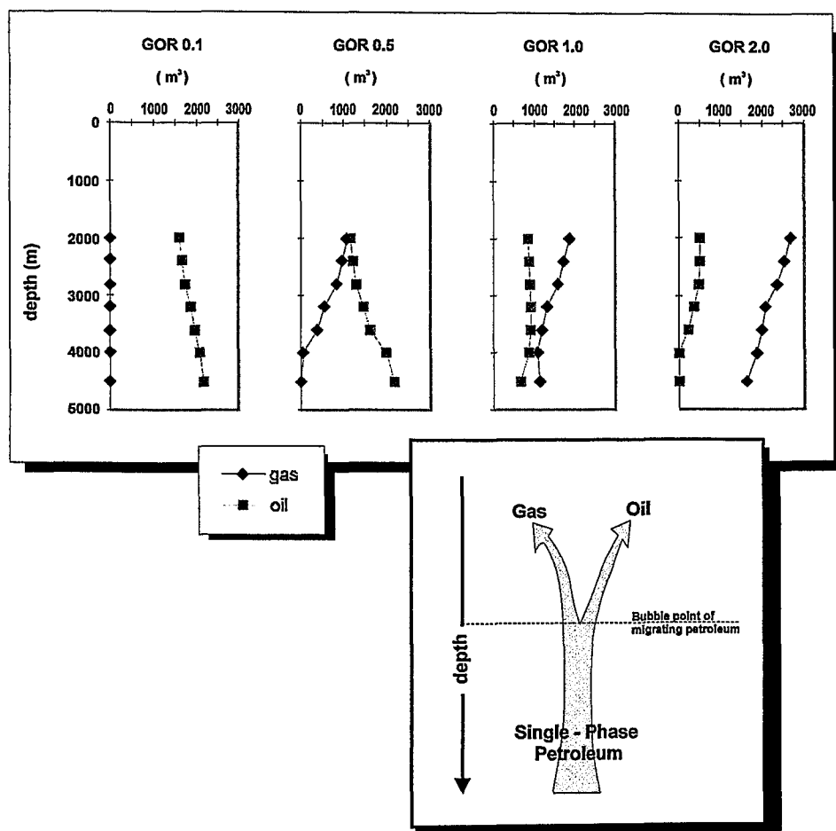
Fig. 56: Volume changes of single gas and oil phases during upward migration after phases have separated above the bubble-point. Four different initial petroleum expressed by their initial GOR's are considered (From Horsfield 1997).
