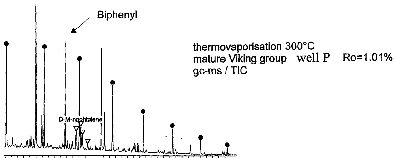
Fig. 55: Occurrence of biphenyl in high maturity settings as observed from thermovaporisation.
