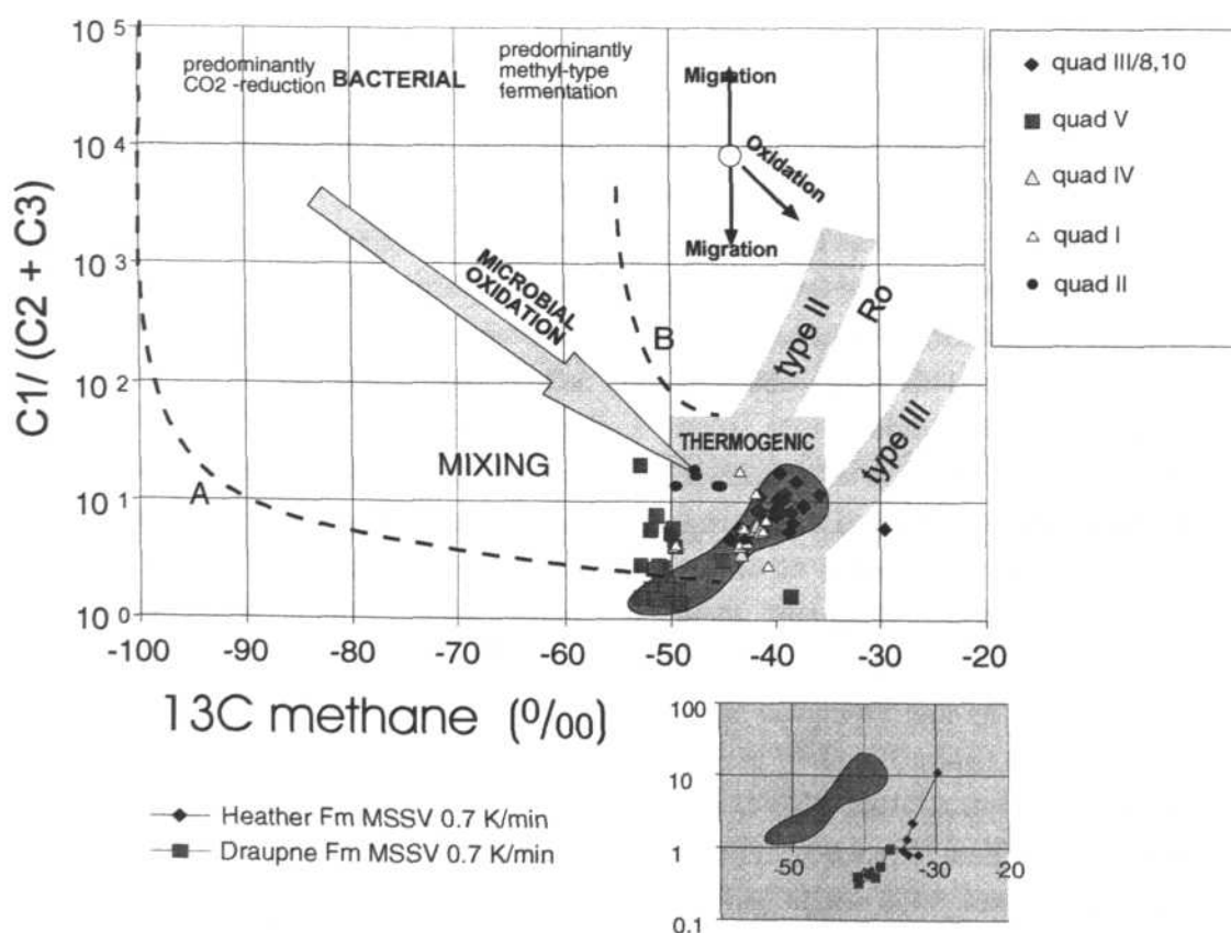
Fig. 76: Bernard plot (Bernard 1978) for Northern North Sea headspace gas data. The small diagram depicts the experimental MSSV values for Heather and Draupne Formation.
