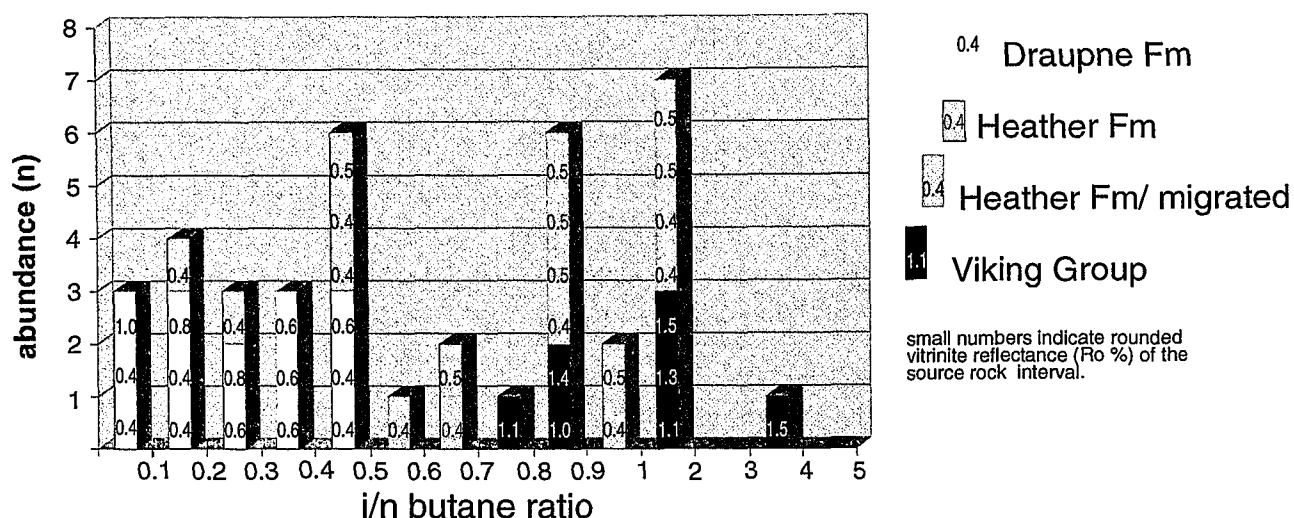
Fig. 69: Thermal extract data for Heather and Draupne Formations (quadrants Vi, I, III and IV) and Viking Group well P, Table 3.
