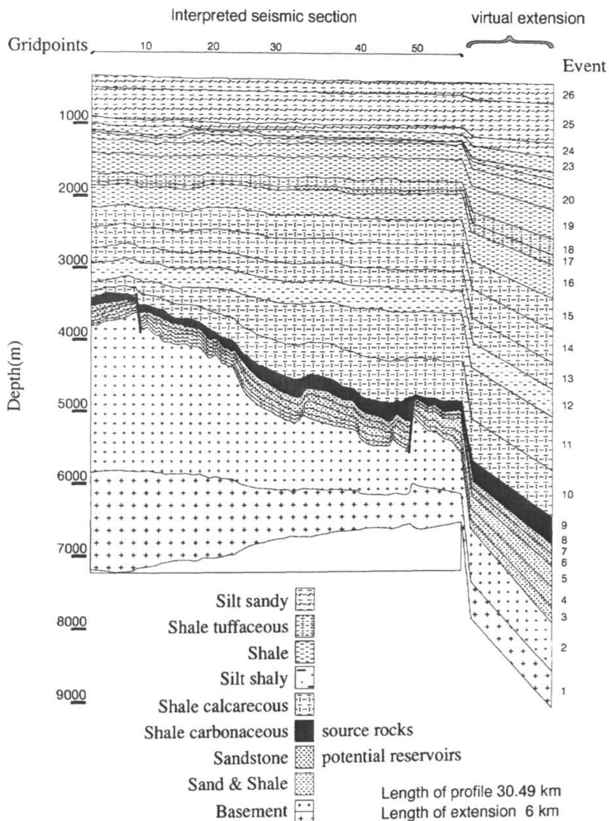
Fig. 41: Petromod-input: Interpreted seismic section including lithologies. 26 events. The section is oriented as left = south, and right = north (see Fig.2 for location).
