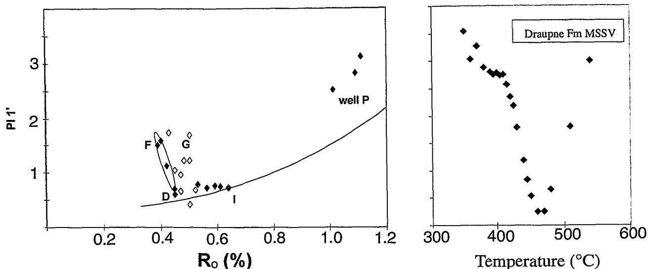
Fig. 65: The modified paraffinicity 1 (for explanation see text) molecular parameter as a function of maturity for thermal extract data and for Draupne formation MSSV pyrolysis data at a heating rate of 0.1 \text{ Kmin}^{-1} (trendline from Schaefer & Littke 1988).
