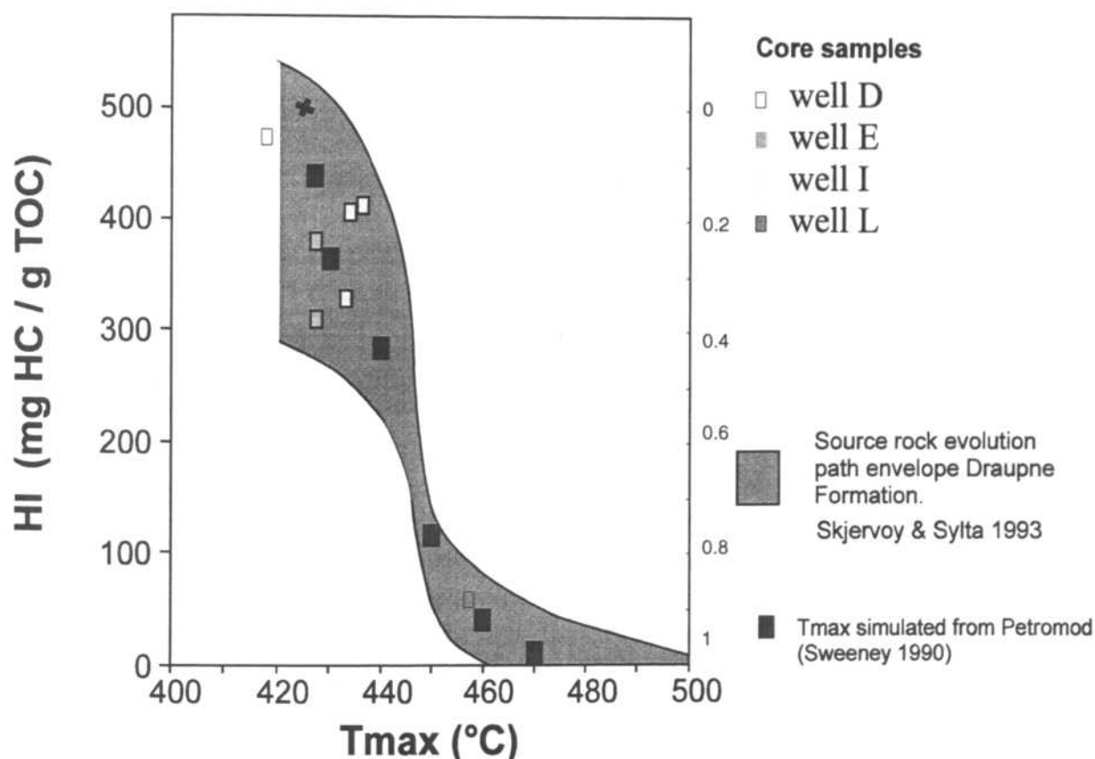
Fig. 43: Comparison of calculated Tmax for Draupne Formation with measured data. The scale on the right gives the calculated transformation ratio for an initial HI of 532 (mg/g TOC), which was used for the Draupne Formation.
