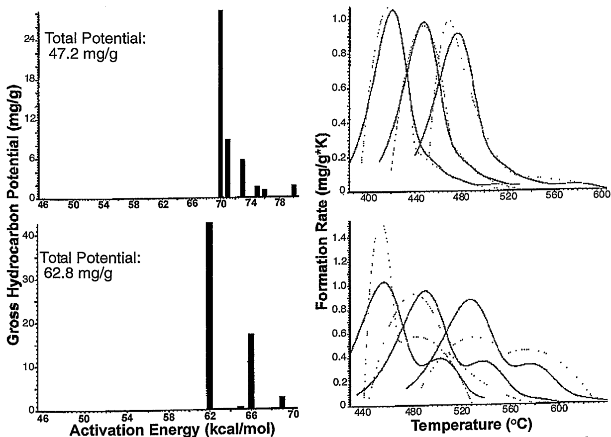
Fig. 35: Secondary gas formation from C_{6+} hump degradation (top) and C_{6+} resolved compound degradation (bottom). „Measured“ and calculated formation rates (right) and corresponding kinetic parameters (left). Draupne Formation.
