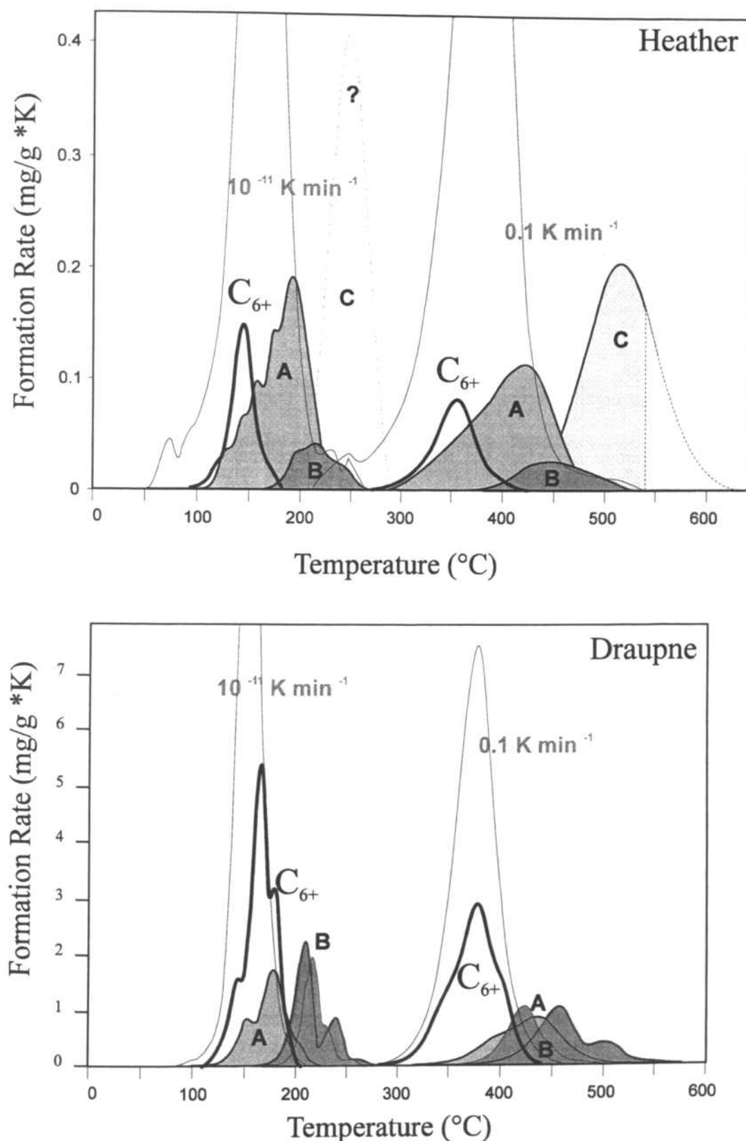
Fig. 39: Comparison of overall results. Experimental curves (right) at 0.1 \text{ K min}^{-1} and extrapolated curves (left) at 10^{-11} \text{ K min}^{-1} . Depicted are Rock Eval bulk kinetic curves (thin lines) and for MSSV pyrolysis: C_{6+} (bold lines, it is C_{6-14} for Heather Formation, for explanation see text), primary gas ( A ), secondary gas ( B ) from cracking of C_{6+} and high temperature secondary gas ( C ). Top is Heather Formation, bottom is Draupne Formation. Kinetic parameters for Rock Eval type total products and C_{6+} and C_{6-14} MSSV products are included in the Appendix.
