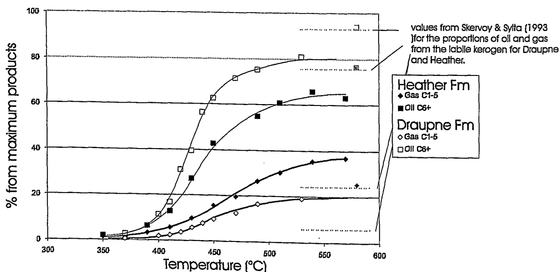
Fig. 15: Multistep open system pyrolysis at 5.0\text{ Kmin}^{-1} for Heather and Draupne Formation and in comparison with published potentials. Values are normalised to maximum product yields.
