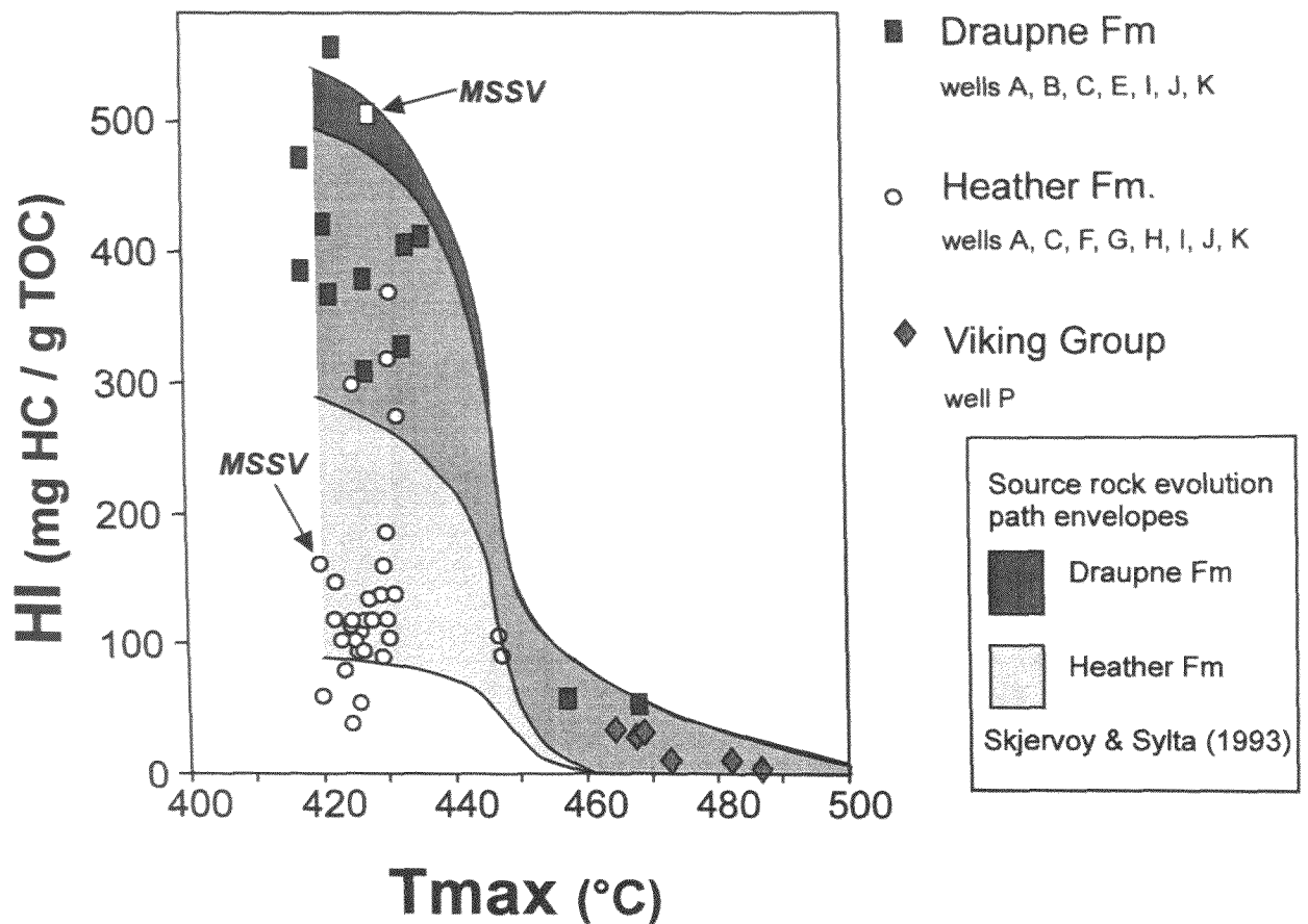
Fig. 10: Draupne and Heather Formation source rock envelopes and samples in a Rock Eval parameter plot, HI versus T_{max} . Data points highlighted by MSSV correspond to samples used for detailed investigations in the chapter "Heating Experiments".
