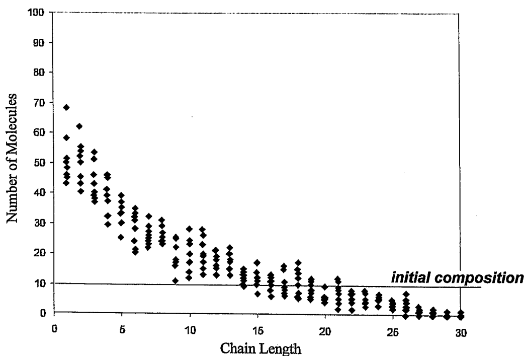
Fig. 53: Result from 1 cracking step of a mathematical random cracking model (performed 8 times. No cracking is optional).
