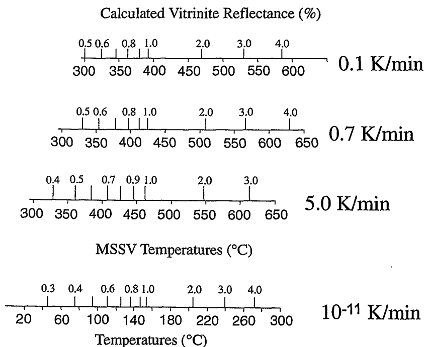
Fig. 40: Calculated vitrinite reflectance (after Sweeney and Burnham 1990, EASY Ro) correlated to pyrolysis and geological temperatures at 4 heating rates. The calculation is based on reaction kinetics for the release of methane CO 2 and water from the vitrinite. In order to provide an additional measure of maturity and because vitrinite reflectance is the most commonly used calibration parameter the correlation is included here.
