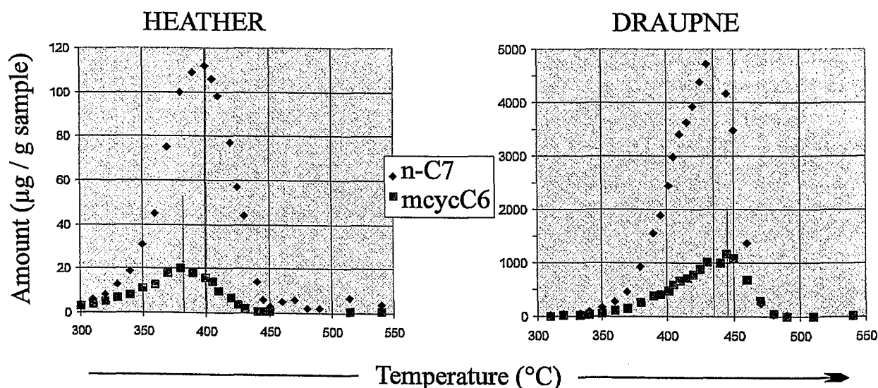
Fig. 63: MSSV pyrolysis formation curves ( 0.1 \text{ Kmin}^{-1} ) for n-heptane and methylcyclohexane for Heather Formation (well G, 2138.75m) and Draupne Formation (well B, 2764.7m). Interest is focused on the different apparent thermal stabilities of both components.
