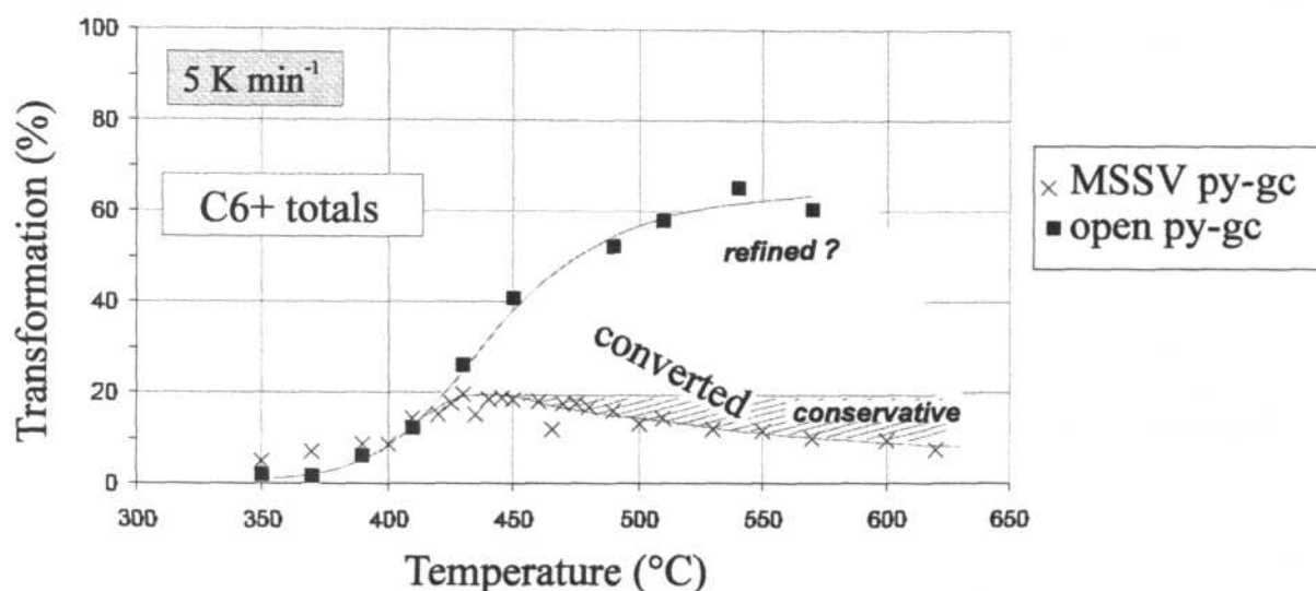
Fig. 25: Conservative and refined areas for conversion into secondary gas. The closed system transformation was calculated by using the open system as reference because the generation of products in MSSV pyrolysis was not completed.
