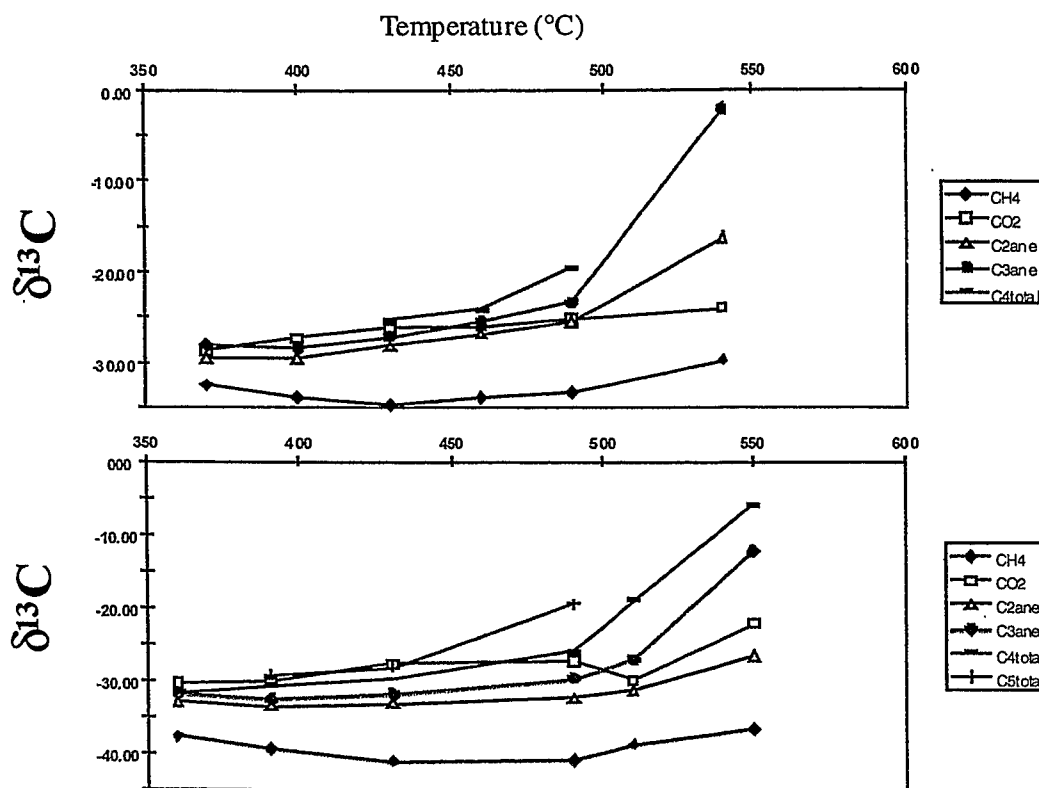
Fig. 73: \delta^{13}\text{C} isotope compositions as a function of MSSV pyrolysis temperature at a heating rate of 0.7 K/min. Top, Heather Formation and bottom Draupne Formation.
