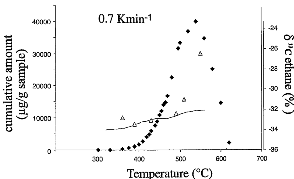
Fig. 74: Measured \delta^{13}\text{C} versus temperature for ethane of Draupne Formation (triangles) and modelled cumulative development (thin line). Rhomboids are measured MSSV pyrolysis amounts.
