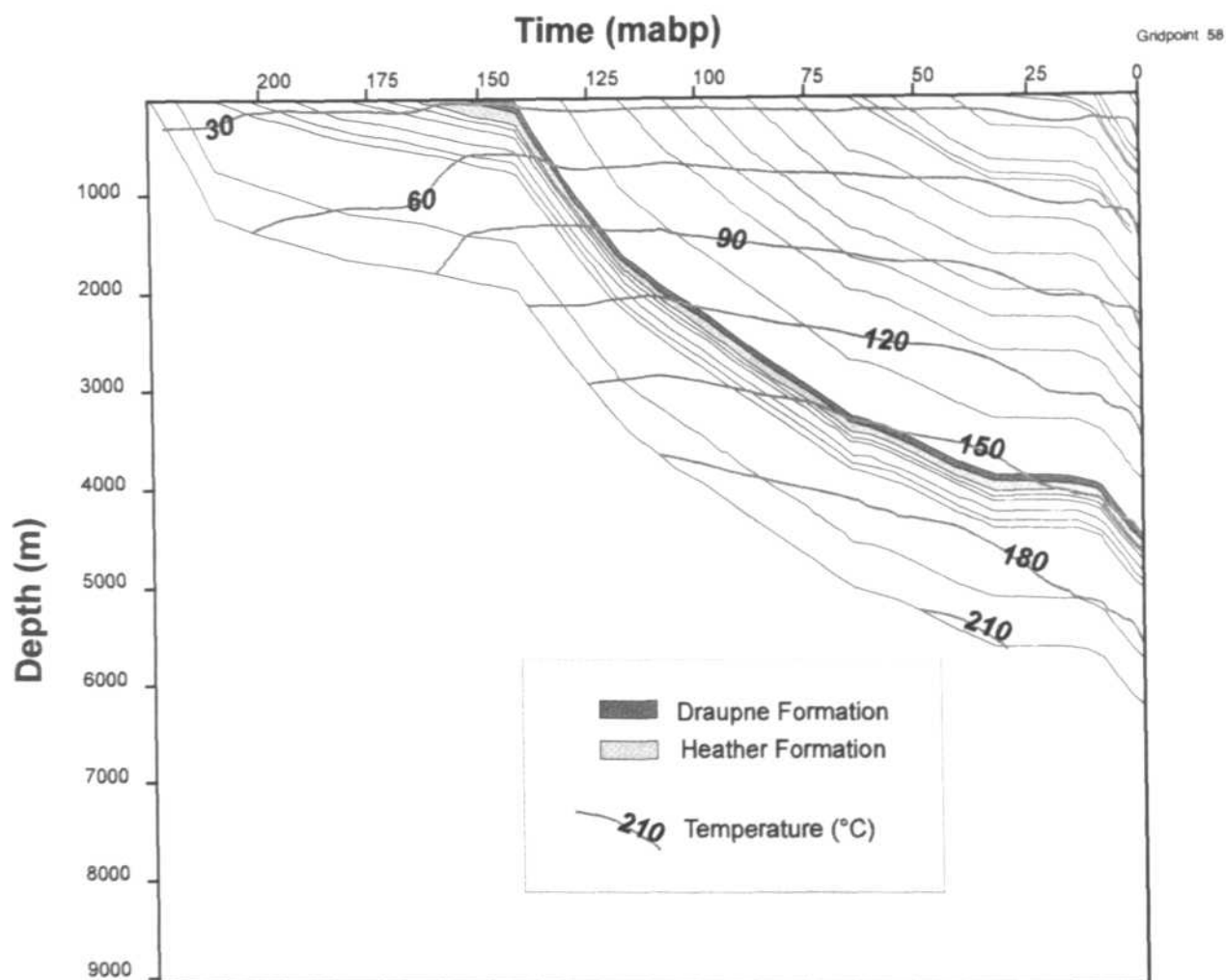
Fig. 44: Reconstructed burial history at gridpoint 58.
