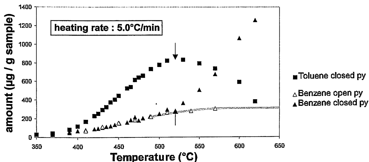
Fig. 54: Comparison of benzene formation in open and closed systems. The deviating formation curve in the closed system seems to be related to the decrease in toluene. Heather Formation.
