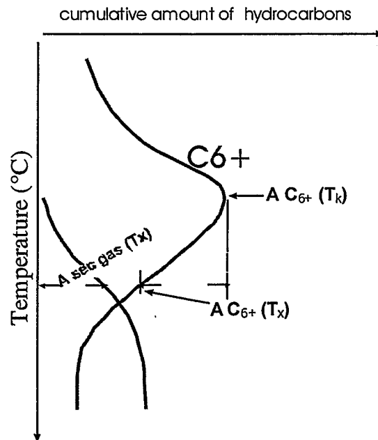
Fig. 18: Model for the calculation of secondary gas formation from the decrease of C_{6+} components.
