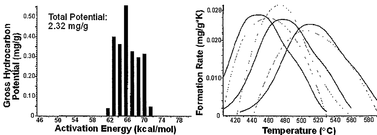
Fig. 36: Heather Formation secondary gas from C_{6+} degradation. Right: "measured" and calculated formation rate curves for three heating rates. Left: Corresponding kinetic parameter set.
