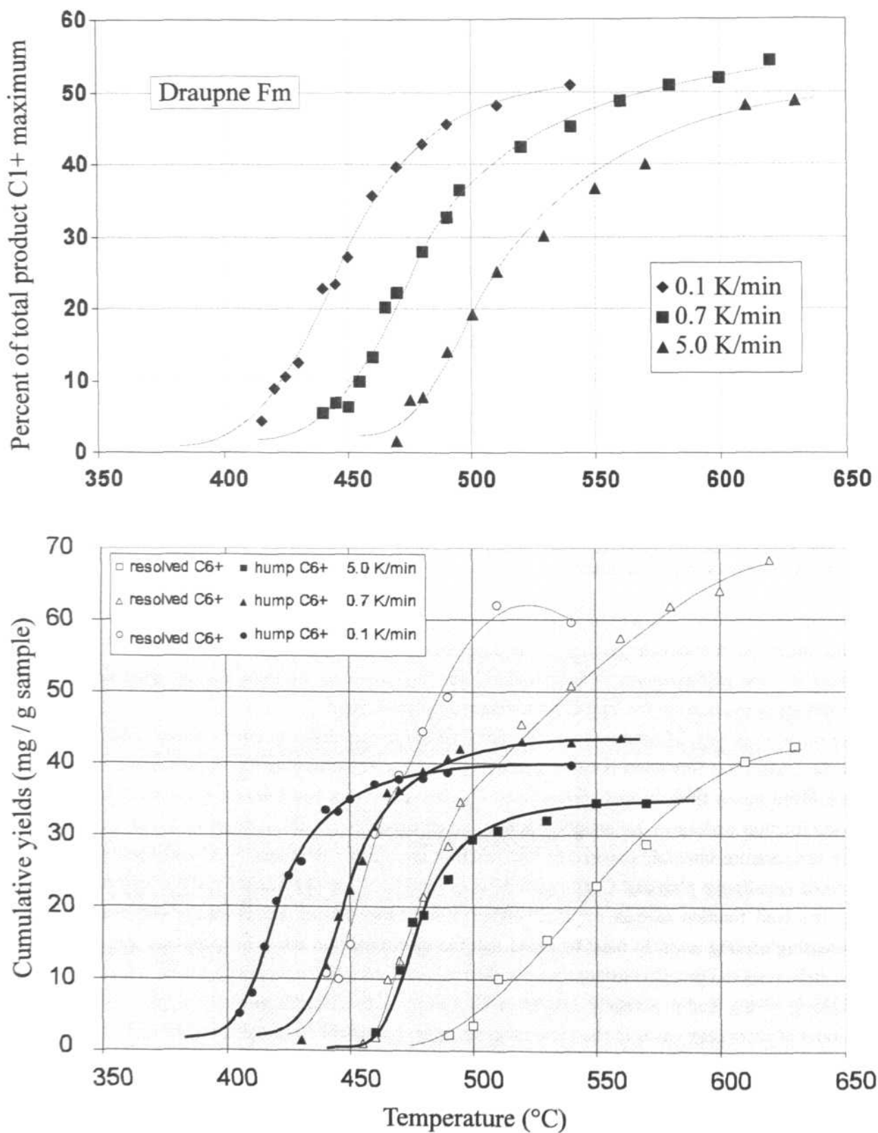
Fig. 24: The diagram at the top displays essentially the same curves as depicted in Fig. 23 but values are normalised to C 1+ cumulative maximum yields. The bottom diagram shows secondary gas discriminated into a C 6+ resolved fraction and C 6+ hump.
