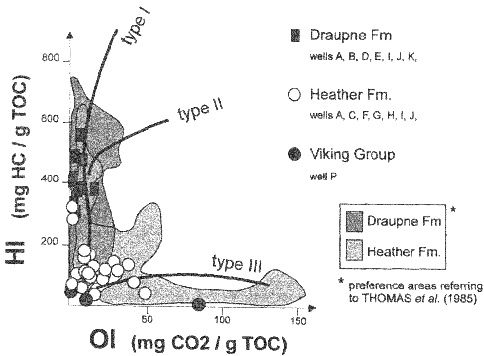
Fig. 4: Kerogen type discrimination on the basis of the Rock Eval parameters Hydrogen Index (HI) and Oxygen Index (OI).
