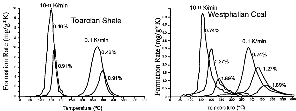
Fig. 11: Total product formation rate curves for samples of increasing natural maturation (given in % vitrinite reflectance), Toarcian Shale and Westphalian Coal. From Schenk & Horsfield (1996).
