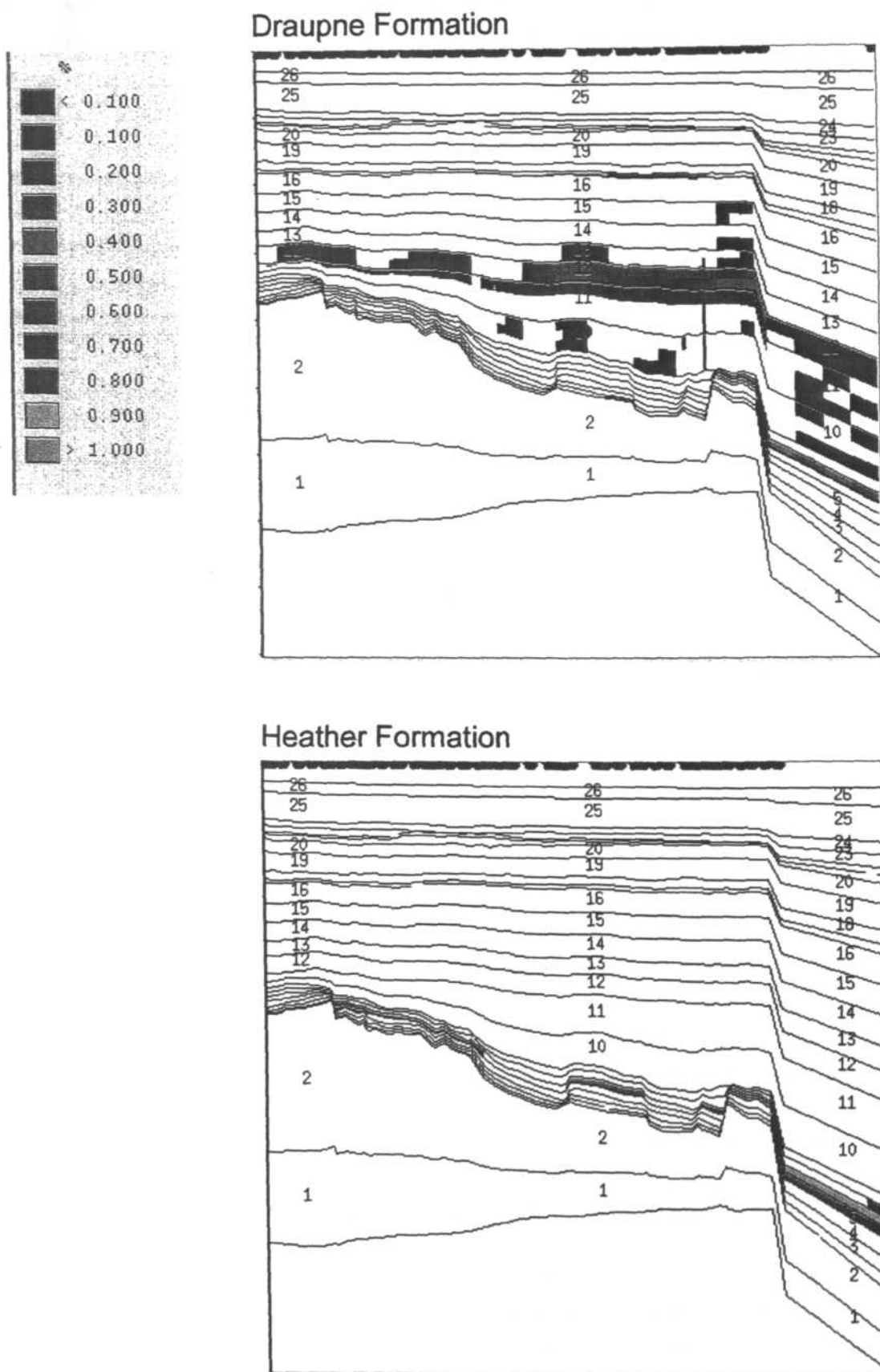
Fig. 48: Petroleum (both oil and gas) saturation expressed as % of pore space. South = left, North = right.
