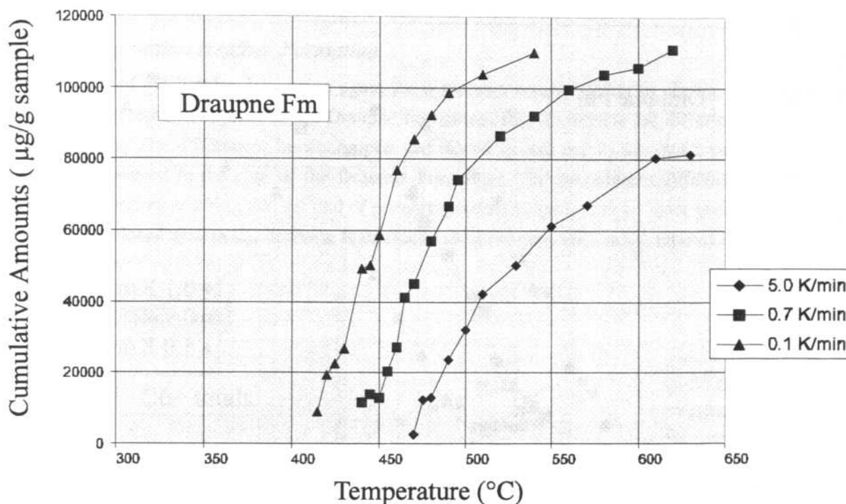
Fig. 23: Draupne Formation secondary gas formation curves. Calculated with the refined evaluation from MSSV pyrolysis at three heating rates.
