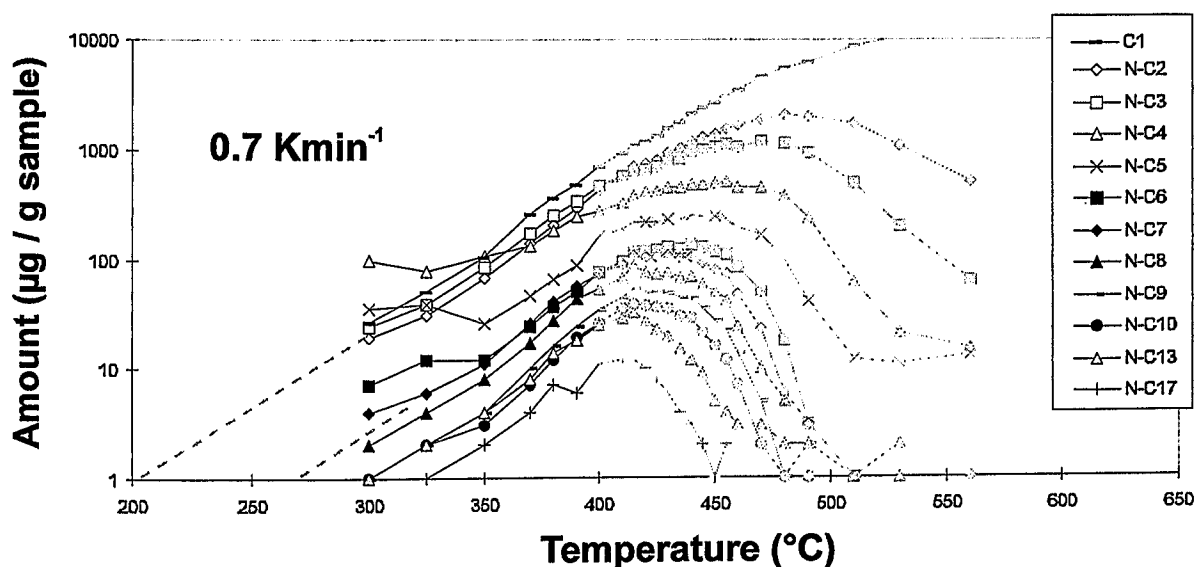
Fig. 50: Formation of n-alkanes during MSSV pyrolysis of the Heather Formation samples. The range which is likely to be exclusively affected by primary cracking reactions is highlighted. The general trends can be observed for Draupne Formation as well (not depicted) and are similar for all heating rates.
