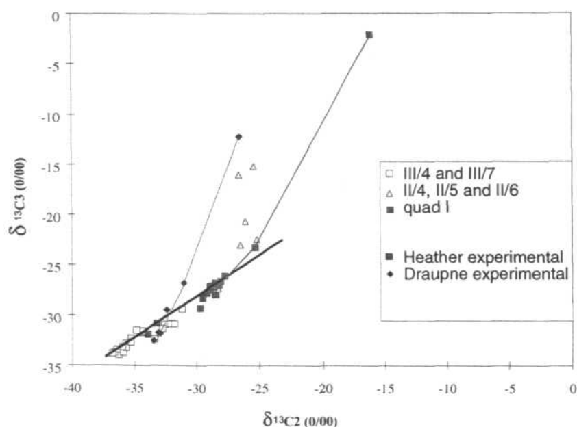
Fig. 75: Experimental ethane versus propane \delta^{13}\text{C} values compared to headspace gas data from the Viking Graben.
