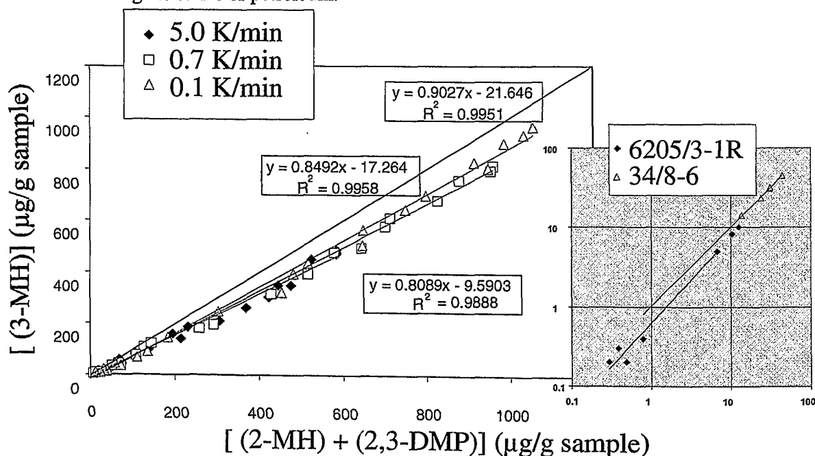
Fig. 59: Molecular ratio [(3\text{-MH}) + (2,4\text{-DMP})] / [(2\text{-MH}) + (2,3\text{-DMP})] modified after Mango (1987) from MSSV pyrolysis Draupne Formation well B (2764,7m). 2-MH = 2-methylhexane, 3-MH = 3-methylhexane, 2,3- DMP = 2,3-dimethylpentane. 2,4-DMP= 2,4-dimethylpentane is not included (see text).
