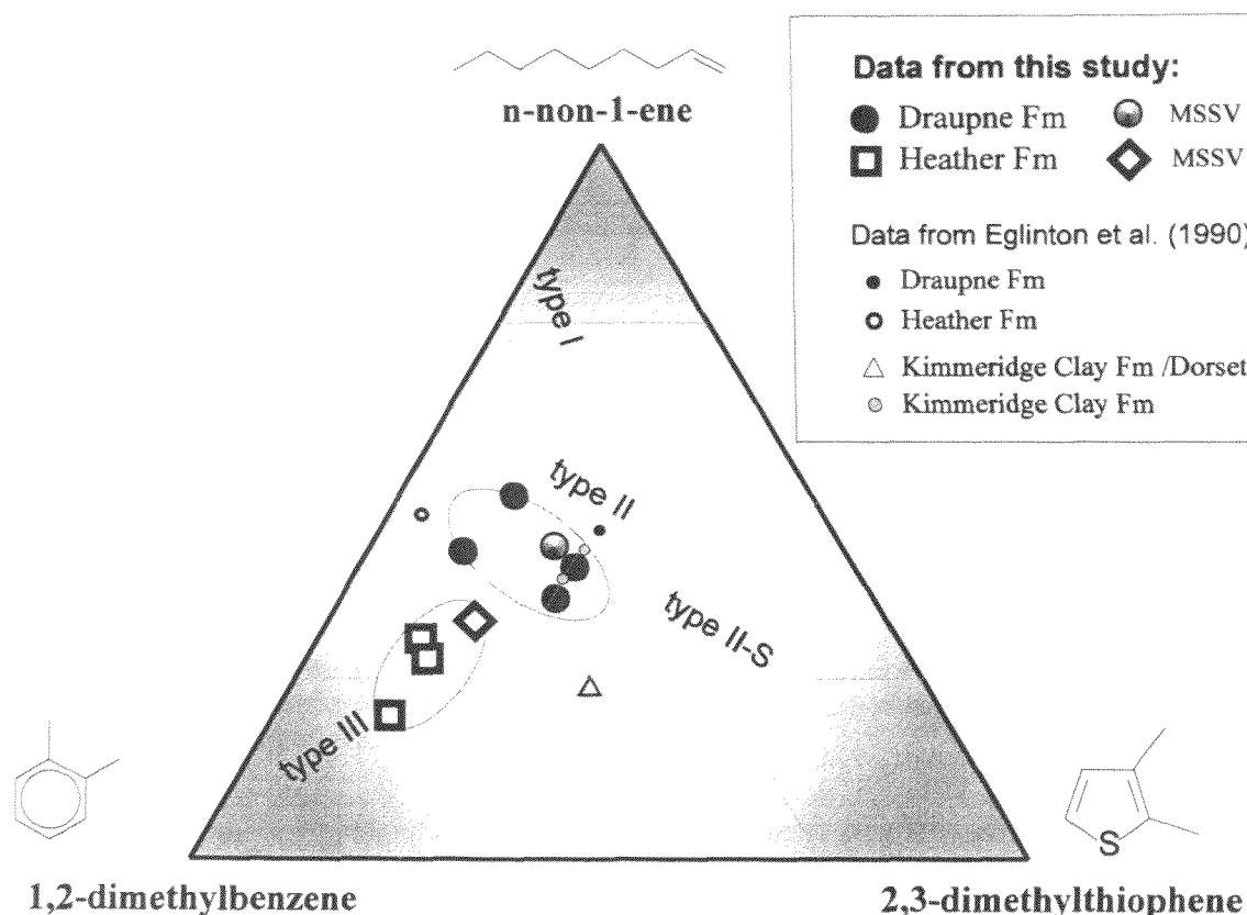
Fig. 7: Ternary diagram modified from Eglinton et al. (1990), scales are from 0 - 100 percent. Kerogen typing using aromatic, sulphur-containing and alkyl- compound groups. Two samples, termed MSSV are also highlighted, but are discussed later in the course of this study (in "Heating Experiments").
