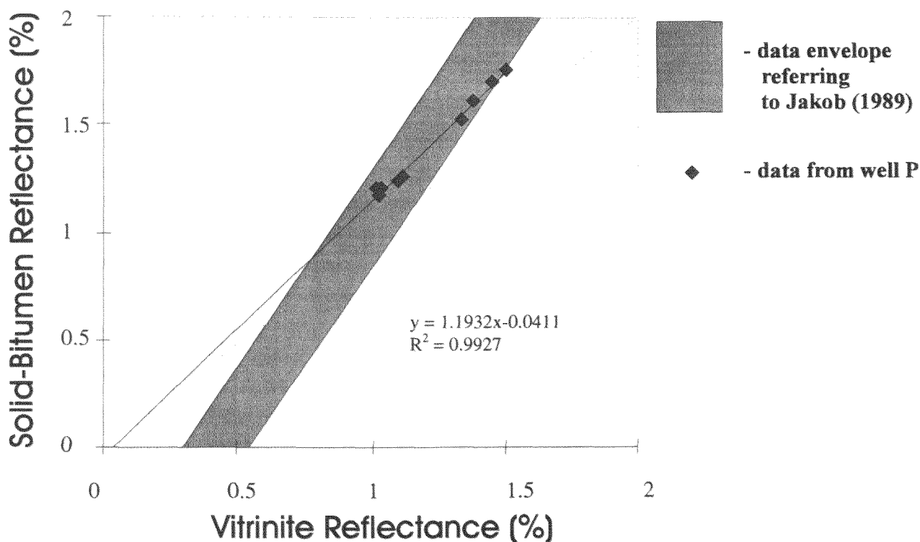
Fig. 9: Correlation between changes in vitrinite reflectance and pyro- or solid-bitumen reflectance.
