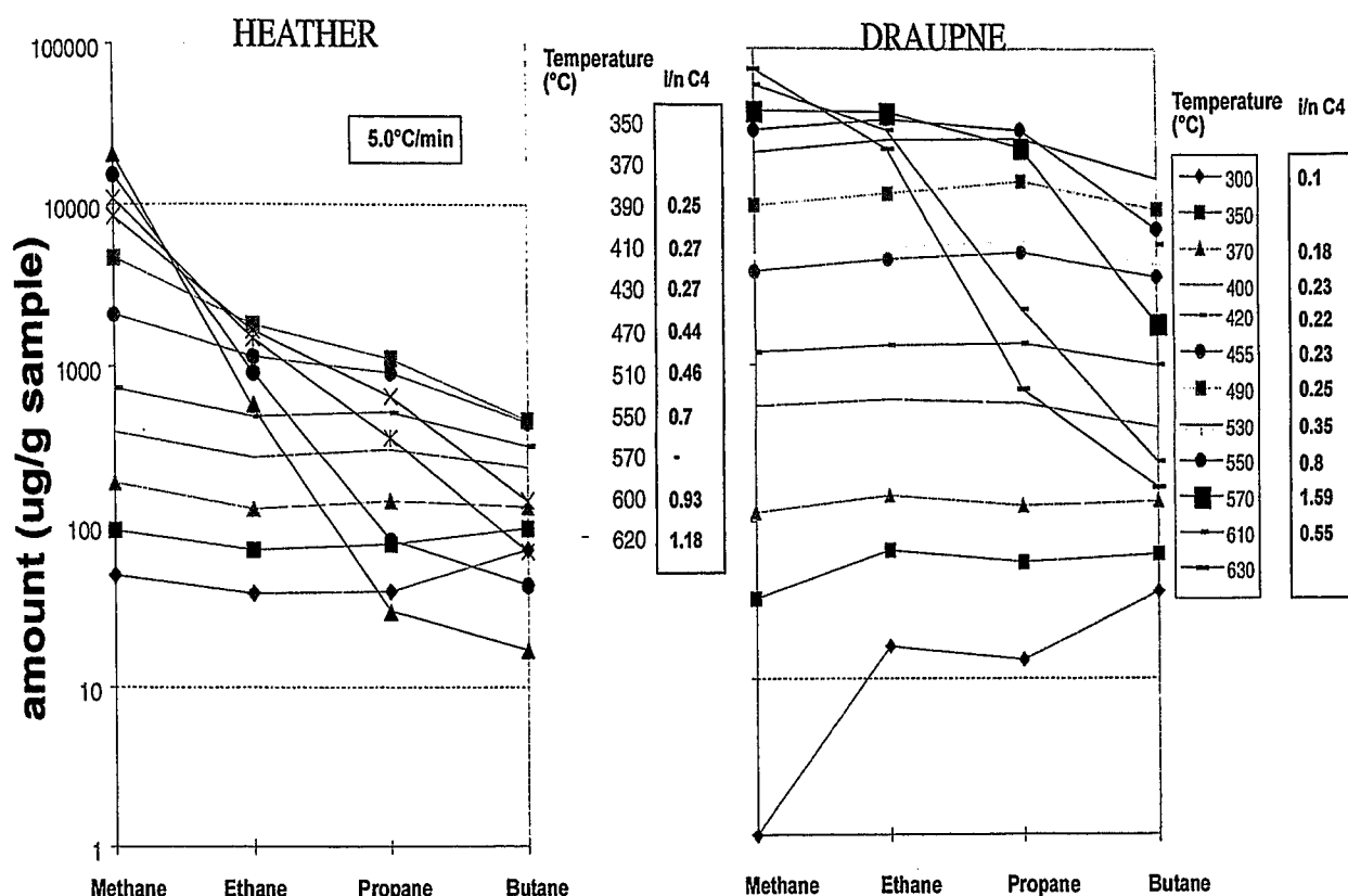
Fig. 70: Compositional evolution of C_{1-4} gas components during MSSV pyrolysis at a heating rate of 5.0 \text{ Kmin}^{-1} for Heather and Draupne Formation.
