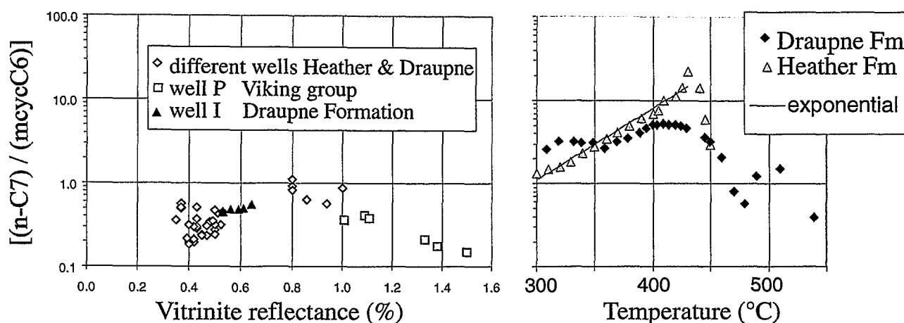
Fig. 64: Paraffinicity 2 (Thompson 1979) for thermal extract data and MSSV pyrolysis (0.1 K/min).
