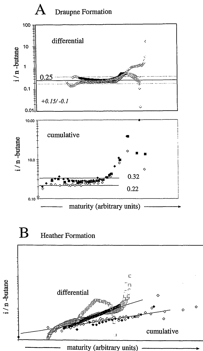
Fig. 67: Molecular ratio i/n butane from MSSV pyrolysis for Draupne and Heather Formation at three heating rates ( 0.1, 0.7, 5.0 \text{ Kmin}^{-1} ). The ratio was calculated from the cumulative MSSV curves i.e. including decrease by secondary cracking at higher temperatures, and from spline approximated and differentiated curves i.e. without regard of secondary cracking. The curves are shifted in temperature direction until best match was obtained.
