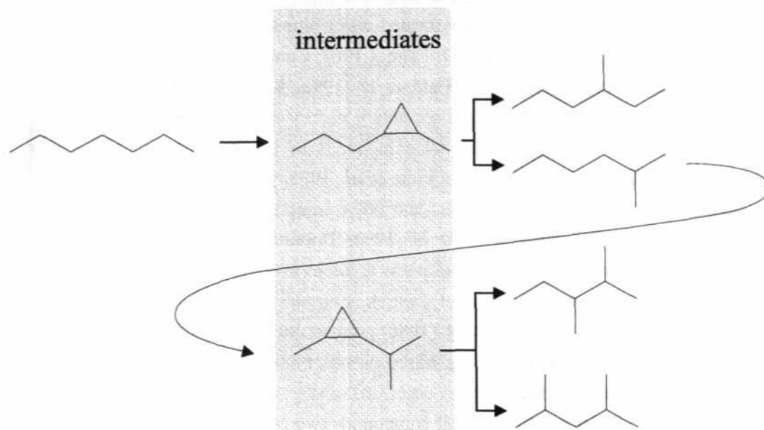
Fig. 13: Reaction scheme after Mango (1987) for the formation of isoheptanes by a steady state catalytic process over short-lived unstable cyclopropane intermediates.
