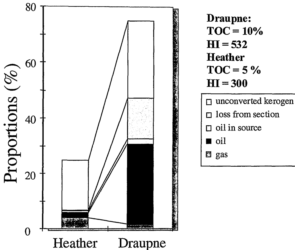
Fig. 46: Mass balance for the present day situation. The depicted distribution results from both generation and migration. Losses from the section are upward losses as basin sides were modelled as closed.
