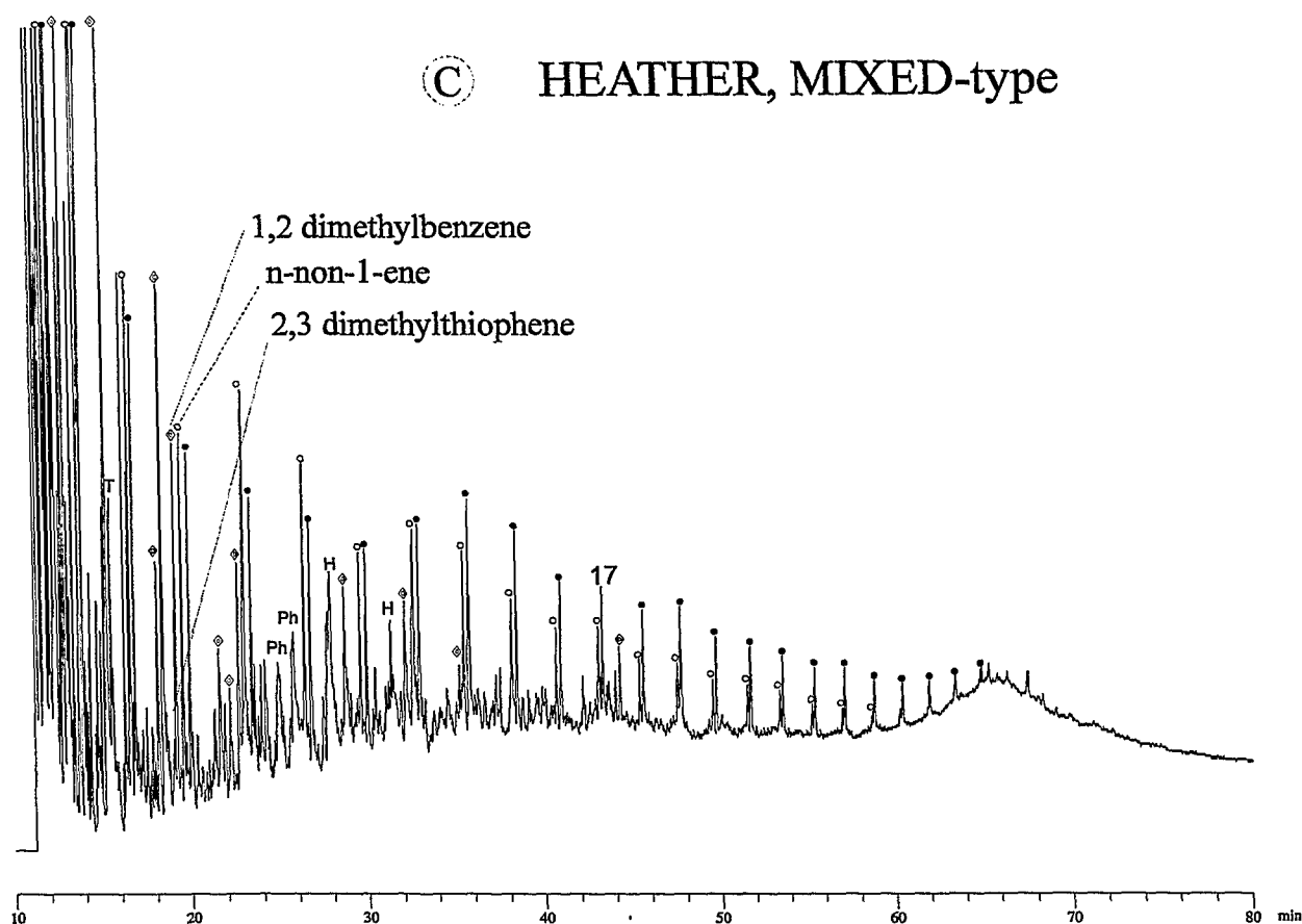
Fig. 5: Open pyrolysis gas-chromatography FID (300-600°C, at 60 Kmin -1 ). A: Draupne Formation well B (2764.7m), B: Upper Heather Formation well G (2134.95m) and C: Lower Heather Formation well G (2546.9m). The three highlighted peaks are used for kerogen characterisation (page 24) in a ternary diagram according to Eglinton et al. (1990).
