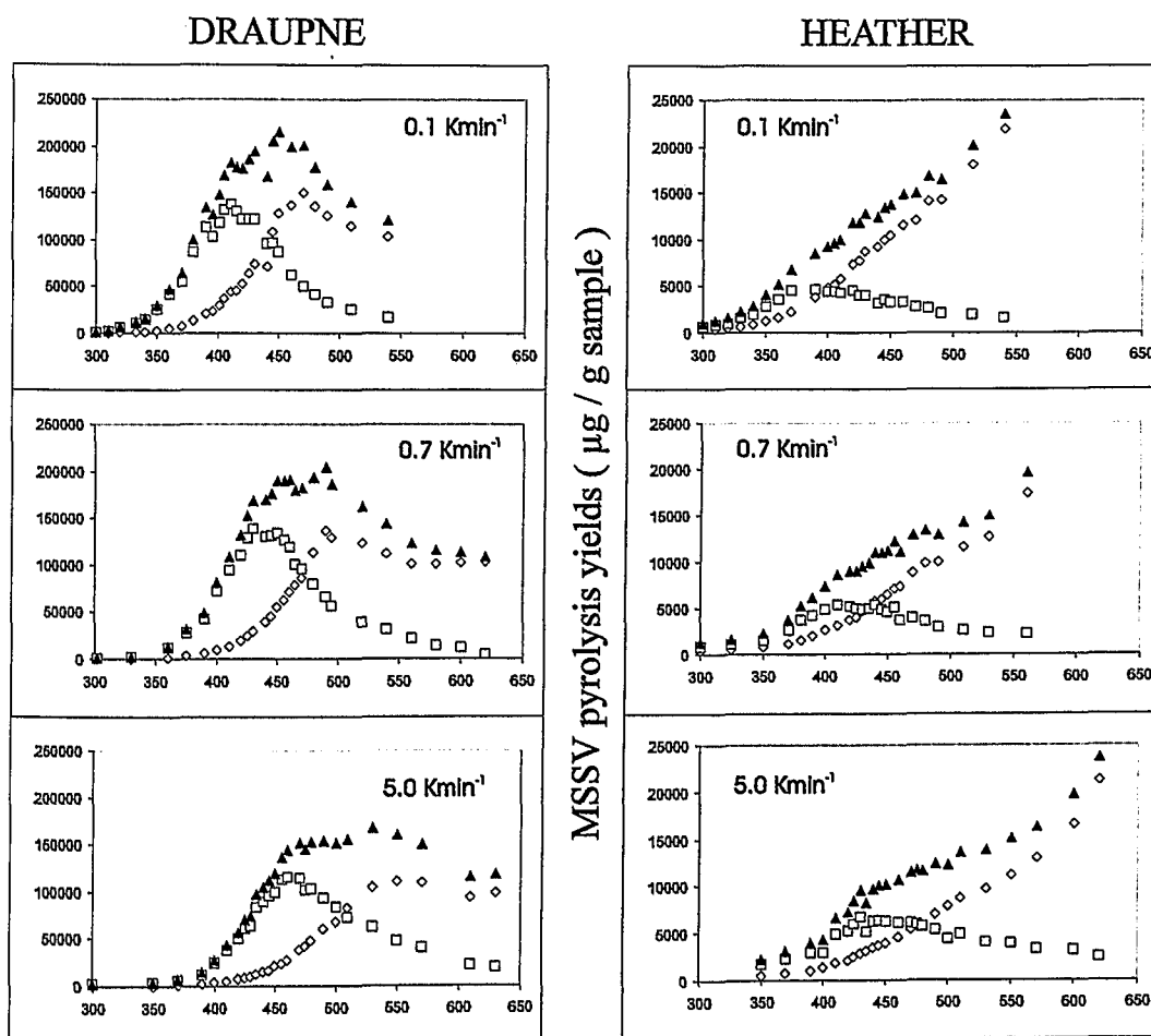
Fig. 14: MSSV pyrolysis total product and C_{1-5} and C_{6+} boiling range evolution at three heating rates, Heather and Draupne Formation (full triangles = C_{1+} , squares = C_{6+} and rhombuses = gas C_{1-5} ).
