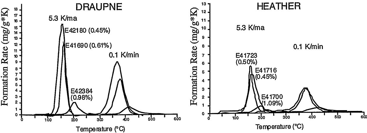
Fig. 12: Bulk hydrocarbon formation rate curves for samples of different degrees of natural maturation (vitrinite reflectance), Heather and Draupne Formation.
