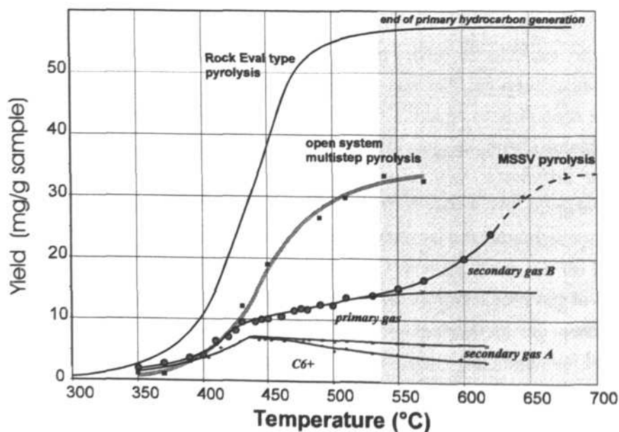
Fig. 27: Comparison of the results of Rock Eval type integrated total product generation, multistep open pyrolysis cumulative total product generation and closed system MSSV pyrolysis total product generation extended by questionmark to higher temperatures. The interpretation of the composition of MSSV pyrolysis products is discussed in the text. All data for a heating rate of 5.0 \text{ Kmin}^{-1} .
