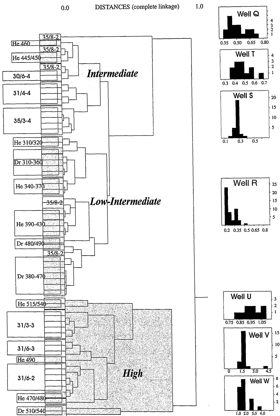
Fig. 71: Result of cluster analyses using headspace and occluded gas data from the eastern Viking Graben flank and experimental MSSV data sets (Heather and Draupne at 0.1 \text{ Kmin}^{-1} ). Input parameters are: \ln ([n-C_1]/[n-C_2]) , \ln ([n-C_2]/[n-C_3]) , \ln ([n-C_3]/[n-C_4]) . The independent i/n-butane distribution is depicted for comparison.
