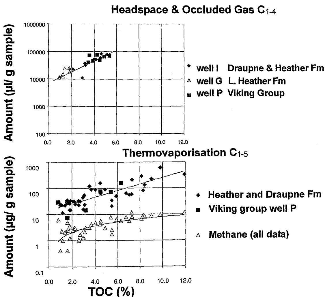
Fig. 58: Retention of gas as a function of TOC. Thermovaporisation and headspace gas data (note different scales).
