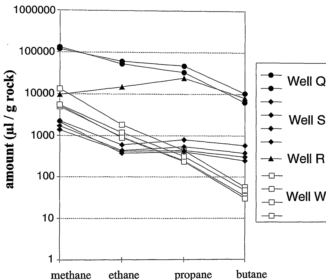
Fig. 72: Headspace and occluded gas compositions. Examples for natural gas compositional patterns. The wells depicted are also part of the cluster analyses in Fig. 71.
