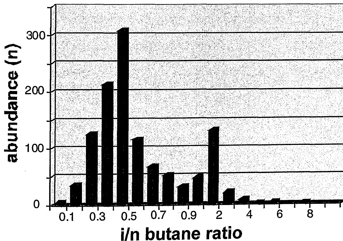
Fig. 68: Headspace and occluded gas data from Norwegian quadrants I, II, III and IV. (Norsk Hydro data base and Table 26).
