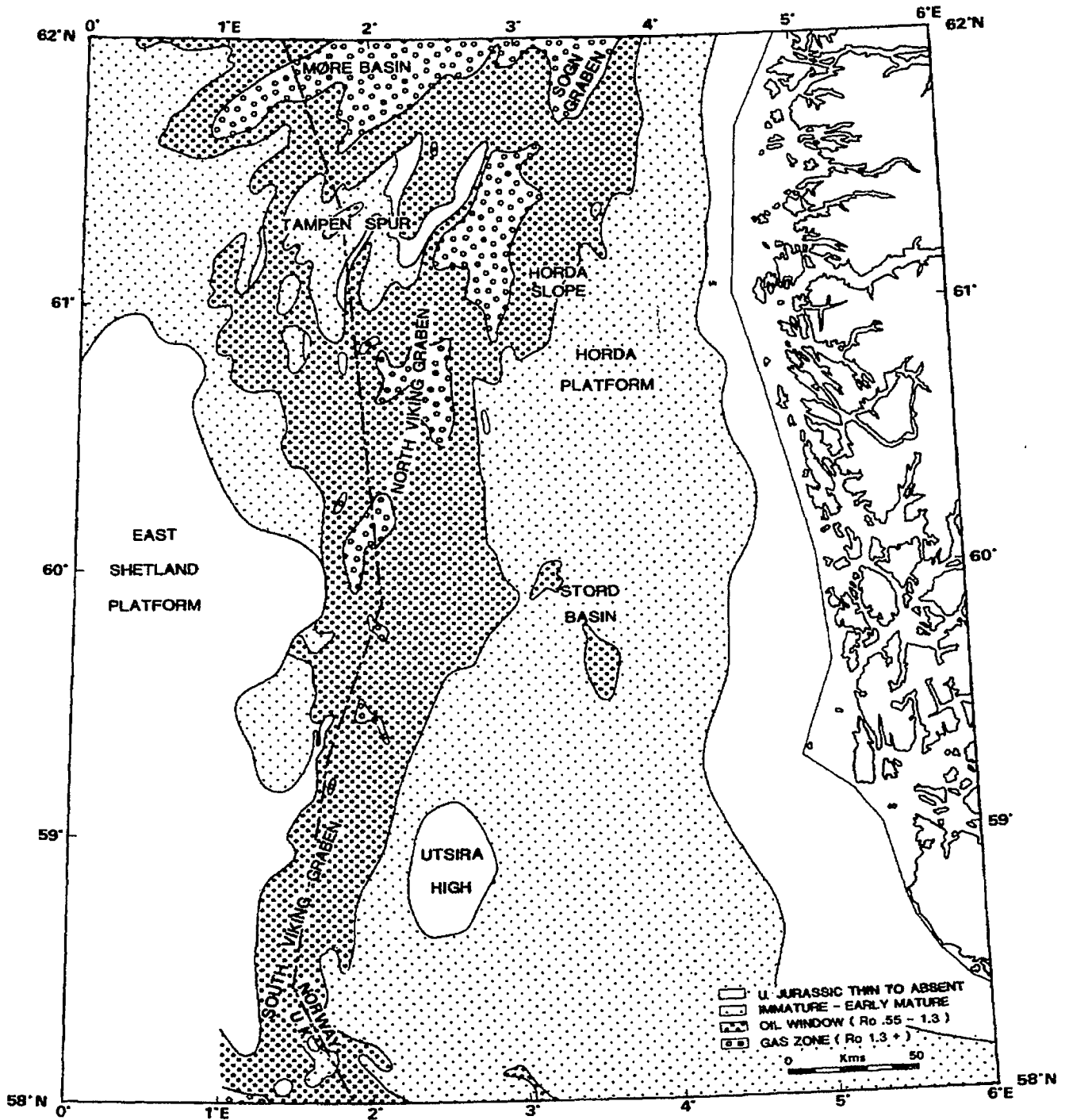
Fig. 1: Northern North Sea. Maturity expressed as vitrinite reflectance encountered in the Upper Jurassic. From Field (1985).
