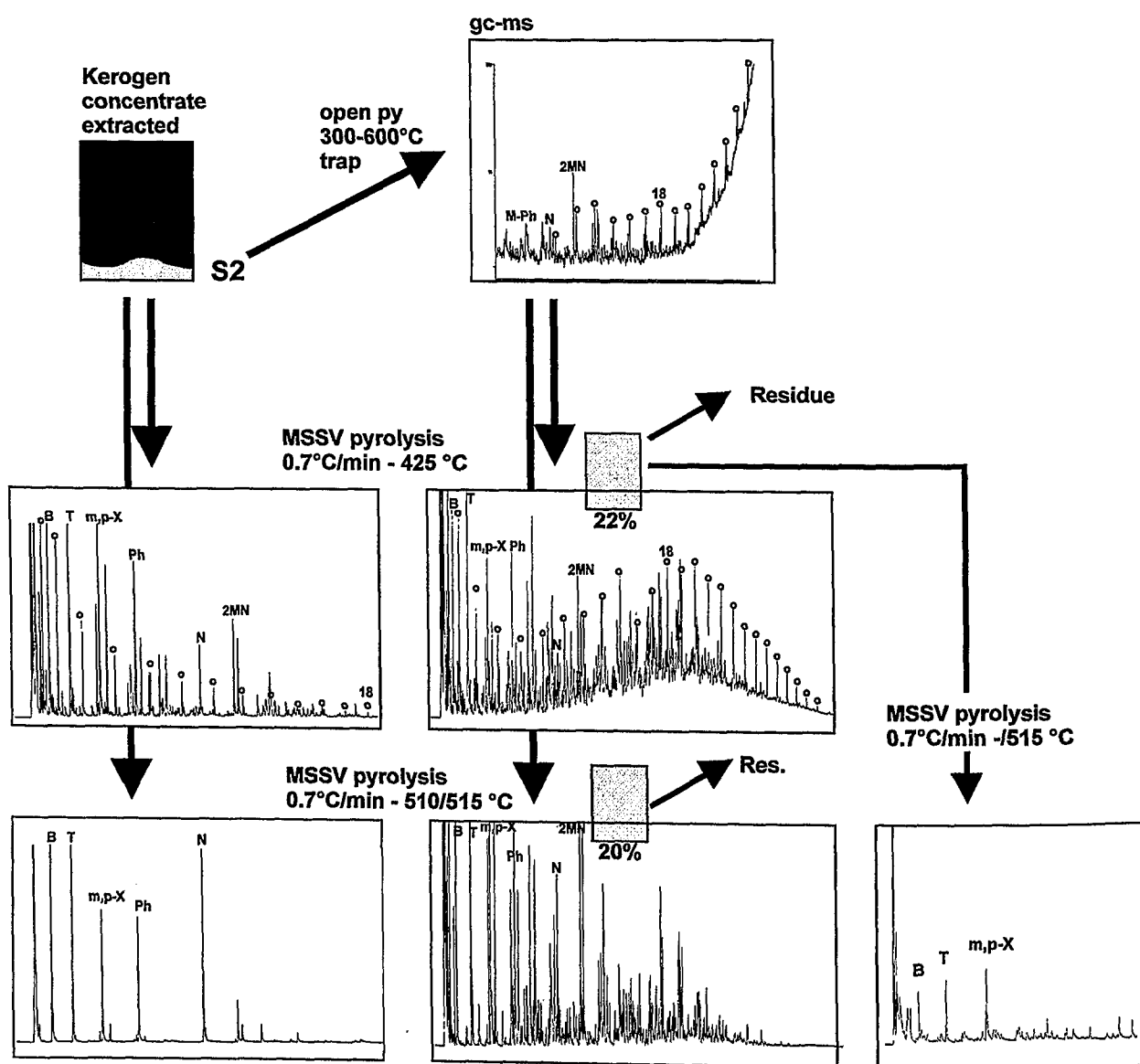
Fig. 32: Heather Formation (E 41716 MK EC), evolution of pyrolysis products from kerogen concentrate versus evolution from isolated Rock Eval S2. Implications for the composition of neoformed bitumen, and gas from cracking of this bitumen (bottom, right).
