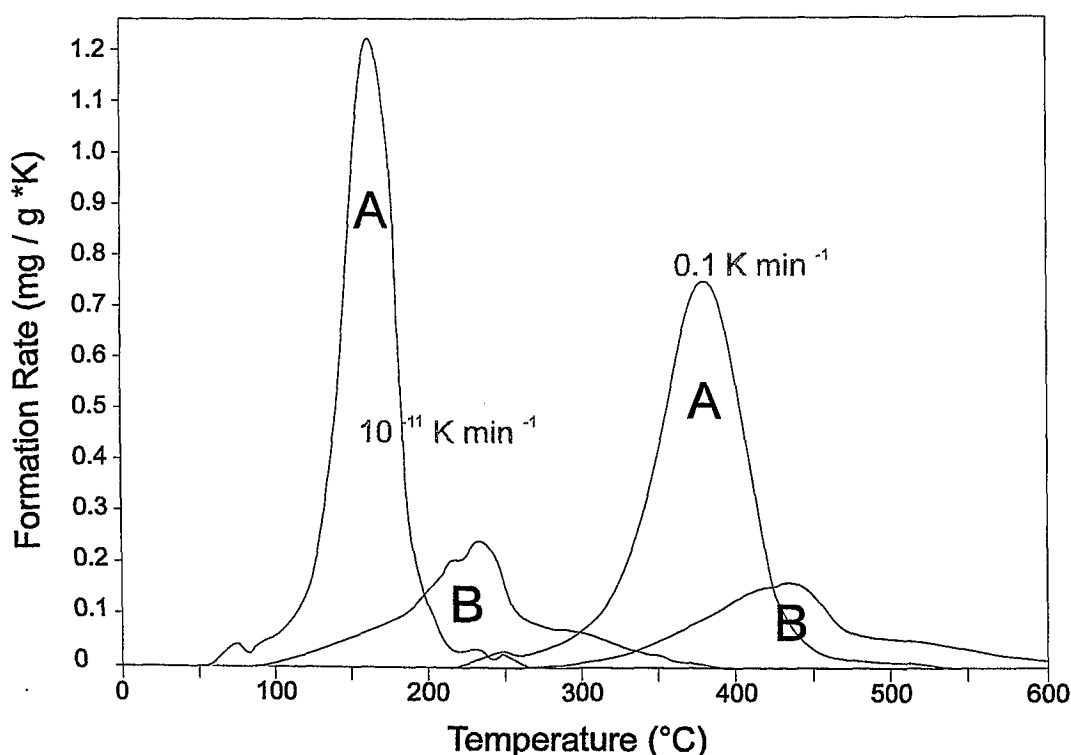
Fig. 30: Rock Eval type pyrolysis. Experimental ( 0.1 \text{ Kmin}^{-1} ) and extrapolated ( 10^{-11} \text{ Kmin}^{-1} ) product formation rates of the A immature ( R_o=0.45\% ) and an B artificially matured sample (MSSV pyrolysis 430^\circ\text{C} at 0.7 \text{ Kmin}^{-1} ).
