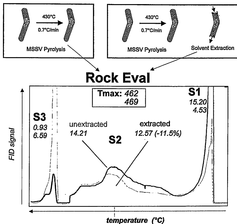
Fig. 29: Rock Eval screening analyses of an extracted and an unextracted aliquot of artificially matured ( 430^\circ\text{C} at 0.7 \text{ Kmin}^{-1} ) Heather Formation sample E 41716 MK EC.
