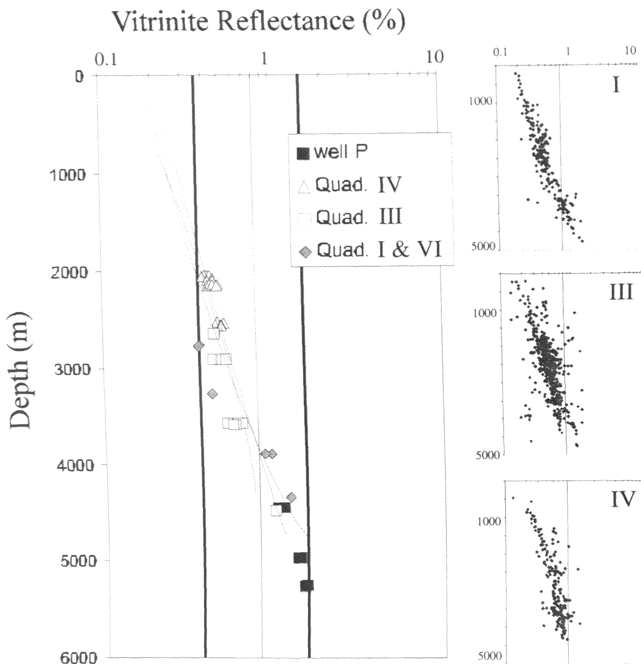
Fig. 8: Vitrinite reflectance ( R_o %) versus depth for the here investigated sample set (left) listed in Table 3. Mean trend-lines from diagrams on the right are included. Right: distributions of R_o (%) versus depth in the Norwegian Quadrants I, III and IV (Norsk Hydro data).
