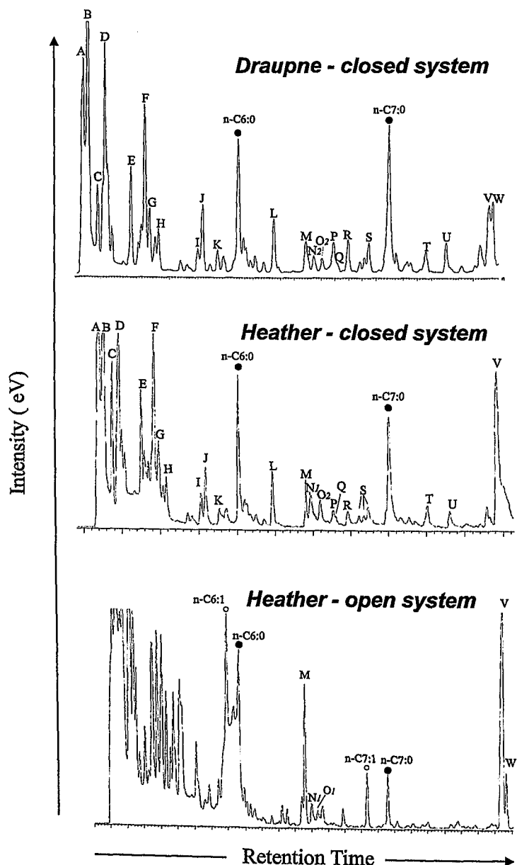
Fig. 16: Compositions in the light hydrocarbon range (Total ion-chromatogram TIC, ethane - toluene) for samples chosen for detailed investigations. Draupne Formation well B 2764.7m (E 43254 MK EC) and Heather Formation well G, 2138.75m (E41716 MK EC). For peak-key see Table 13 Pyrolysis conditions: MSSV closed system - 460^{\circ}\text{C} at 5.0 \text{ Kmin}^{-1} (Draupne) and 430^{\circ}\text{C} at 0.7 \text{ Kmin}^{-1} (Heather) and open system - 300\text{-}600^{\circ}\text{C} at 60 \text{ Kmin}^{-1} .
