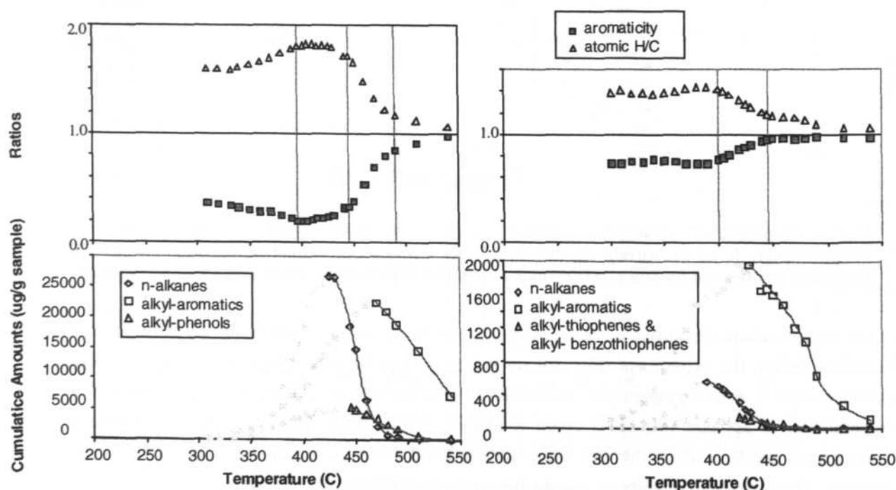
Fig. 51: MSSV pyrolysate (resolved fraction) compositional changes, Draupne Formation (left) and Heather Formation (right). All curves at 0.1 \text{ Kmin}^{-1} . H/C ratios are calculated as the sum of all component H/C ratios weighted by their abundance. Aromaticity was determined as: sum of identified aromatics / sum of resolved C_{6+} pyrolysate.
