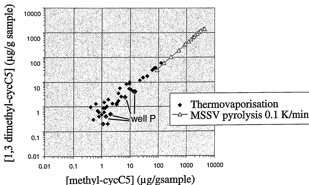
Fig. 60: Concentration-plot modified from Mango (1990) for MSSV pyrolysates of Draupne Formation well B (2764.7m) and all available thermovaporisation data (Table 3). For the case of MSSV pyrolysis only data prior to the onset of secondary cracking are included.
