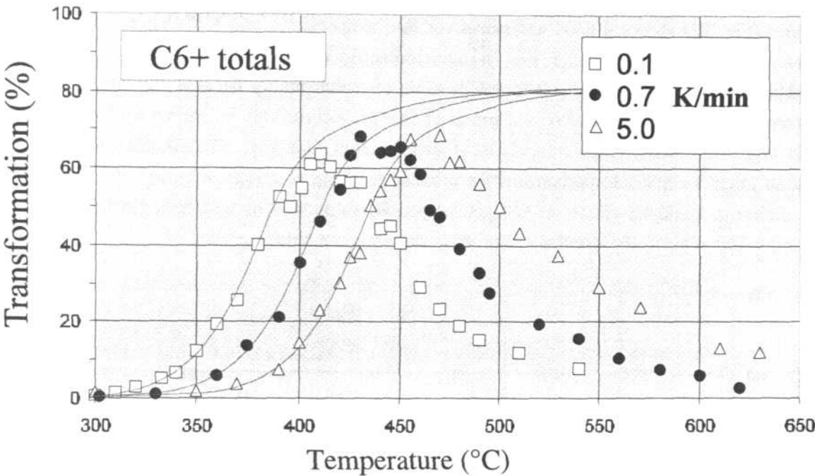
Fig. 20: MSSV pyrolysis C 6+ cumulative formation curves normalised to C 1+ total products. The curves are compared to the open system derived C 6+ curve determined at 5.0 Kmin -1 .
