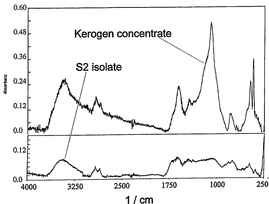
Fig. 31: IR spectroscopy of kerogen concentrate and isolated S2. Comparison of bands at 2900, 1443, 1378 and 780 (1/cm).
