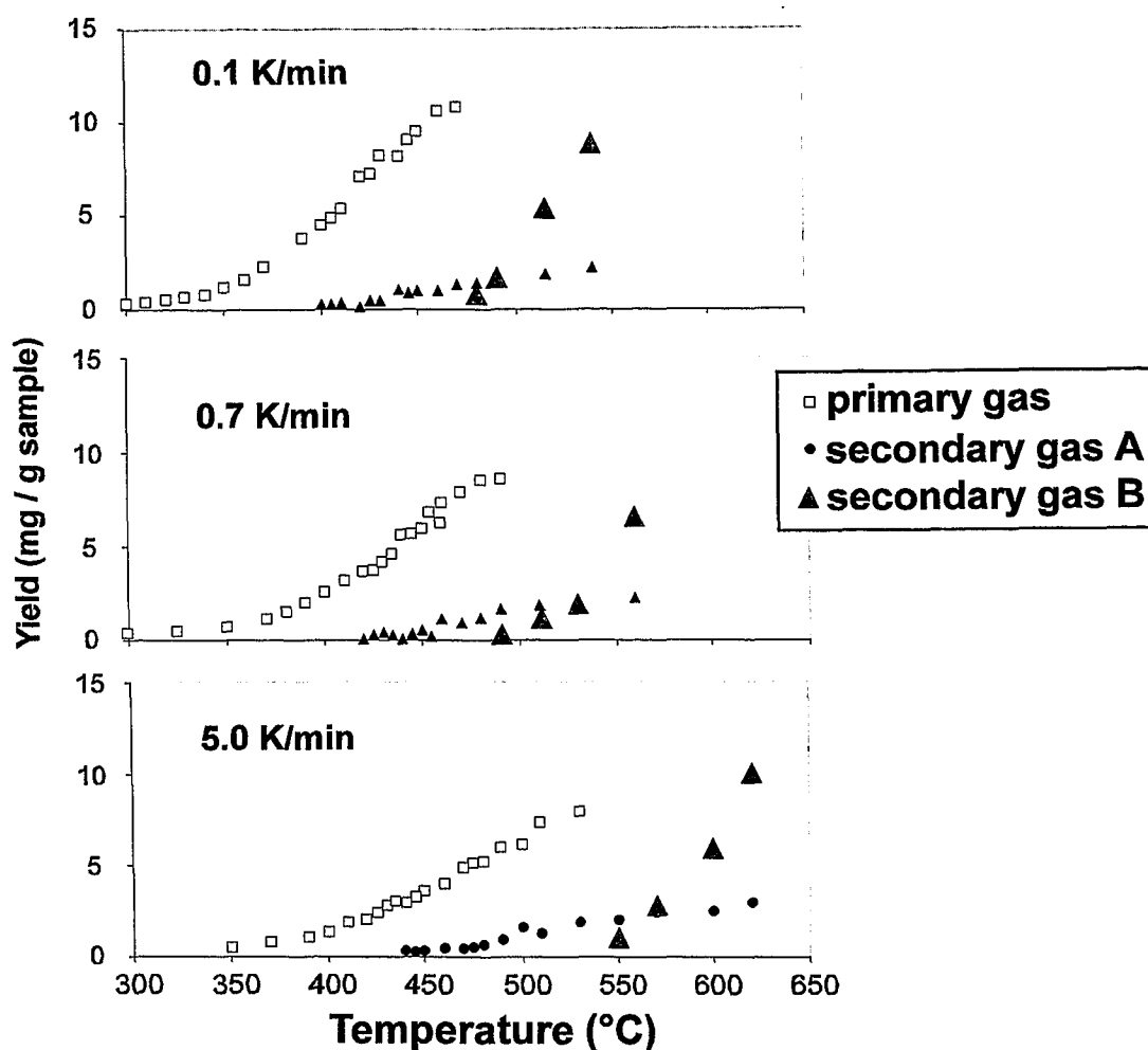
Fig. 28: MSSV pyrolysis. Calculated primary gas formation and two types of secondary gas formation, A = from total detected C_{6+} and B = from neo-formed residuum. Secondary gas A was calculated from the decrease of C_{6+} according to the equations 1-3. Secondary gas B is assumed to equal the gas formation above 550°C because primary production can be excluded.
