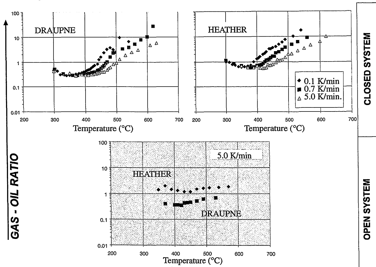
Fig. 57: GOR of products from artificial maturation of immature kerogens during closed (top) and open system pyrolysis (bottom).
