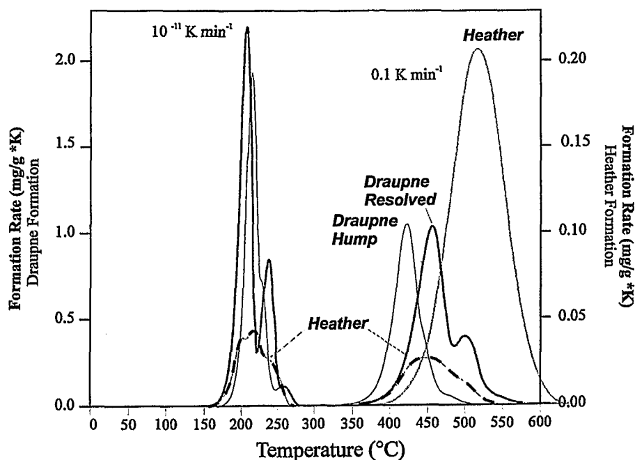
Fig. 38: Secondary gas from cracking of C_{6+} hump and C_{6+} resolved compounds, Draupne Formation and C_{6+} total Heather Formation. For secondary cracking of neoformed bitumen a formation rate curve for laboratory conditions was constructed (see text). Left, predicted rate curves at a geological heating rate and right, measured rate curves at an experimental heating rate.
