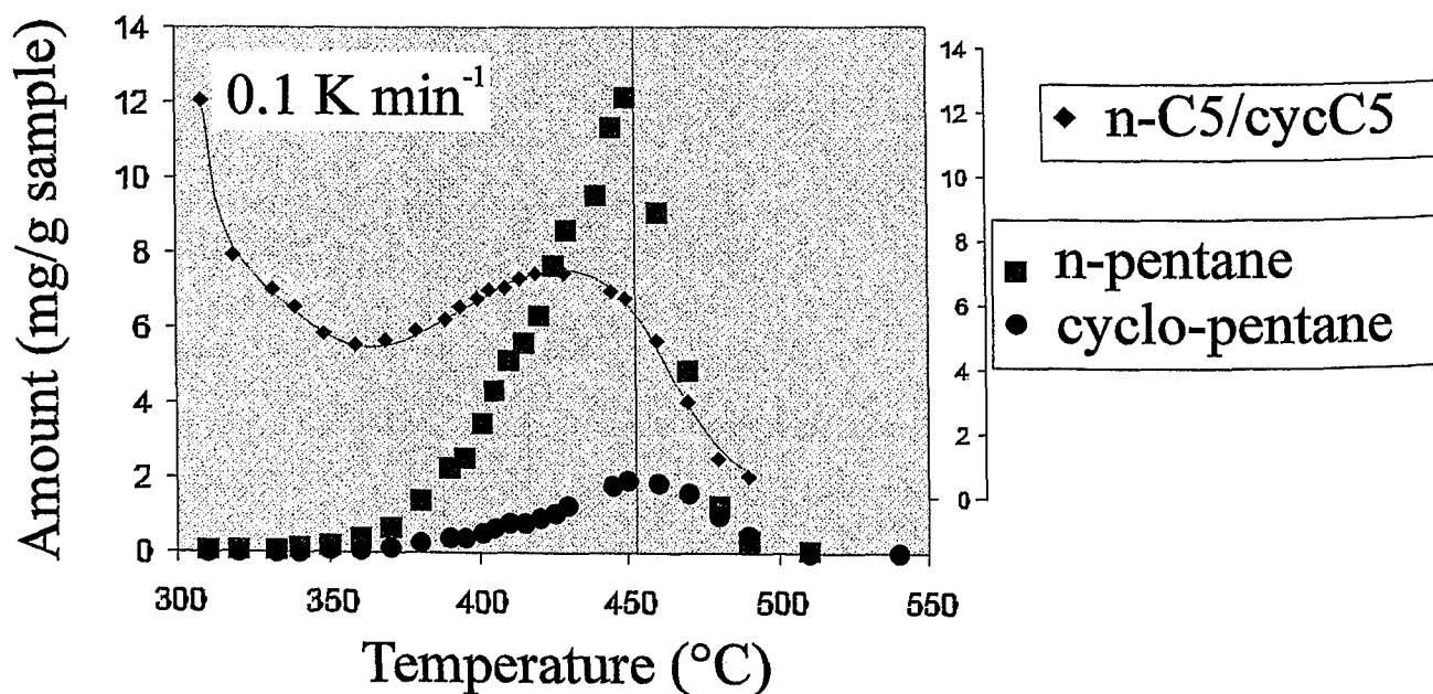
Fig. 61: N-C5 and cyc-C5 as a function of MSSV pyrolysis temperature (left scale) for Draupne Formation sample from well B (2764.7m) and their respective paraffinicity ratio (right scale).
