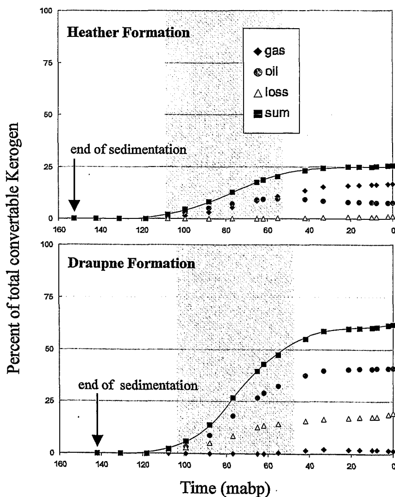
Fig. 47: Petroleum product balancing taking account for the complete section (100%). Kerogen conversion is by far more complete for Draupne Formation. Heather Formation shows oil to gas cracking, but the contribution of high maturity methane seems to be still negligible.
