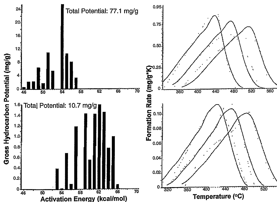
Fig. 33: Measured and calculated formation rate curves for primary gas generation at heating rates of 0.1, 0.7 and 5.0 \text{Kmin}^{-1} (right) and kinetic parameters for Draupne Formation (top) and Heather Formation (bottom) . Potentials are in mg per g sample.
