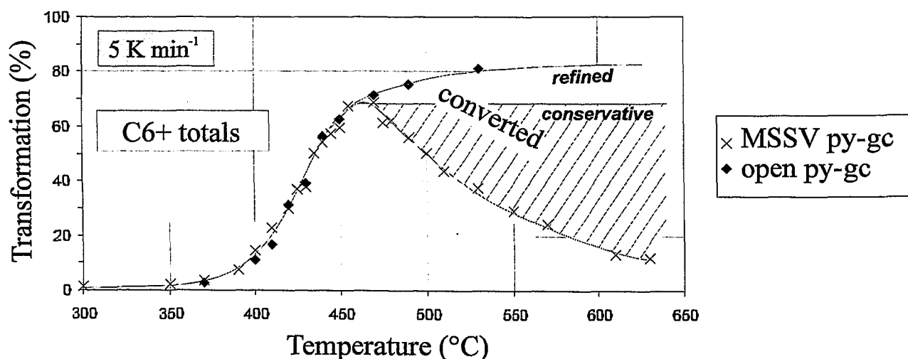
Fig. 19: Comparison of open and closed system C_{6+} temperature versus transformation curves. Transformation is calibrated using the C_{1+} total product yields maximum. The onset of secondary cracking occurs before primary generation ends. Two different scenarios for the amount of educts for secondary gas generation are displayed.
