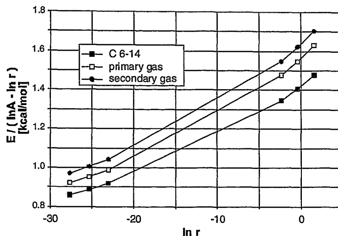
Fig. 37: T_{\max} as an expression of kinetic parameters and heating rate. T_{\max} measures for C_{6-14} , primary gas and secondary gas ( C_{6+} decrease) from Heather Formation.
