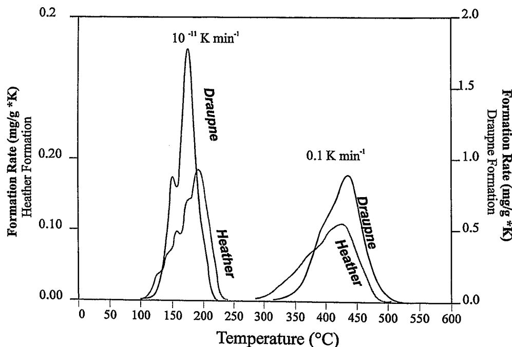
Fig. 34: Primary gas C_{1-5} formation rate curves for Heather and Draupne Formation. Slowest laboratory heating rate and extrapolation to a geologically reasonable heating rate. Note different scales for Heather and Draupne.
