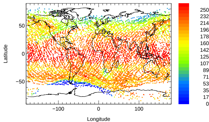
Fig. 1. CRISTA observations of \text{N}_2\text{O} between 4 November 1994, 21:00 UT and 6 November 1994, 12:00 UT at \Theta=700\pm 50 K transformed to a synoptic time by trajectory calculations.
