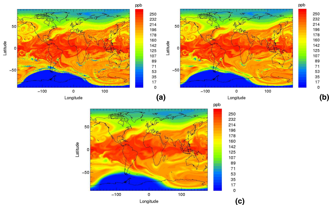
Fig. 5. CLaMS simulations with different mixing intensities for the 6 November 1994 initialised on 20 October 1994 with PV/N 2 O correlation ( \Theta=675 K) derived from the CRISTA observations. In-situ optimised mixing ((a), case B), satellite optimised mixing ((b), case C) and enhanced mixing ((c), case D).
