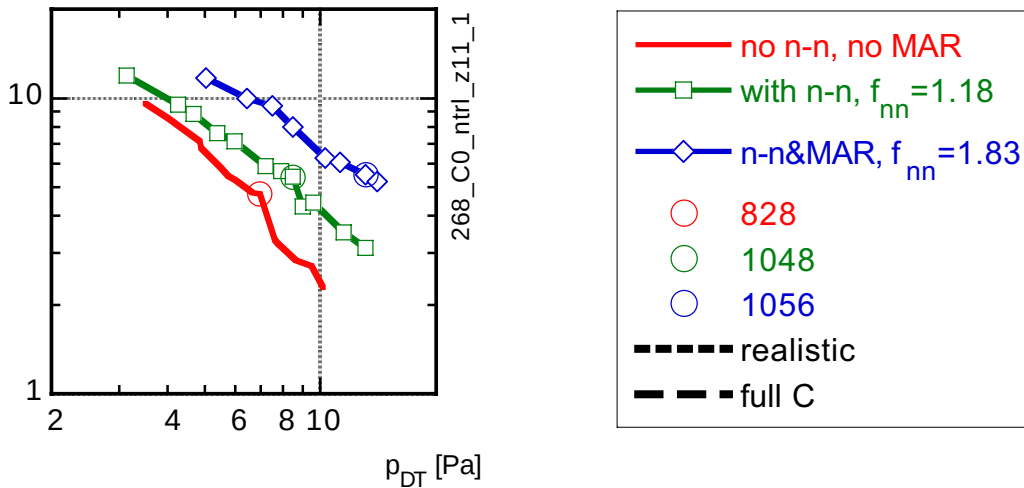
Fig. 3. Variation of the peak power loading of the target with the neutral pressure in the PFR for different assumptions on the neutral transport. Cases near or at the transition points for each series (cases 828, 1048, and 1056) are circled. The same legend applies to Figs. 4, 5, and 8–13. In the legend for the scalings, “realistic” refers to realistic surfaces, and “full C” to full carbon walls [5].
