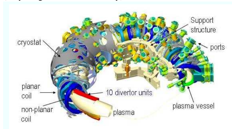
Fig. 1. Components of Wendelstein 7-X.
