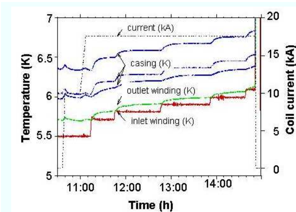
Fig. 3. Temperature and current signals during current quench test.
