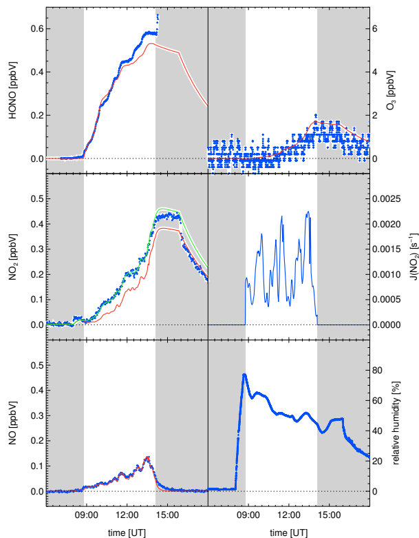
Fig. 2. HONO, NO x , and ozone formation in SAPHIR illuminated with sunlight using an additional filter foil in the presence of 550 ppmV of CO on 2 July 2002 (experiment type D, see Table 2). Blue symbols mark observations, red and green lines show the result of model calculations (see text).
