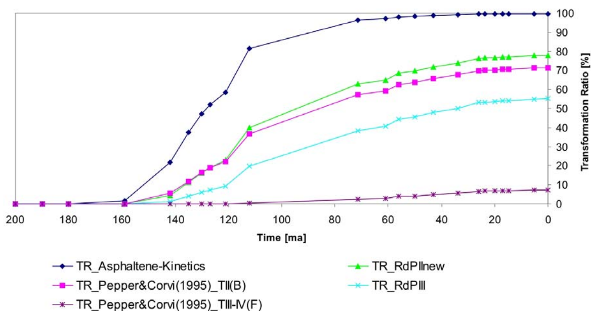
Figure 4-34: Transformation ratios of used kinetics for the Upper Jurassic source rock for the central part of the Porcupine Basin, profile MS81RE-94
