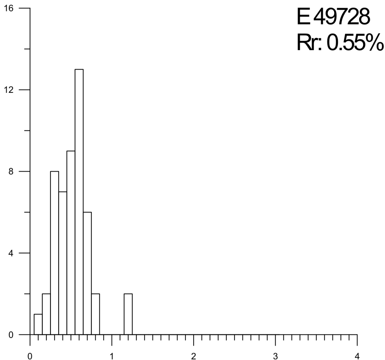
Figure 4-24: Histogram for the vitrinite reflectance for Jurassic sample 49728
