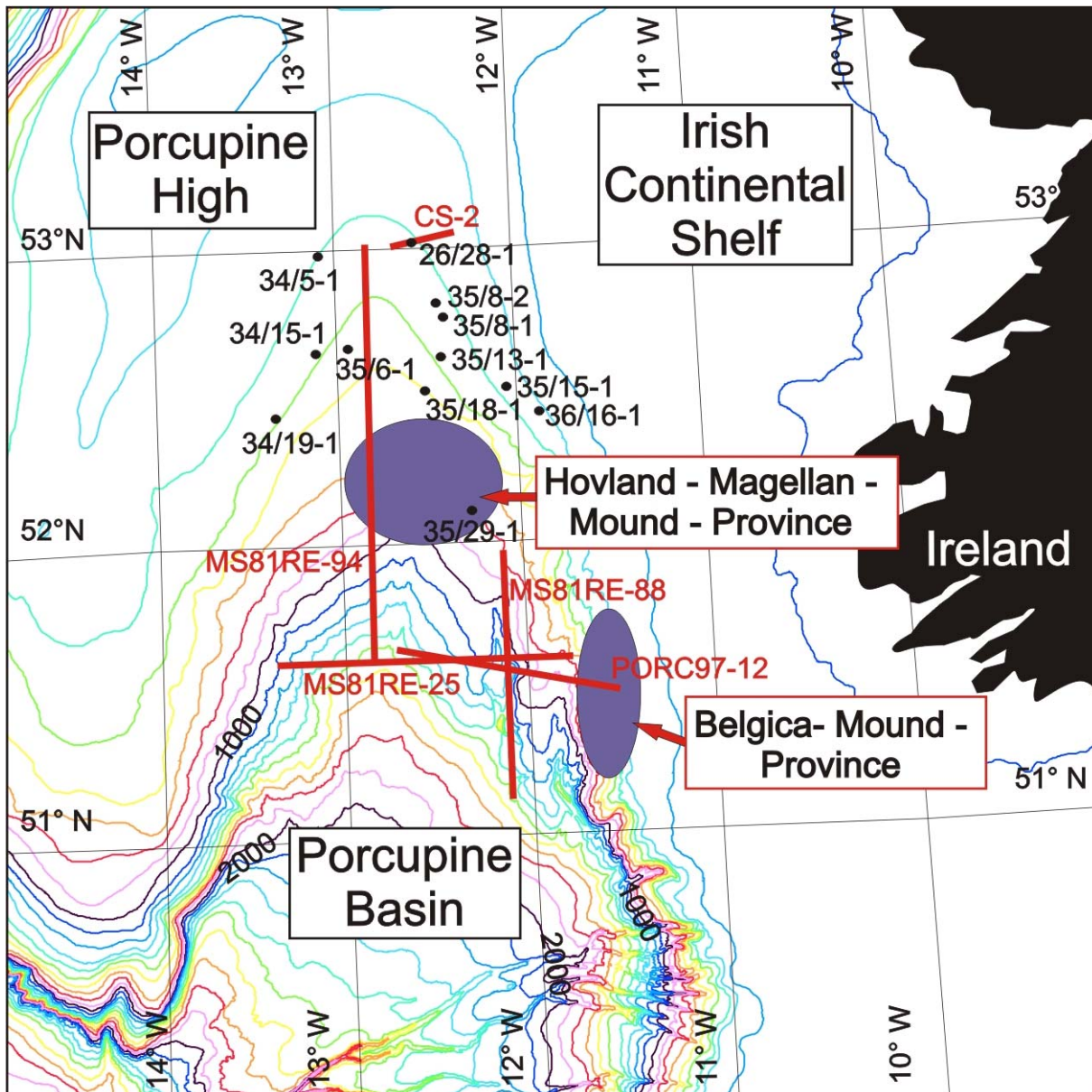
Figure 2-1: The Porcupine Basin including the location of mound provinces, wells and seismic lines; bathymetric contours are in 100 m intervals
