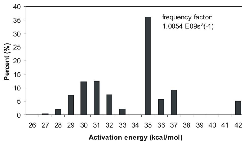
Figure 4-31: Distribution of asphaltene fraction for sample E49854
