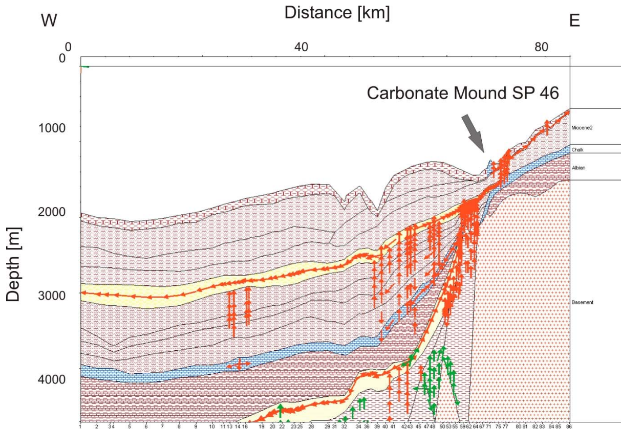
Figure 4-42: Modelled gas (red vectors) and oil (green vectors) migration along Aptian and Miocene sand layers (yellow) on profile PORC97-12 towards the carbonate mound SP46
