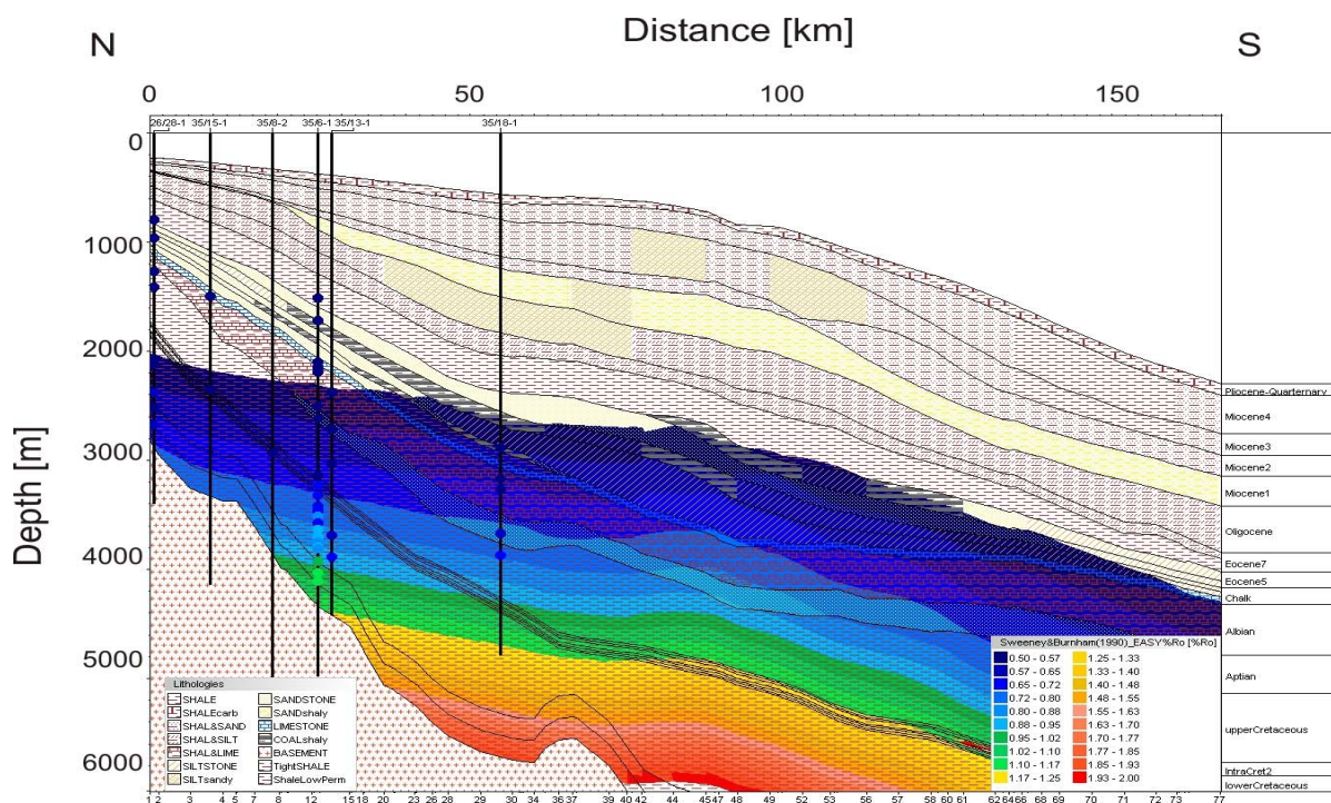
Figure 4-9: Line RE94 with calibration wells and Easy Rr overlay
