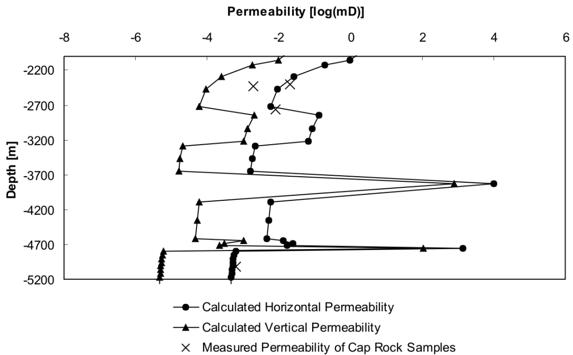
Figure 4-4: Modelled and measured permeability
