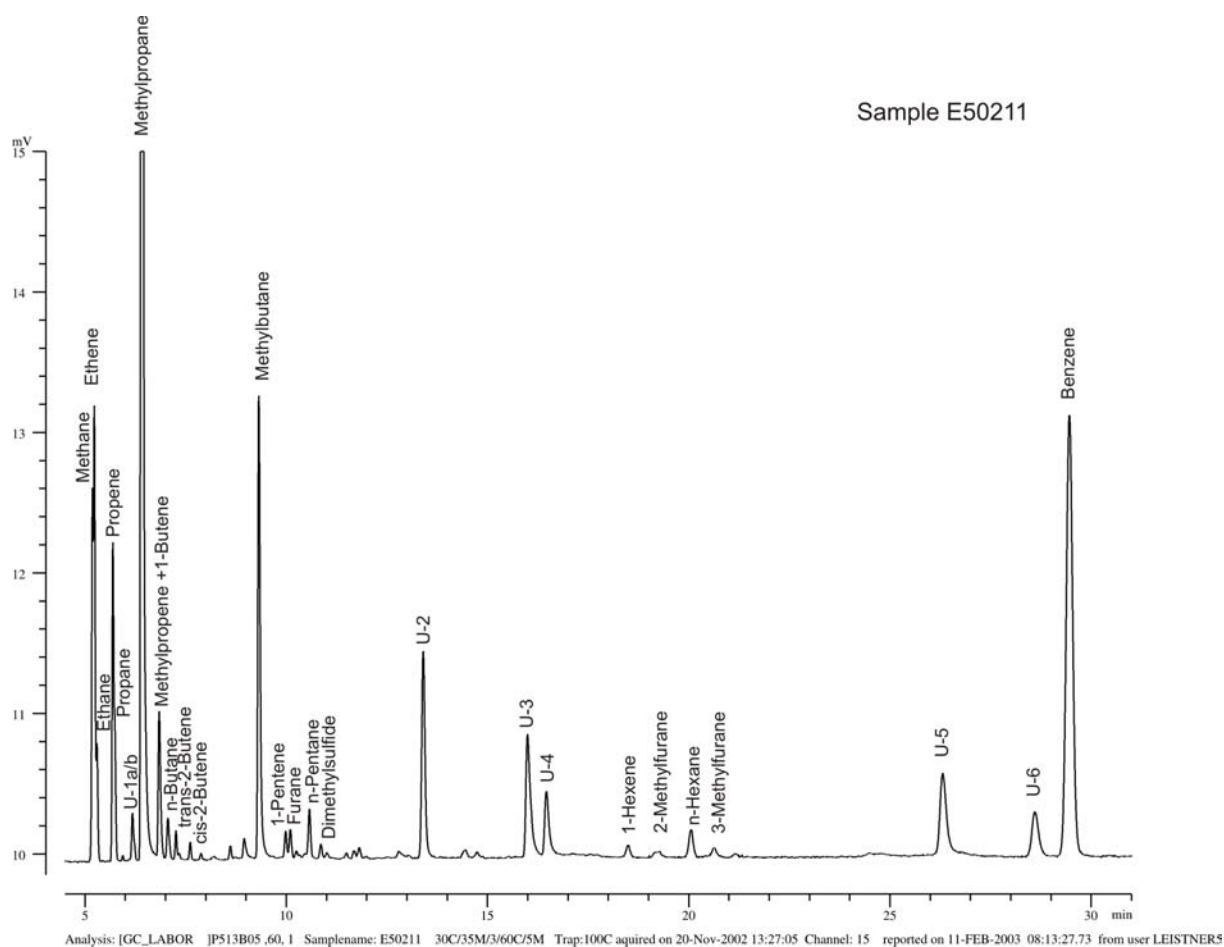
Figure 5-4: Gas chromatogram of sample E50211 from the Belgica mound province with identified peaks
