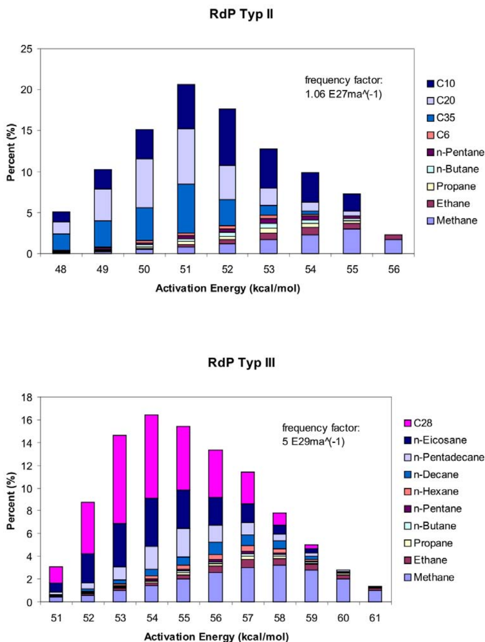
Figure 4-33: Kinetic data for the RdP kinetics
