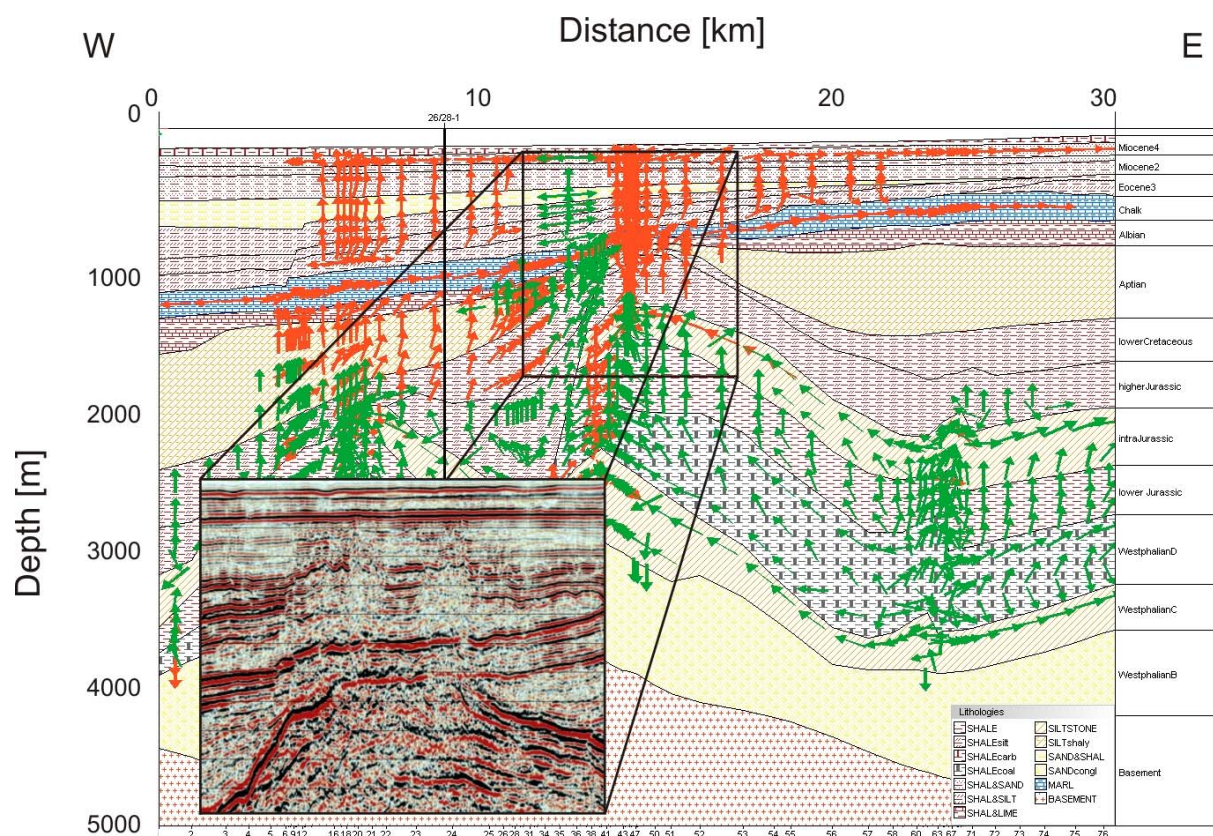
Figure 4-44: Profile CS2 through the Connemara field showing well 26/28-1 and modelled gas (red vectors) and oil (green vectors) flow as well as the gas chimneys and pockmarks observed in the seismics
