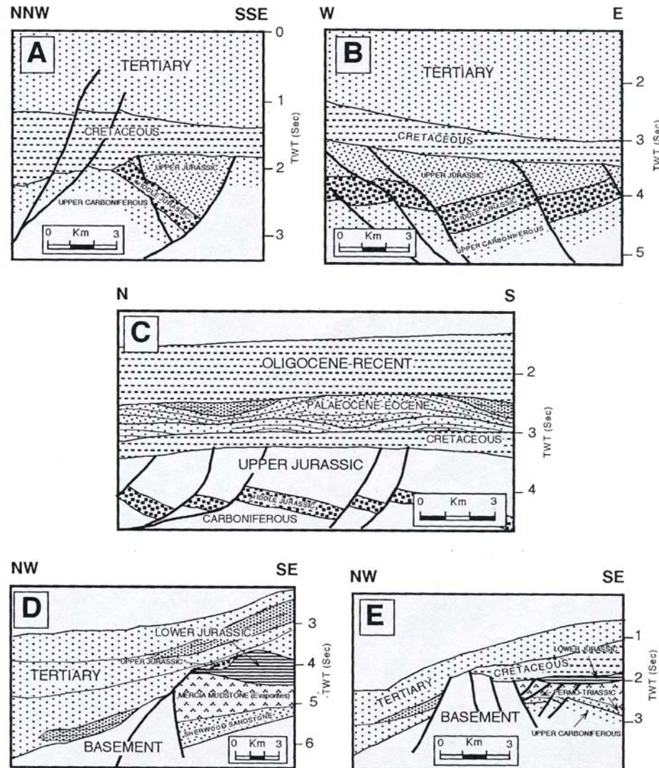
Figure 2-6: Play types with A: rotated and tilted fault blocks, B: basin edge tilted fault blocks, C: deltaic stratigraphic traps, D: stratigraphic traps adjacent to Basement and E: stratigraphic traps on basement horsts (Crocker et Shannon, 1995)
