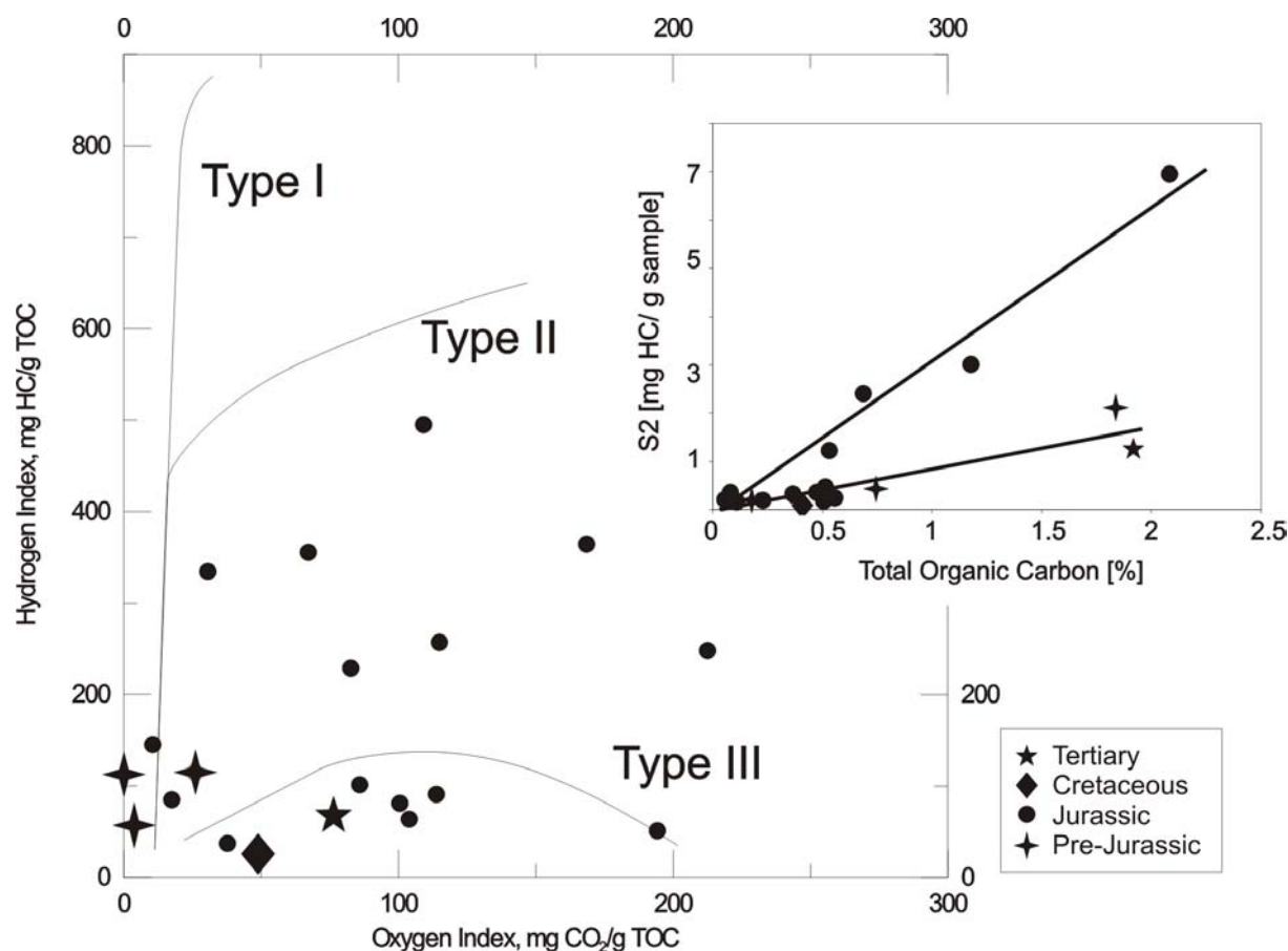
Figure 4-26: Kerogen type discrimination on the basis of Rock Eval parameters Hydrogen Index (HI) and Oxygen Index (OI), S2 and TOC
