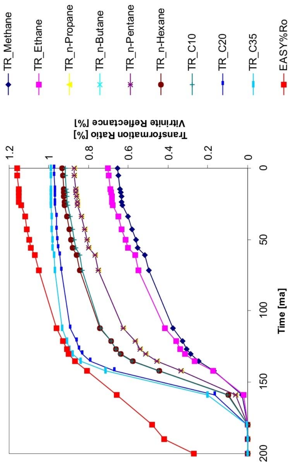
Figure 4-35: Transformation ratios of single compounds of the RdPII kinetic and calculated vitrinite reflectance for the Upper Jurassic source rock in vicinity of the Connemara area calculated of line CS-2
