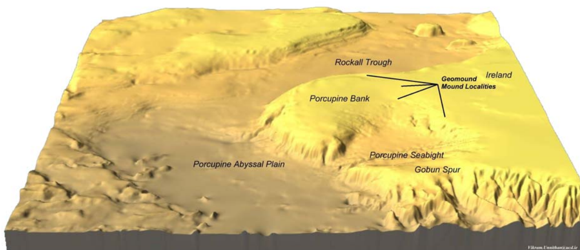
Figure 1-7: Porcupine Basin located offshore Ireland in the Atlantic Ocean including mound areas (Unnithan, 2000)
