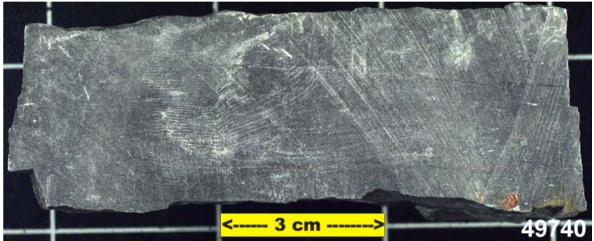
Figure 4-21: Cretaceous samples 49740
