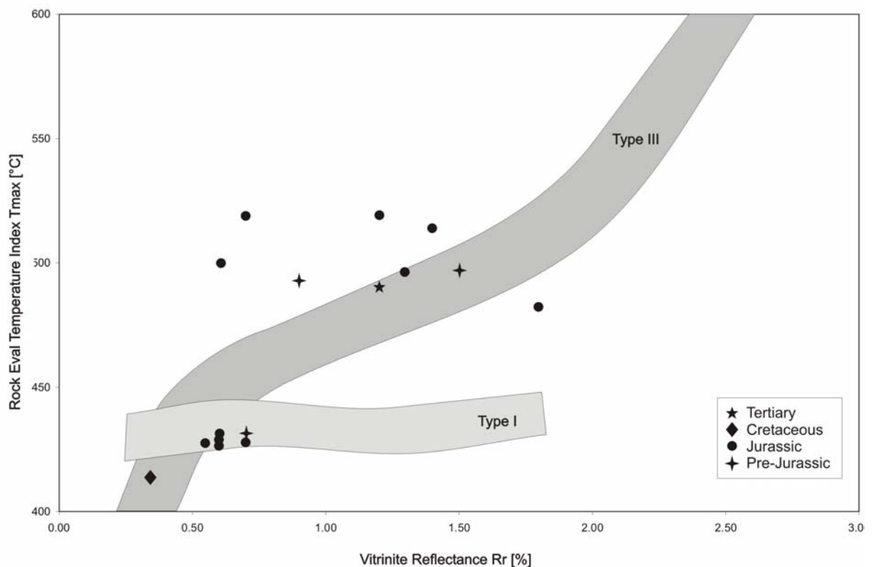
Figure 4-25: Relationship between the temperature index Tmax and the vitrinite reflectance after Tissot et al. (1987)
