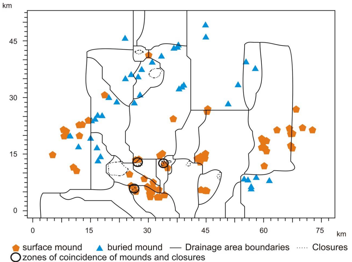
Figure 4-50: Results from the drainage area analysis for the C30 – map
