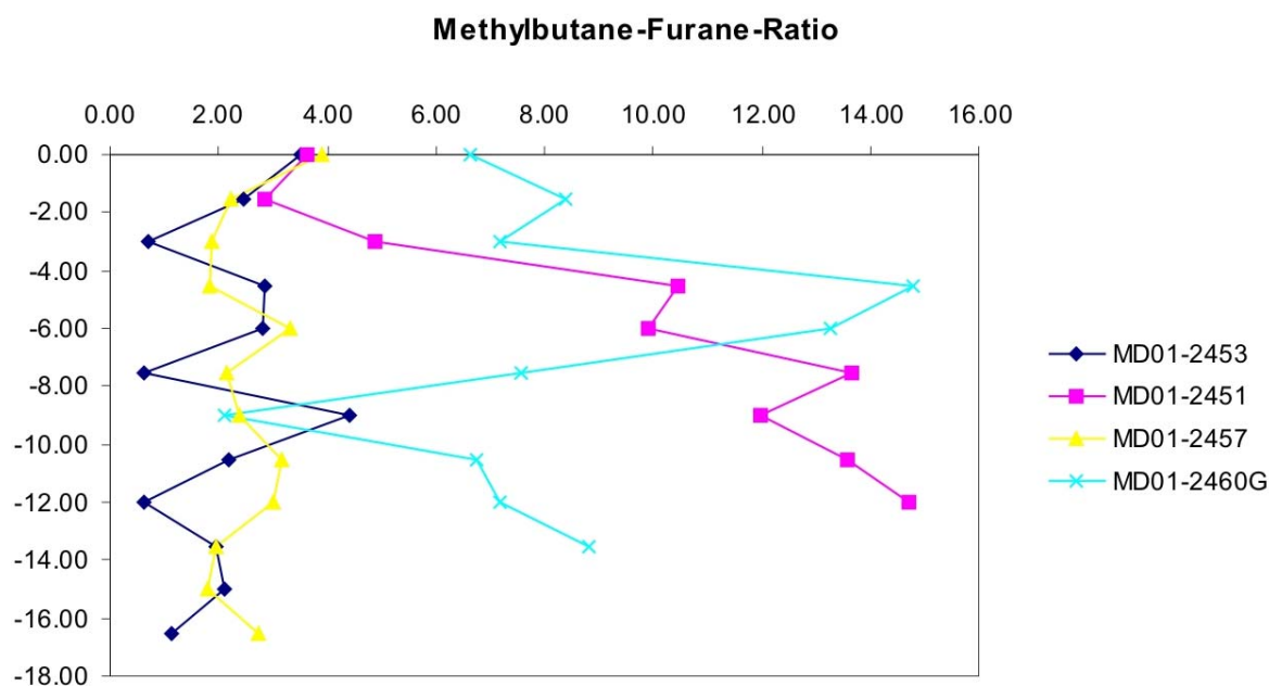
Figure 5-9: Methylbutane-Furane-Ratio
