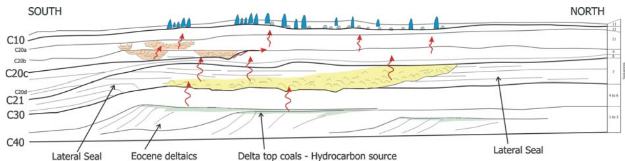
Figure 4-46: Model for hydrocarbon migration through the Cenozoic section (McDonnell, 2001)
