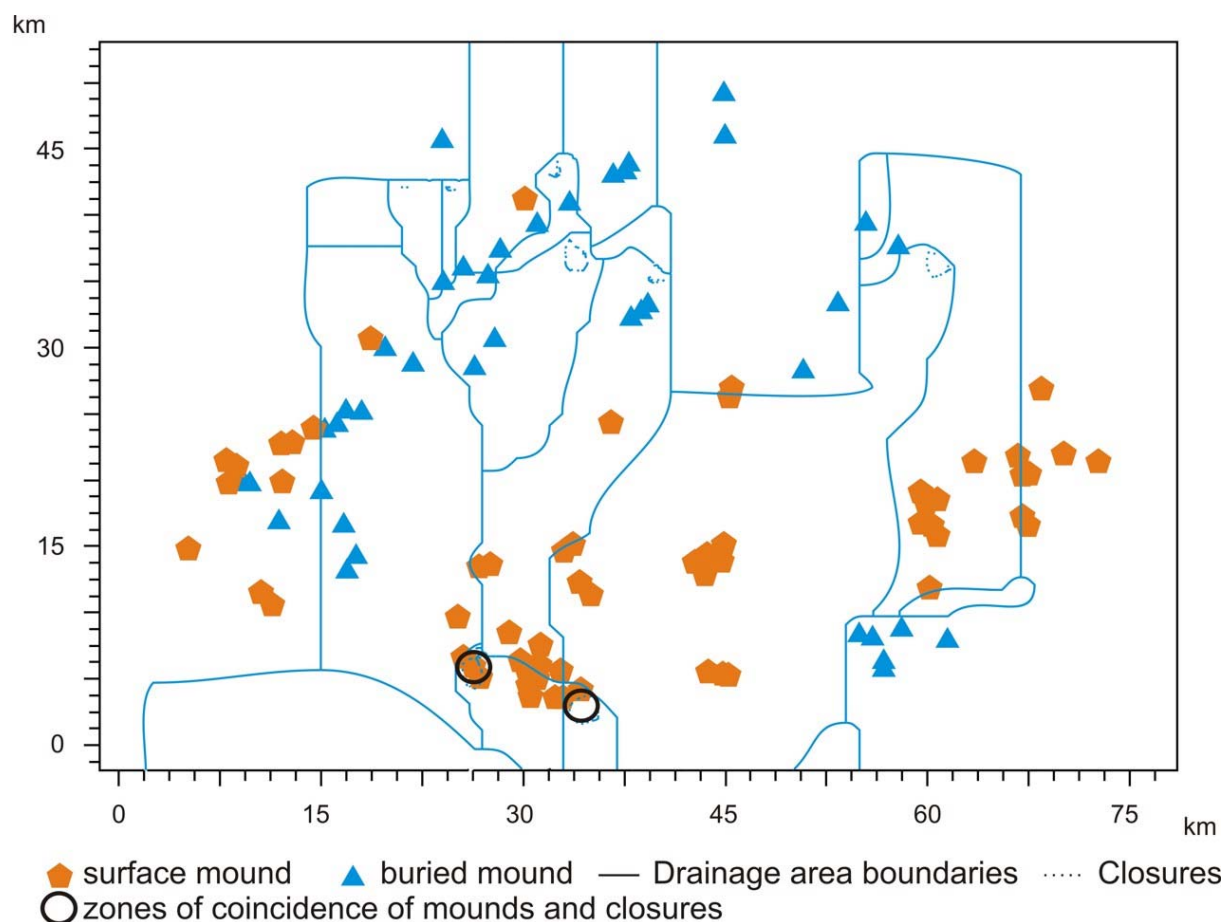
Figure 4-51: Results from the drainage area analysis for the Base-Miocene – map
