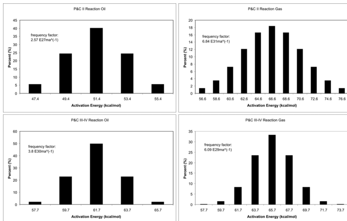
Figure 4-32: Kinetic data set for oil and gas of kerogen type II and III-IV (Pepper and Dodd, 1995)
