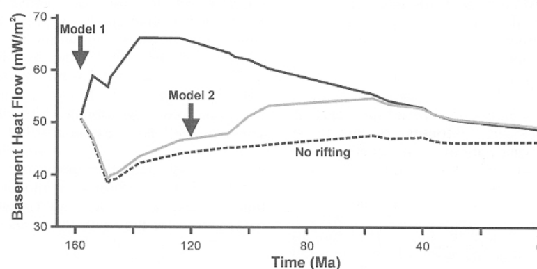
Figure 4-15: Heat flow models used by Baxter et al. (2001)
