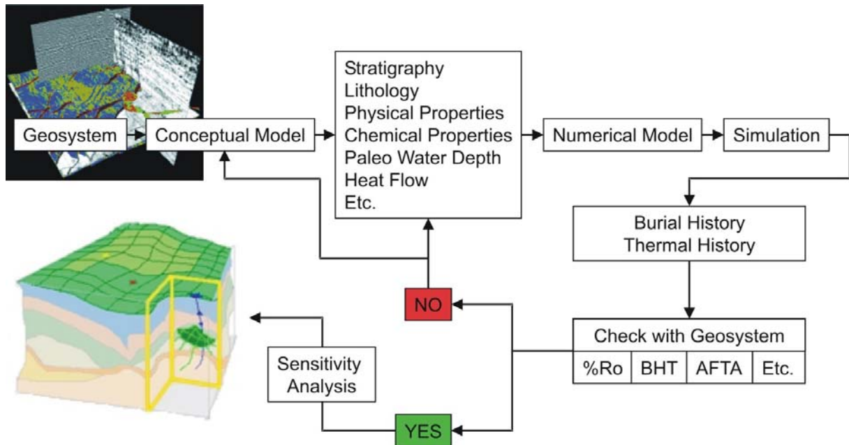
Figure 3-1: Principles of numerical simulation
