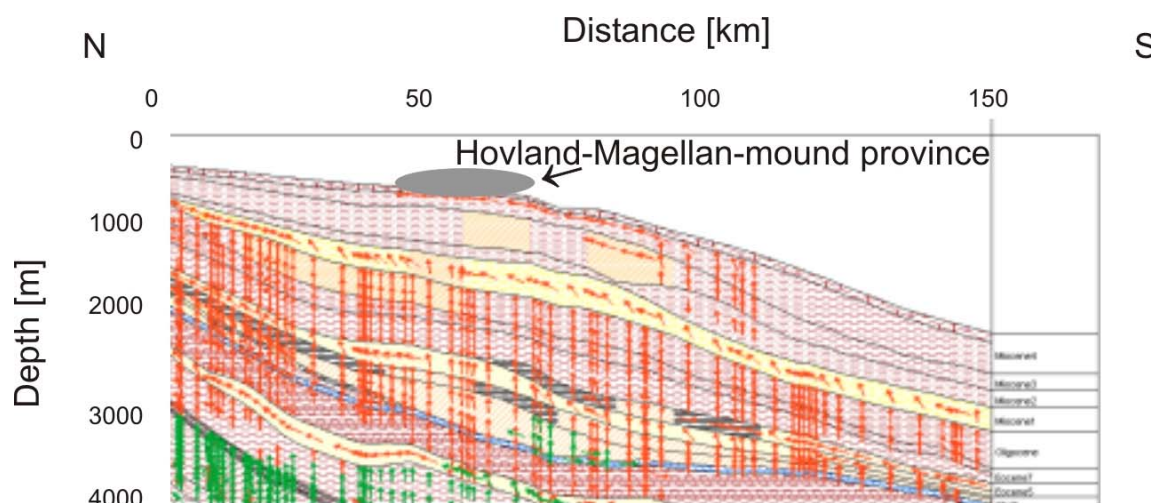
Figure 4-47: Gas migration towards the Hovland-Magellan mound province with no significant flow through the high permeable contourite deposits (light brown) after the model from McDonnell (2001)
