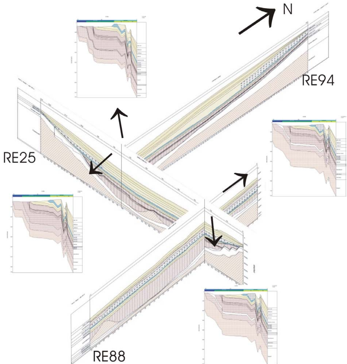
Figure 4-1: Basin geometry at intersection of the seismic lines
