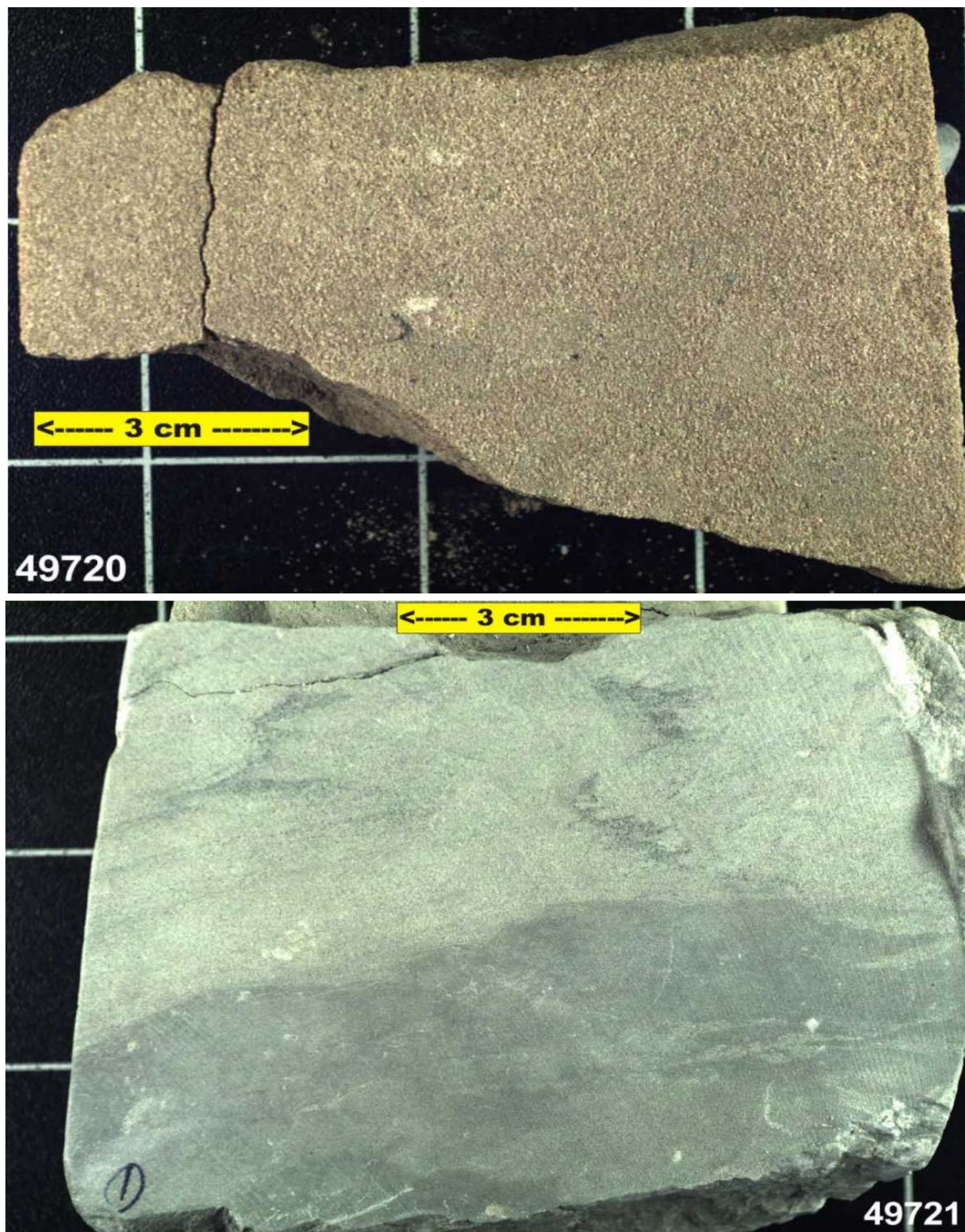
Figure 4-20: Upper Jurassic samples 49720 and 49721
