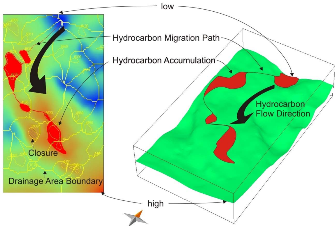
Figure 4-48: Theoretical background of drainage area modelling showing a map in 3D-view with hydrocarbon migration pathways and accumulations on the right. On the left a map view including migration pathways, accumulations and drainage area boundaries and closures
