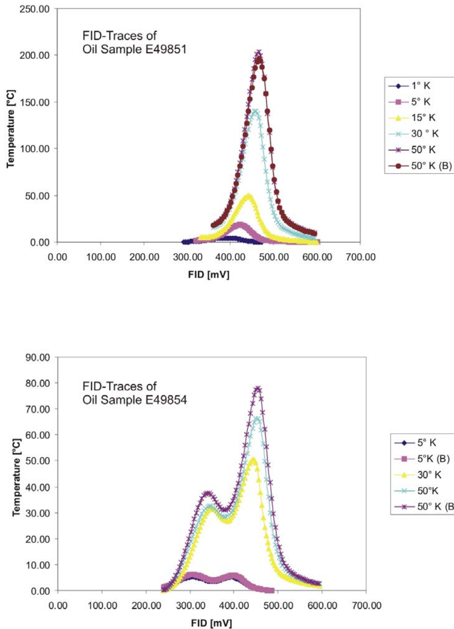
Figure 4-28: Original FID-traces
