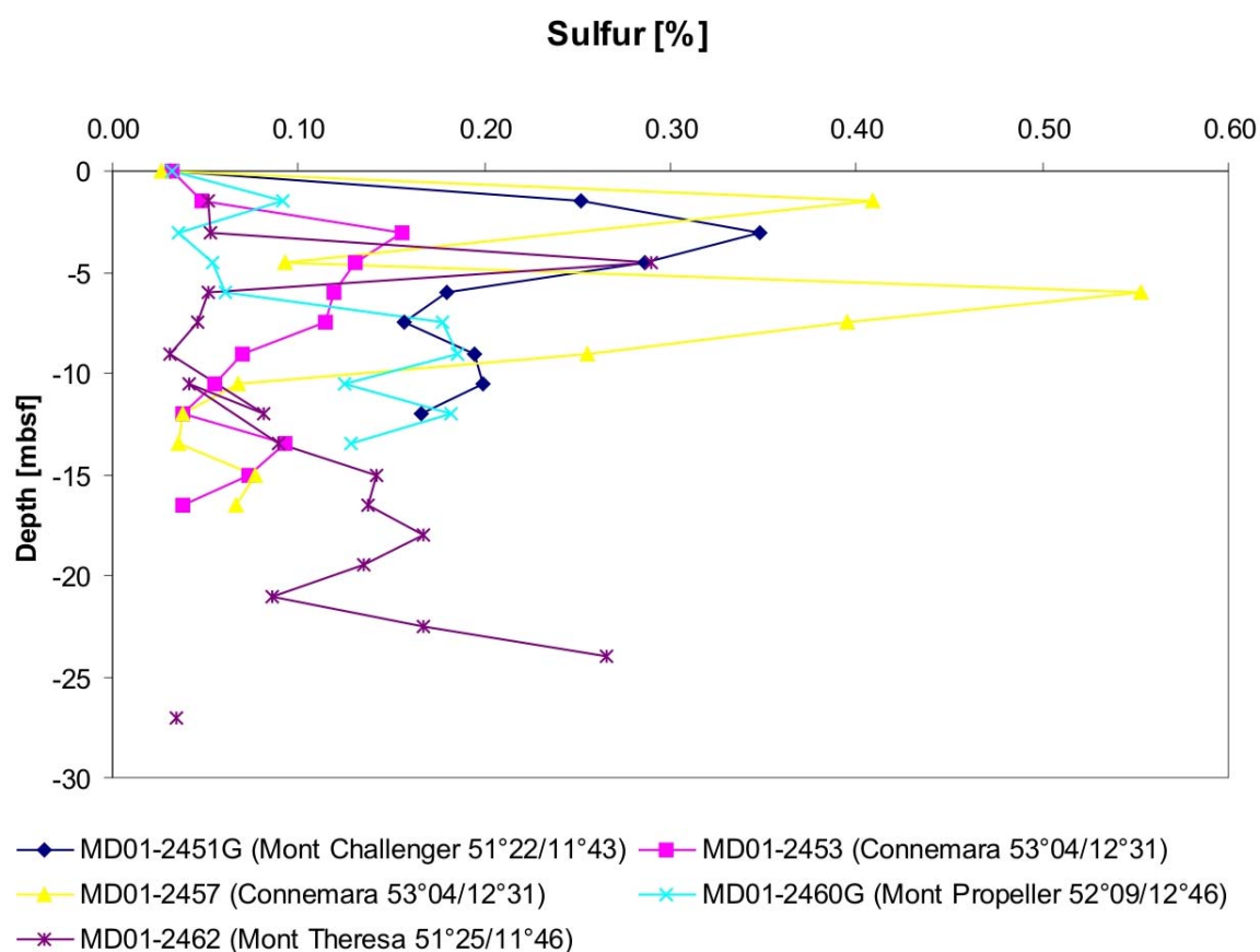
Figure 5-2: Sulfur content plotted versus depth for the cores MD01-2451G, MD01-2453, MD01-2457, MD01-2460G and MD01-2462
