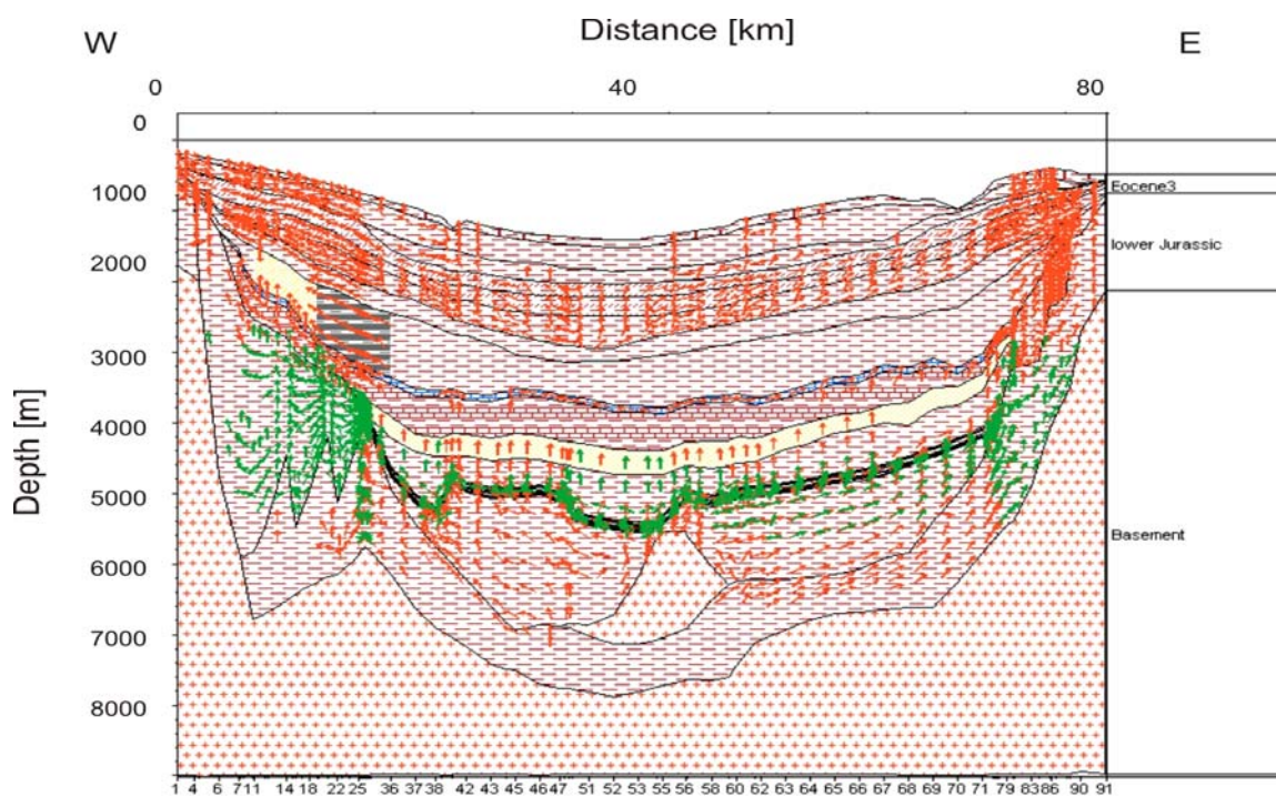
Figure 4-38: Present day configuration of modelled gas (red vectors) and oil (green vectors) flow along profile RE25
