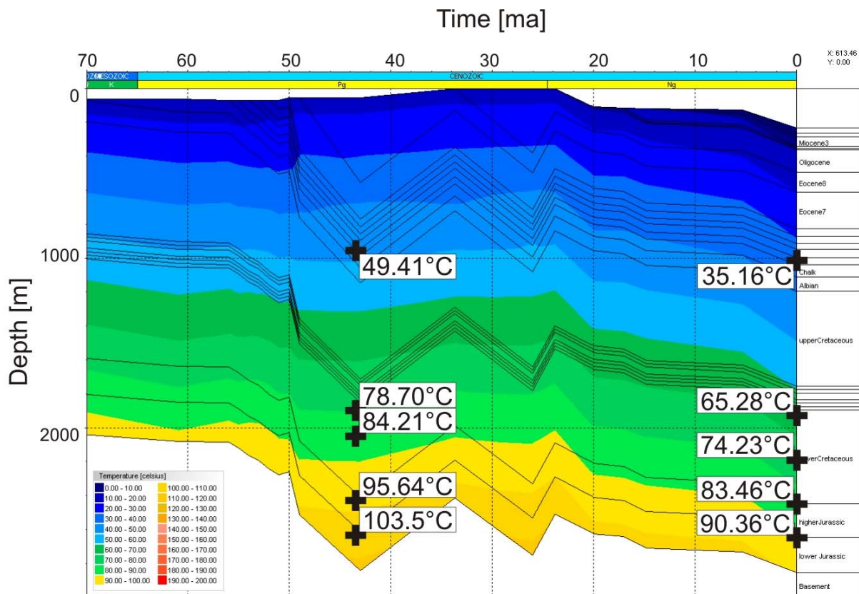
Figure 4-14: Modelled present and paleo temperatures (Paleocene) of well 26/28-1. Results at Paleocene time are influenced by the Iceland plume heat pulse and compared favourably to AFTA maximum paleotemperatures reported by McCulloch et al. (1993). Location of temperature points corresponds to McCullochs samples PB6 - PB10 from top to bottom, PB11 is of Carboniferous age and in the stratigraphic basement of the model.
