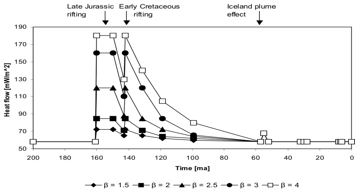
Figure 4-12: Heat flow depending on rifting events and stretching magnitude as described by the stretching value \beta (s. Figure 4-13)
