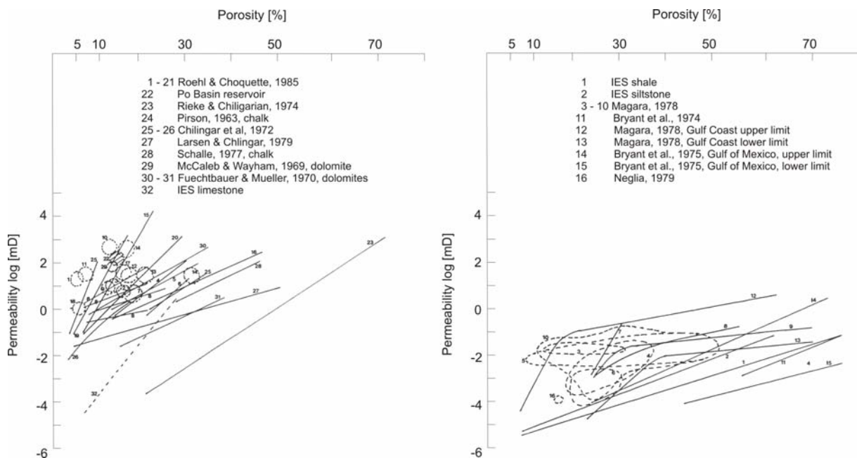
Figure 4-3: Porosity - permeability relationship for limestones and shales (Wygrala, 1989)
