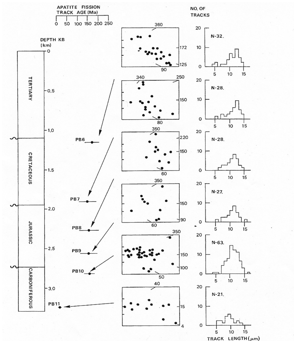
Figure 4-8: AFTA-data (McCulloch, 1993)
