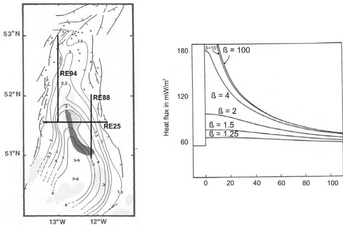
Figure 4-13: \beta - factor map of Tate et al. (1993) with modelled line locations and the modified McKenzie (1978) stretching factor – heat flow relationship
