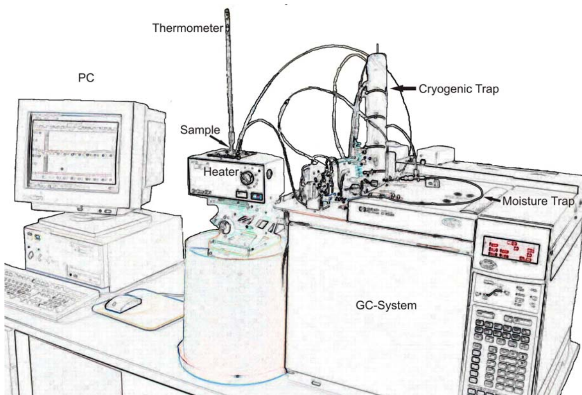
Figure 3-10: Dynamic headspace system
