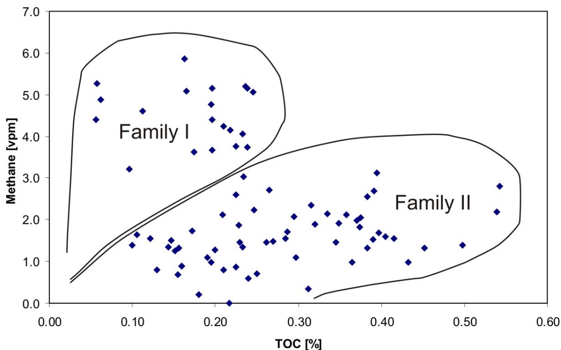
Figure 5-3: Relationship between TOC content and methane content
