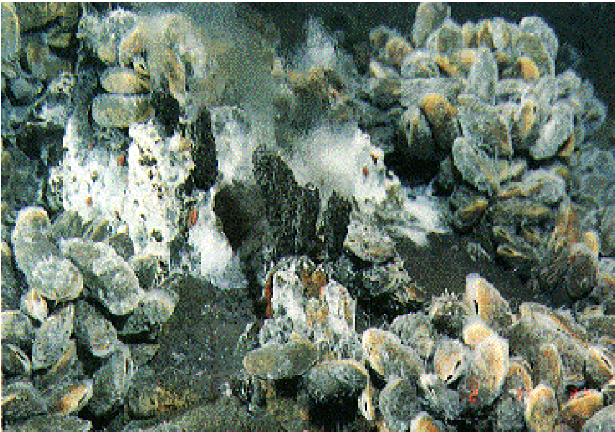
Figure 1-3: Chimney and hydrothermal vent community at Suiyo seamount, Izu-Ogasawara (Bonin) Islands, 1400 m deep (Jamstec, 2003)
