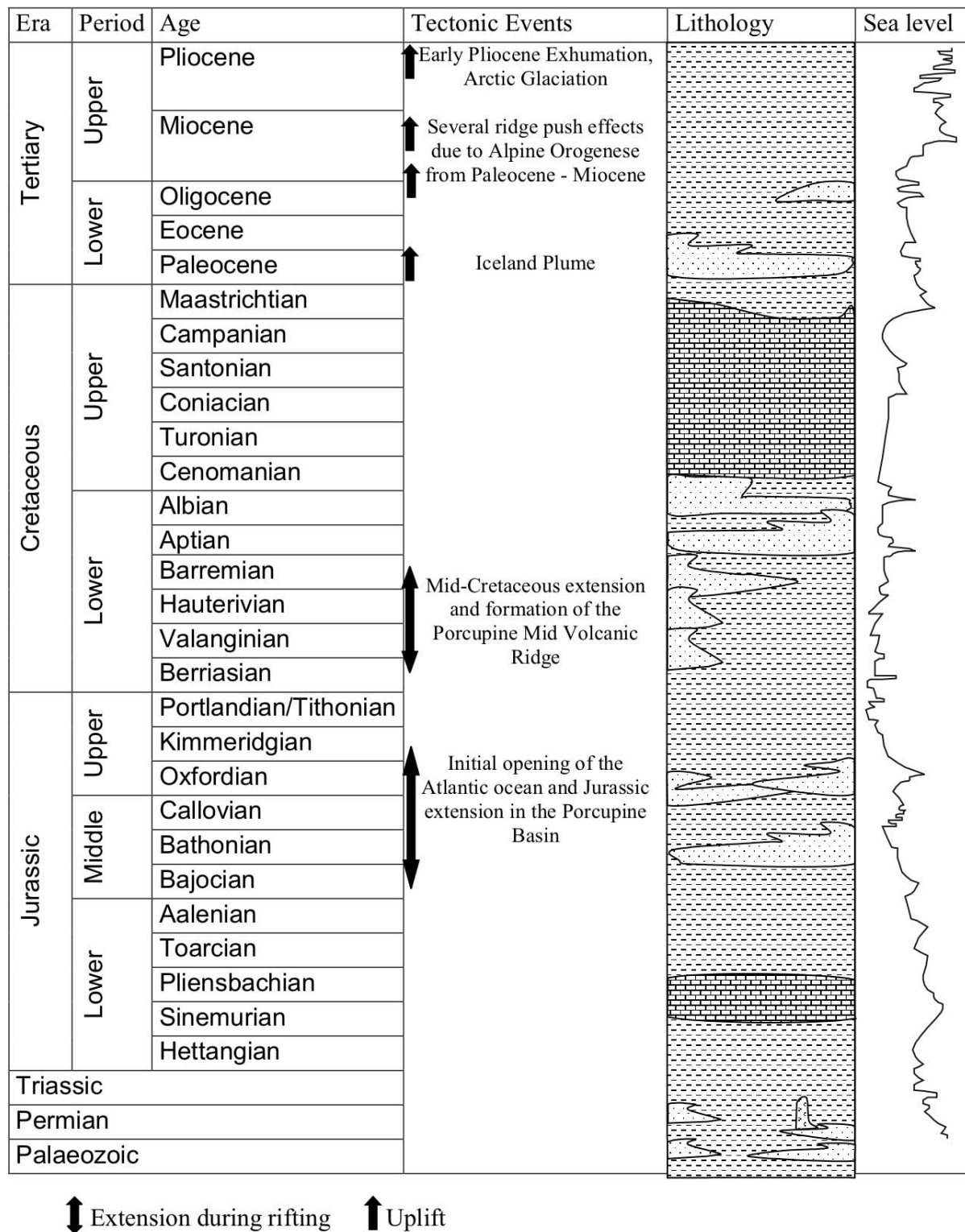
Figure 2-3: Schematic stratigraphy of the Porcupine Basin
