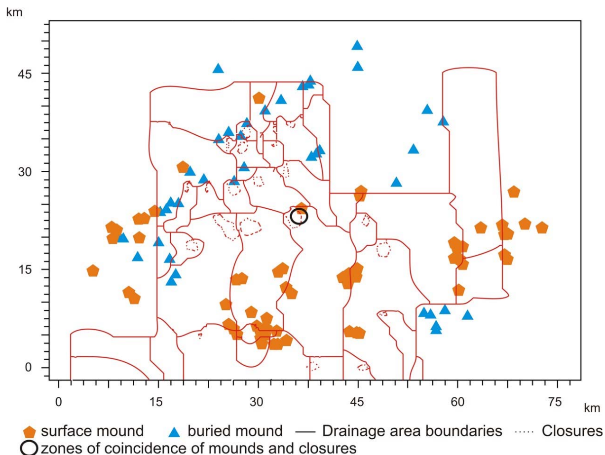
Figure 4-53: Results from the drainage area analysis for the C10 - map
