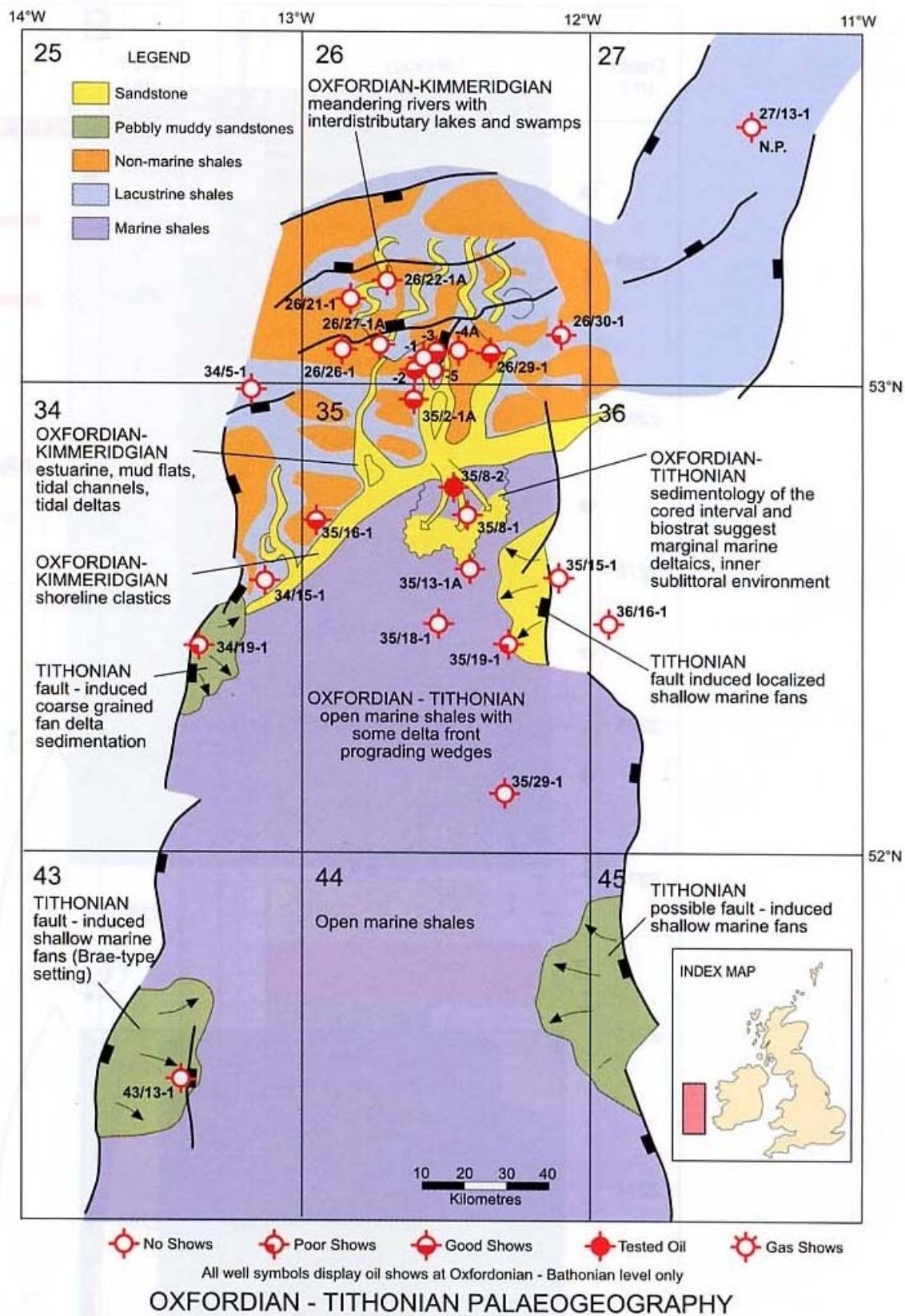
Figure 2-5: Generalized Late Jurassic paleogeographical reconstructions of the Porcupine Basin (Butterworth et al. 1999)
