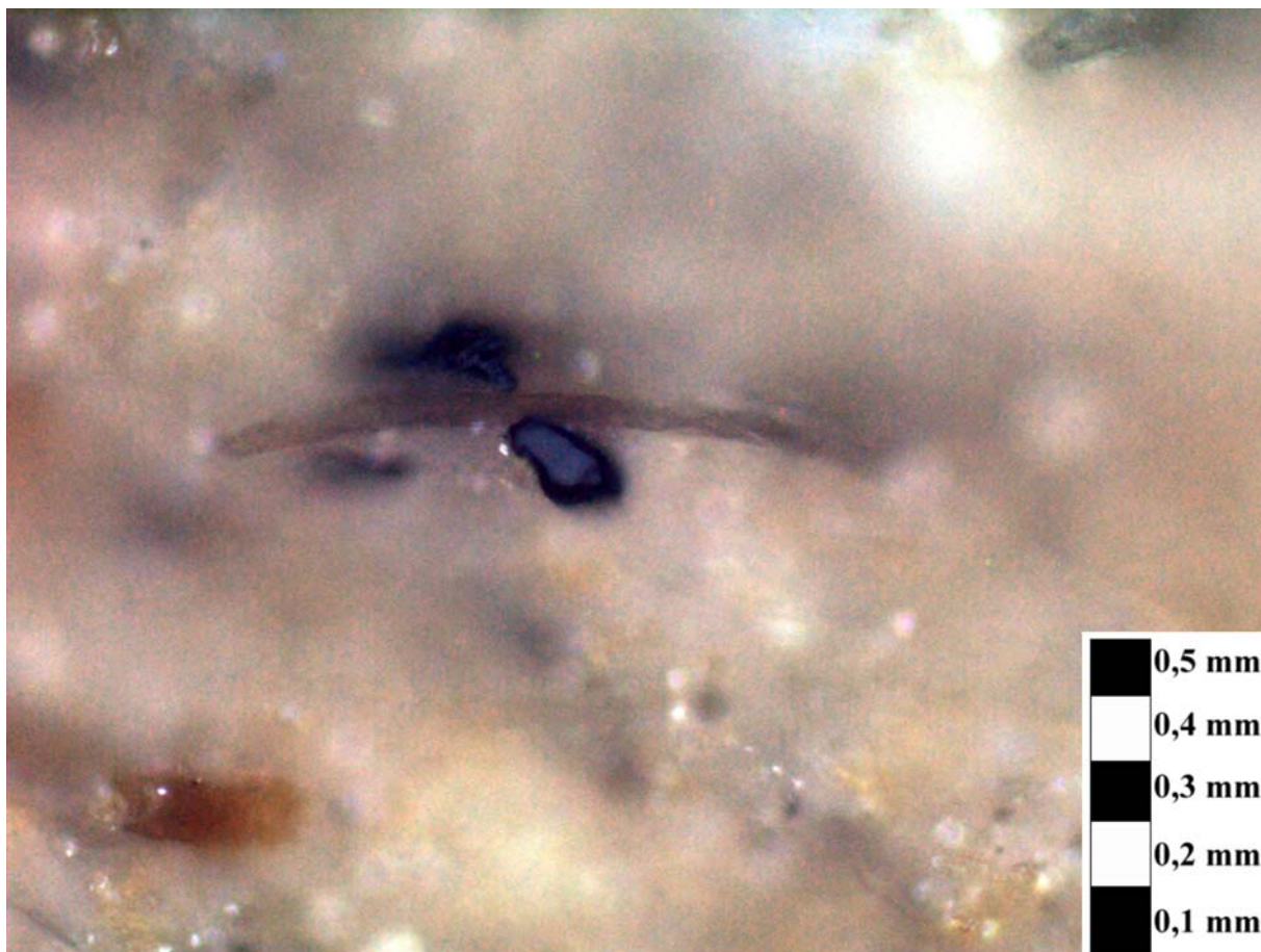
Figure 4-23: A microscopic view (600x magnification) of the Late Jurassic potential source rock sample 49728 showing a small vitrinite particle in the middle of the photo
