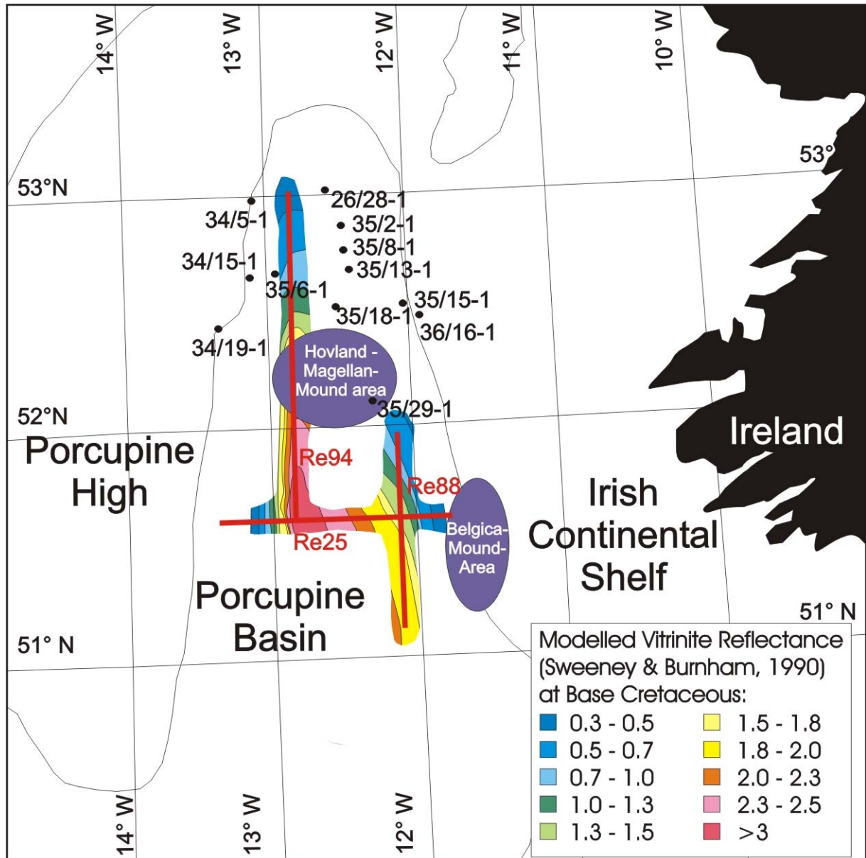
Figure 4-16: Maturity map of the Base Cretaceous based on the 2D modelling results of the profiles RE25, RE88 and RE94
