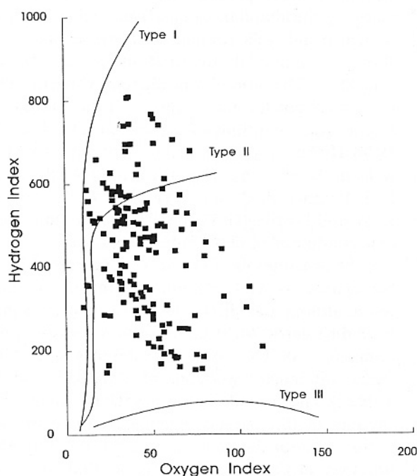
Figure 4-27: Source rock properties of the Egret Member
