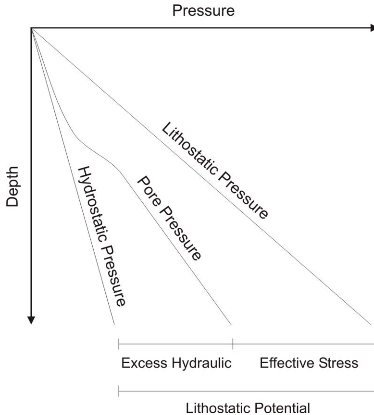
Figure 3-2: Relation between hydrostatic, pore and lithostatic pressure (modified after Welte et al., 1987)
