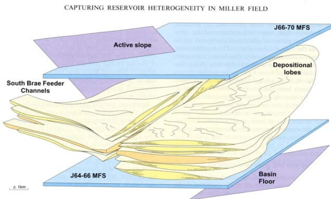
Figure 4-43: Miller fan schematic architecture (Garland et al. 1999)
