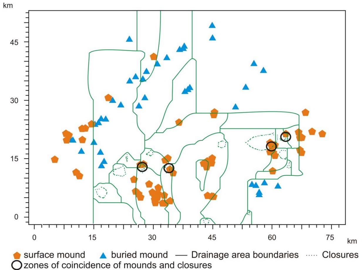
Figure 4-52: Results from the drainage area analysis for the C20 - map
