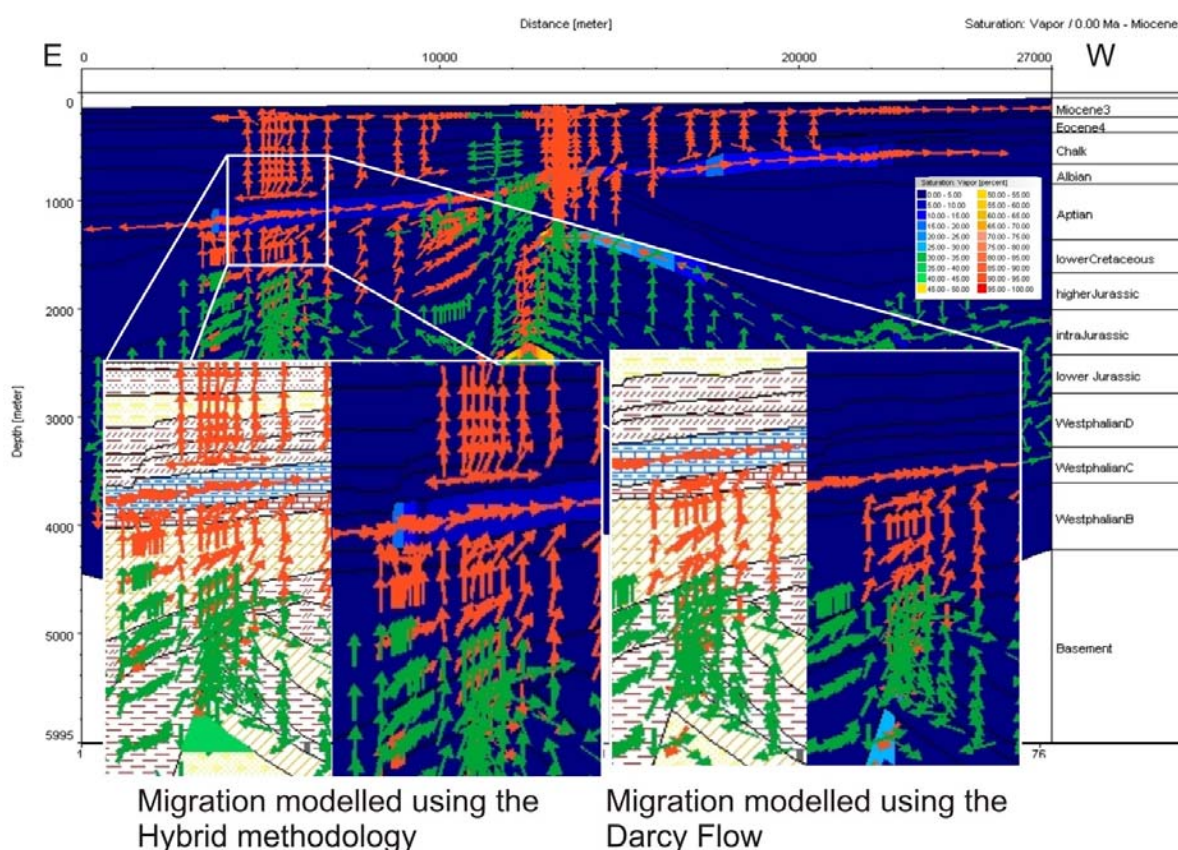
Figure 4-45: Migration modelled using hybrid and Darcy flow with gas saturation overlay
