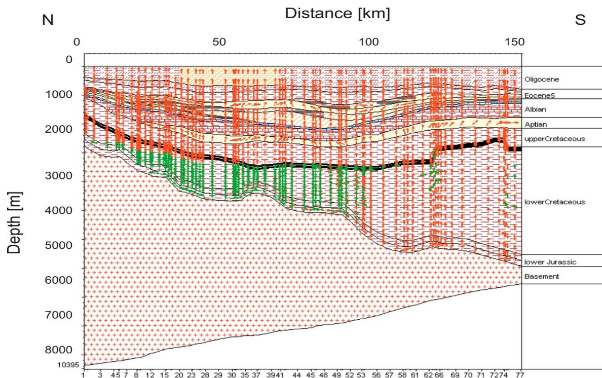
Figure 4-40: Oligocene configuration of modelled gas and oil flow along profile RE94
