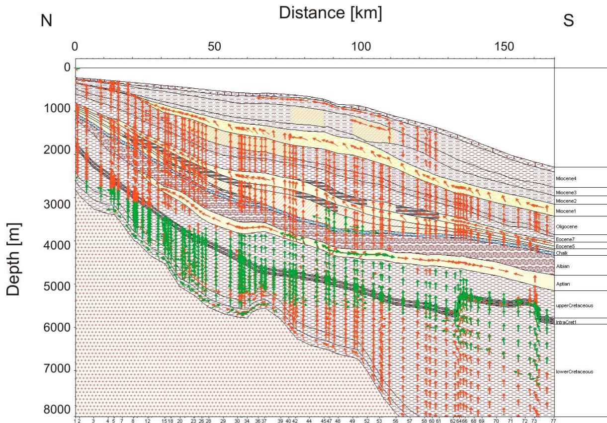
Figure 4-36: Present day configuration of modelled gas (red vectors) and oil (green vectors) flow along profile RE94
