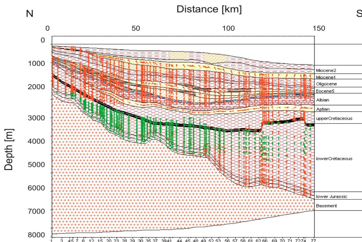
Figure 4-41: Miocene configuration of modelled gas and oil flow along profile RE94
