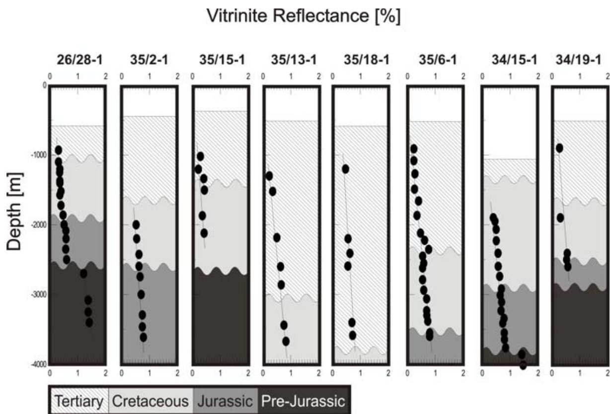
Figure 4-6: Vitrinite reflectance measured in wells close to Line RE94
