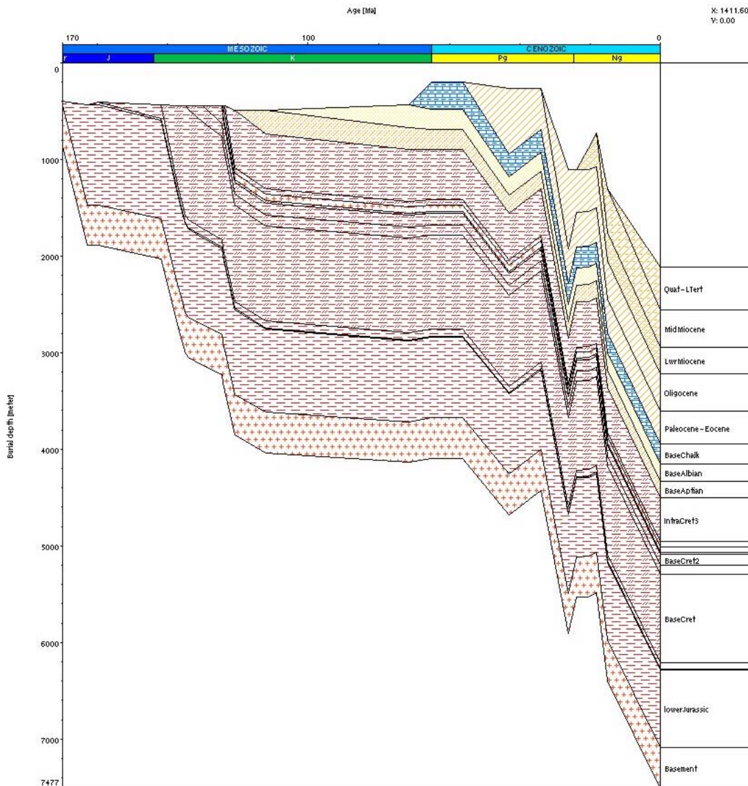
Figure 4-2: Burial history of profile RE94 at intersection with profile RE25
