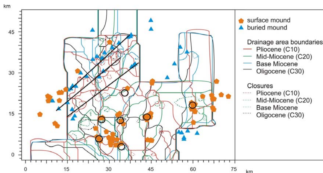
Figure 4-49: Results from the drainage area analysis, coincidence of surface mounds and closures are marked by black circles, the trend seen in the buried mounds is marked by the black lines.
