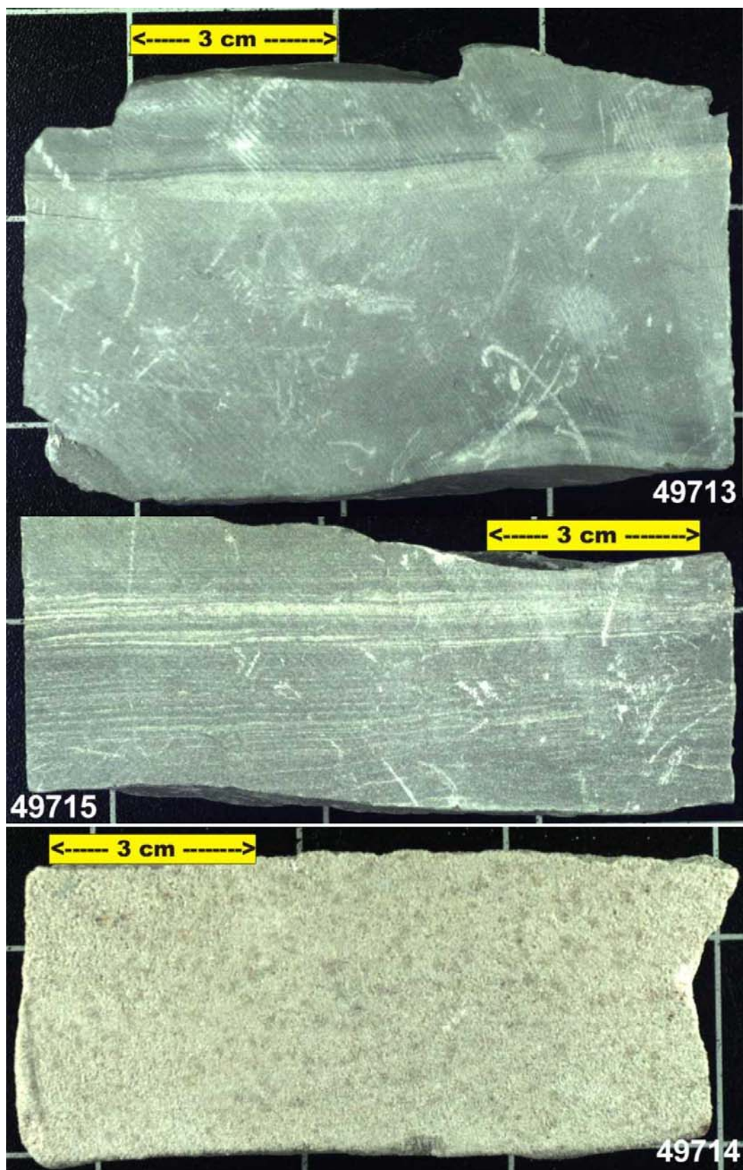
Figure 4-18: Lower Jurassic samples 49713, 49714 and 49715
