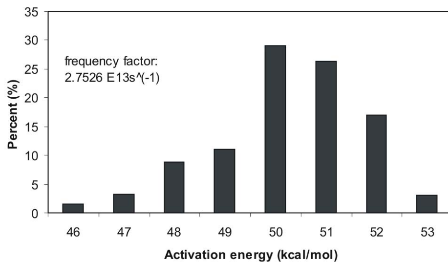
Figure 4-30: Distribution of asphaltene fraction for sample E49851
