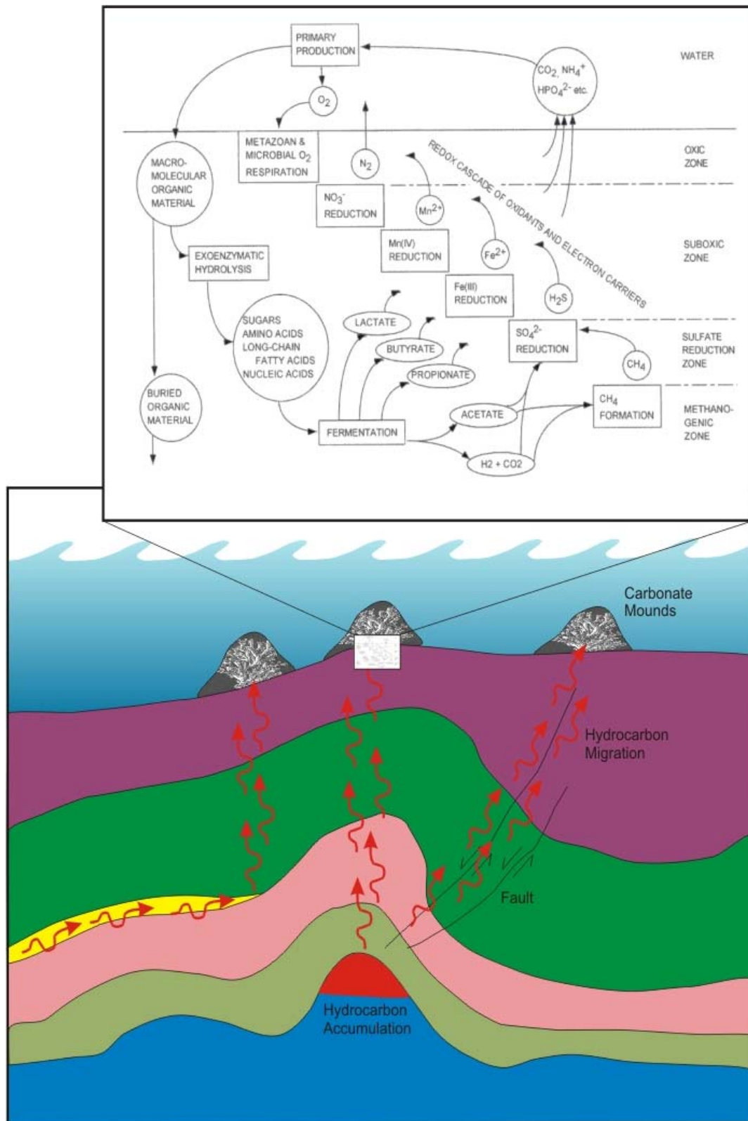
Figure 1-8: Carbonate mound formation mechanism based on focussed hydrocarbon flow through pinch outs, cap rock failure and faults. Hydrocarbon reduction pathways at the sediment water interface are stated on top modified from Boetius et al. (2002)
