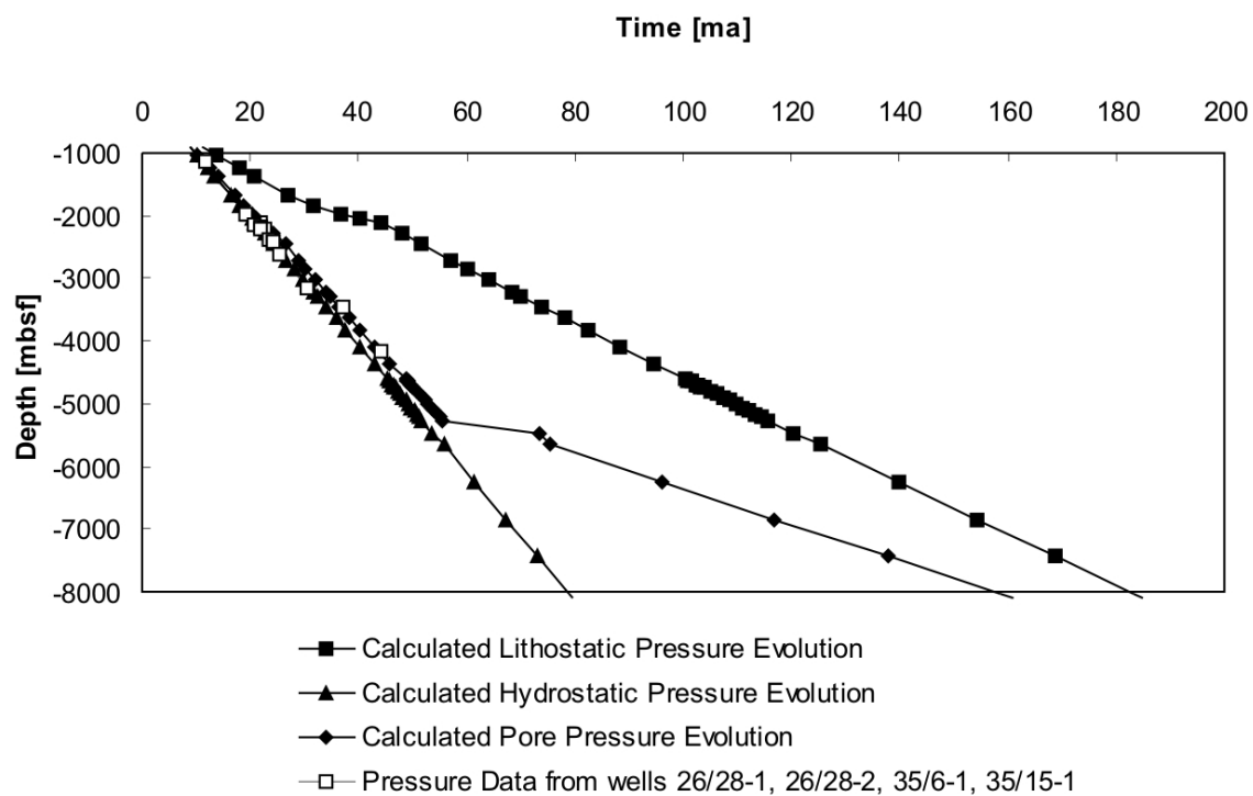
Figure 4-5: Pressure regime in the Porcupine Basin based on modelled lithostatic, hydrostatic and pore pressure as compared to the available calibration data
