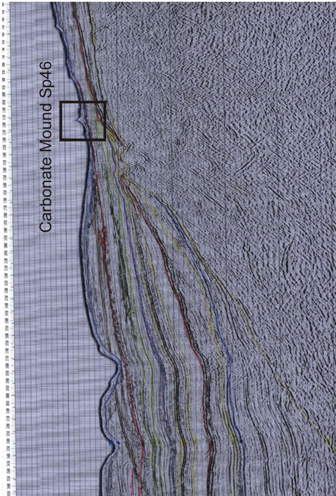
Figure 3-7: Profile PORC97-12 including carbonate mound SP46
