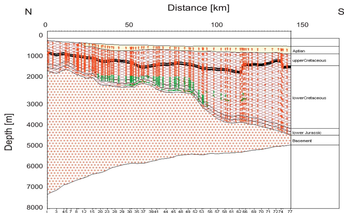
Figure 4-39: Aptian configuration of modelled gas and oil flow along profile RE94
