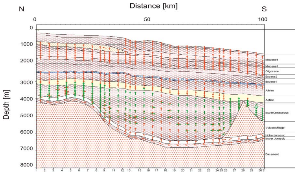
Figure 4-37: Present day configuration of modelled gas (red vectors) and oil (green vectors) flow along profile RE88
