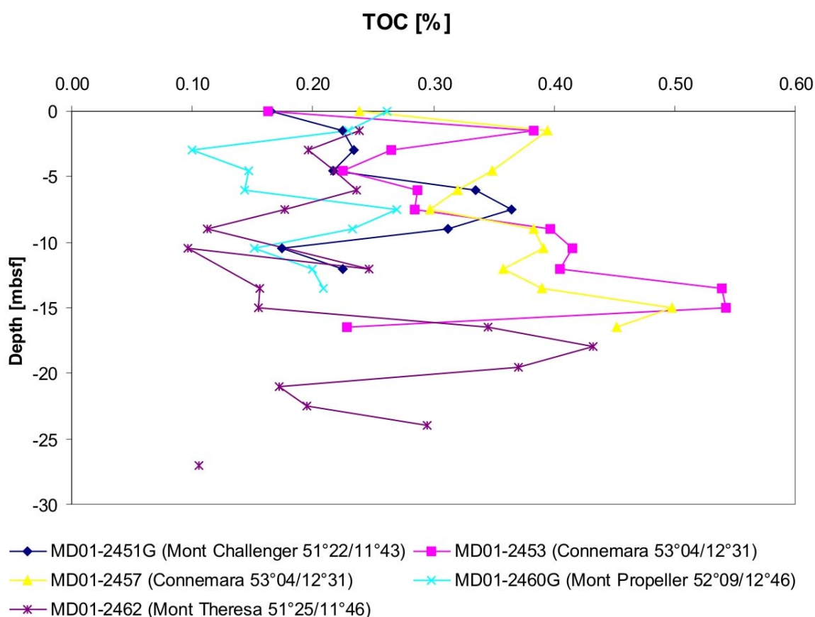
Figure 5-1: TOC plotted versus depth for the cores MD01-2451G, MD01-2453, MD01-2457, MD01-2460G and MD01-2462
