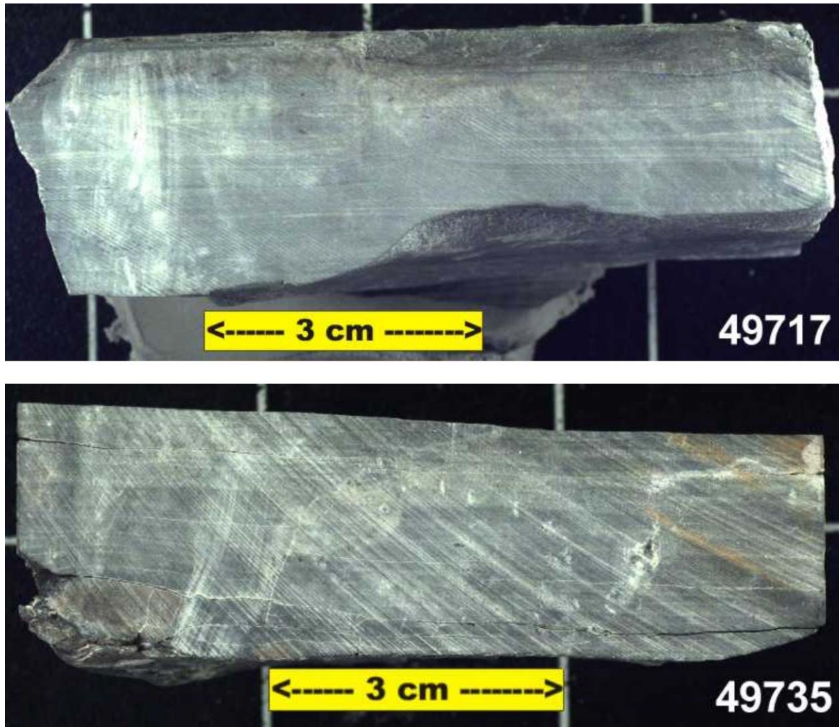
Figure 4-17: Carboniferous core samples 49717 and 49735
