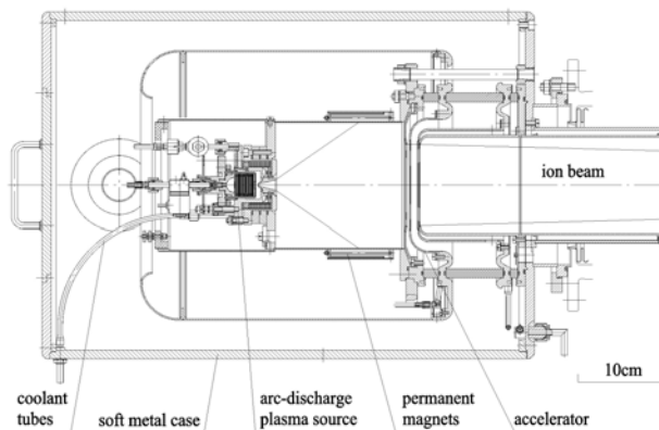
FIG. 4. Schematic view of ion source with an arc-discharge plasma box.
