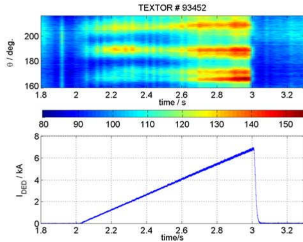
Fig. 2. Temporal evolution of a poloidal profile of D_\alpha emission across the DED target (top) and time trace of the DED current (bottom) in the 12/4 configuration ( I_p=450 kA / B_T=1.9 T, a=0.44 m, R=1.71 m).
