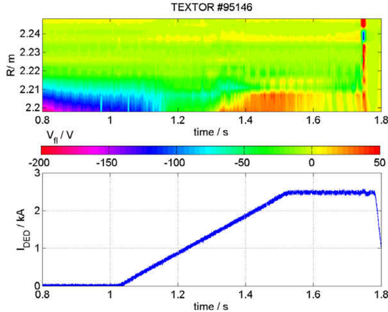
Fig. 9. Time evolution of the profile of the floating potential measured by a rake probe and time trace of the DED current (3/1 configuration, I_p = 260 kA, B_T = 1.89 T, a = 0.45 m, R = 1.76 m)
