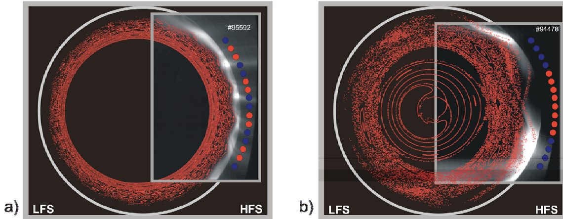
Fig.1. Divertor structure as seen in CIII light: a) example with 12/4 configuration, b) example with 3/1 configuration of the DED coils
