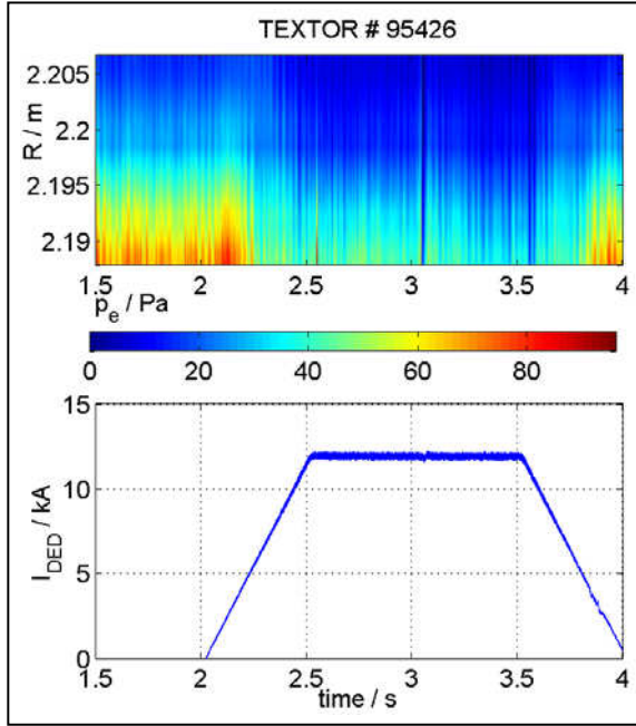
Fig.3. Temporal evaluation of the electron pressure profile at the LFS (top) and the time trace of the DED current (bottom) in the 12/4 configuration ( I_p = 350 kA, B_T = 1.9 T, a = 0.46 m, R = 1.75 m)
