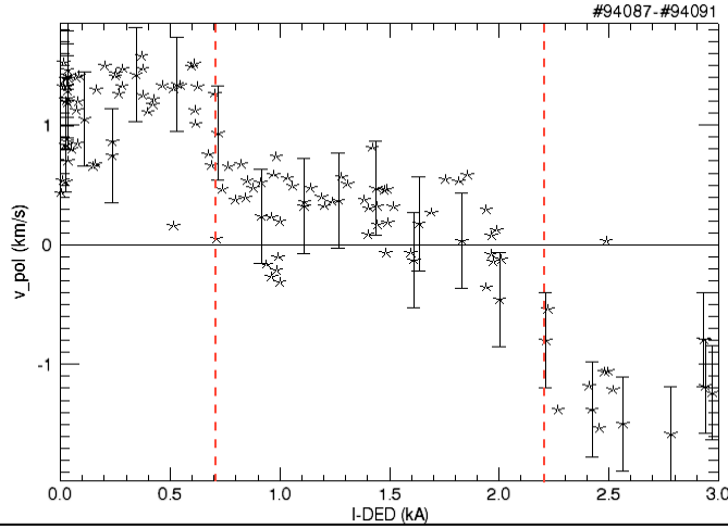
Fig. 8. Poloidal rotation deduced from the Doppler shift of C^{2+} ions as a function of the DED current in the 3/1 configuration ( I_p = 350 kA, B_T = 2.25 T, a = 0.46 m, R = 1.75 m).
