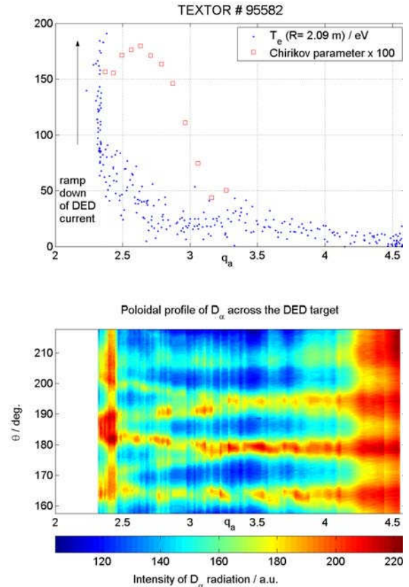
Fig.4. Electron temperature and Chirikov parameter at R = 2.09 m (top) and evolution of a poloidal profile of D_\alpha emission across the DED target (bottom) as a function of q_a (12/4 configuration, B_T = 1.9 T, I_p ramped from 200 – 400 kA, R = 1.68 m, a = 0.4 m).
