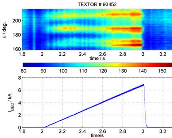
Fig. 2. Temporal evolution of a poloidal profile of D_\alpha emission across the DED target (top) and time trace of the DED current (bottom) in the 12/4 configuration ( I_p=450 kA / B_T=1.9 T, a=0.44 m, R=1.71 m).
