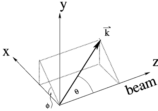
FIG. 4. The kaon momentum \vec{k} plotted in the coordinate system used; the z axis is along the beam direction.
