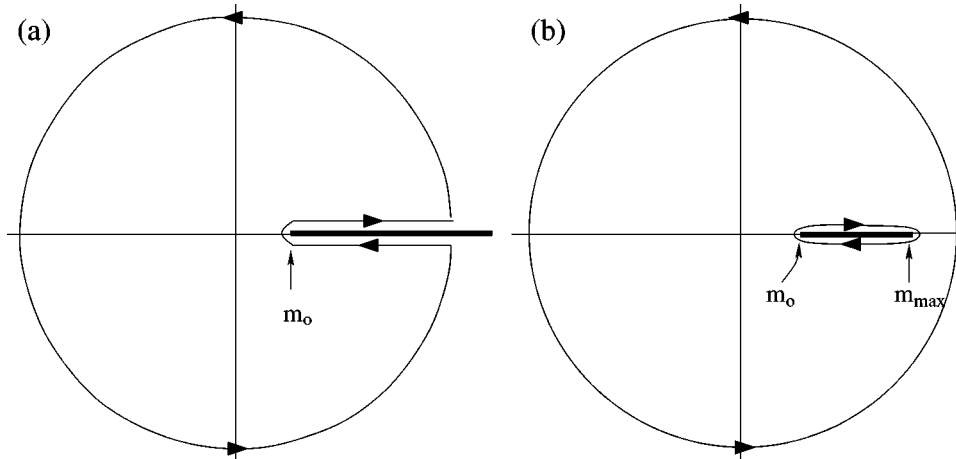
FIG. 1. The integration contours in the complex m'^2 plane to be used to derive Eq. (12) (a) and Eq. (17) (b). The thick lines indicate the branch cut singularities.
