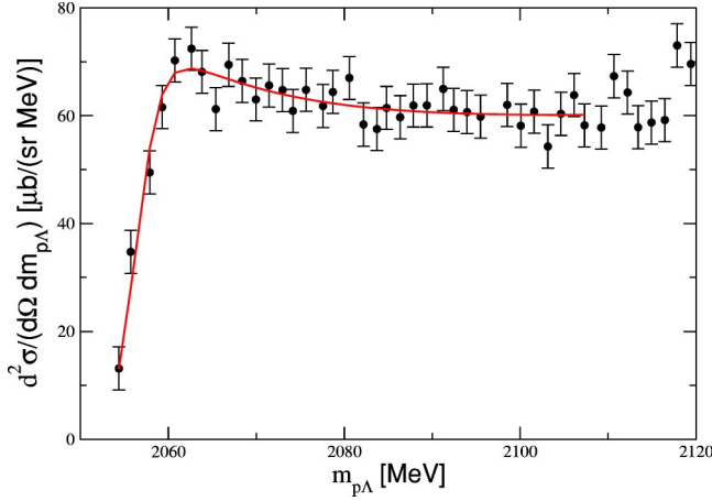
FIG. 3. pp \rightarrow K^+X inclusive missing mass spectrum at T_p = 2.3 GeV for kaon laboratory scattering angles \theta_K^L = 10 \pm 2^\circ [38]. The solid line is our fit as described in the text. Note that the scattering length extracted is insensitive to the parametrization of the data used (see Appendix A for details).
