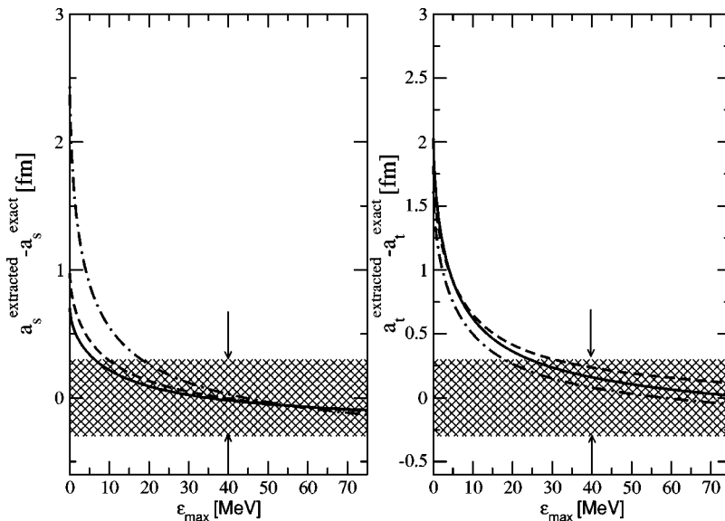
FIG. 2. Dependence of the extracted scattering lengths on the value of the upper limit of integration, \epsilon_{\max} . Shown is the difference from the exact results for the spin-singlet scattering length a_s (left panel) and the spin-triplet scattering length a_t (right panel). The solid and the dot-dashed lines correspond, respectively, to model NSC97a and NSC97f of Ref. [5] and the dashed one corresponds to the YN model of Ref. [6]. The shaded area indicates the estimated error of the proposed method and the arrows indicate the value for \epsilon_{\max} as estimated based on scale arguments.
