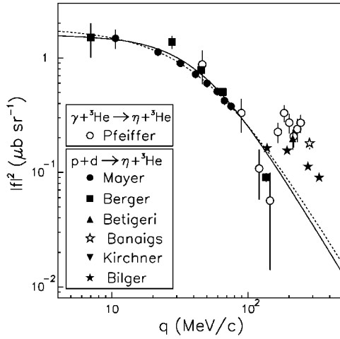
FIG. 2. Spin and angle averaged transition amplitudes |f|^2 extracted from \gamma^3\text{He} \rightarrow \eta^3\text{He} [19] and pd \rightarrow \eta^3\text{He} [3,18,20–23] data as functions of the final momentum q in the c.m. system. The |f|^2 from coherent photoproduction was arbitrarily multiplied by a factor of 6. The solid line is our overall fit [5] to low-energy data from Mayer et al. [3] and Berger et al. [18], while the dashed line shows our fit to the data from Mayer et al. [3] alone.
