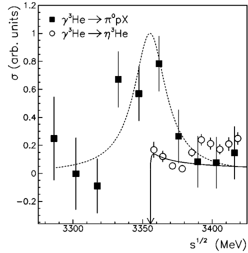
FIG. 3. The \gamma^3\text{He} \rightarrow \eta^3\text{He} cross section (open circles) and the difference between the \gamma^3\text{He} \rightarrow \pi^0 pX reaction for 170^\circ \leq \theta_{\pi^0 p} \leq 180^\circ and that for 150^\circ \leq \theta_{\pi^0 p} \leq 170^\circ (solid squares) as a function of the invariant collision energy \sqrt{s} . The arrow indicates the \eta production threshold. The dashed curve is a fit to the data based on Eq. (9) and the solid curve is the result based on Eq. (7), employing the amplitude shown in Fig. 2 (solid line).
