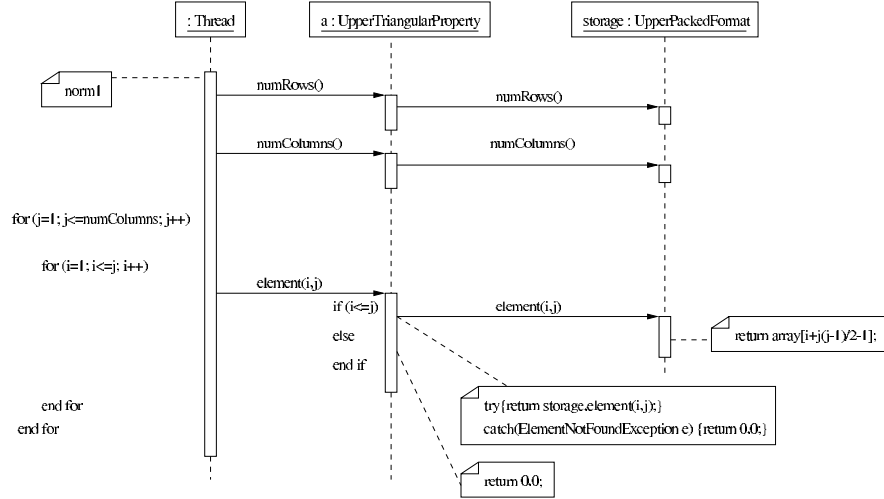
Fig. 14. Sequence diagram for \|A\|_1 implemented at MA-level with A upper triangular and stored in packed format.
