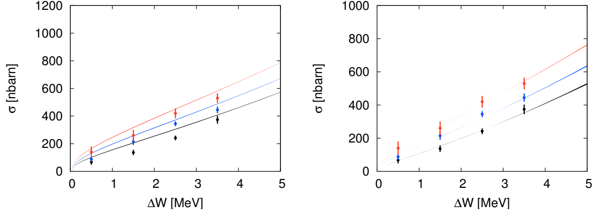
Fig. 10. Left panel: Total cross section as a function of \Delta W for three different values of the photon polarization in comparison to the MAMI data [1] for fit 1 and the NNLO wave functions. The upper/middle/lower band corresponds to the largest/medium/smallest value of \varepsilon . Right panel: Same for fit 2.
