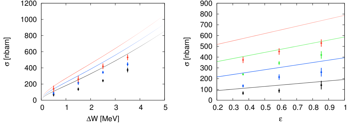
Fig. 6. Left panel: Total cross section as a function of \Delta W for three different values of the photon polarization in comparison to the MAMI data [1] for fit 1 and the NNLO wave functions. The upper/middle/lower band corresponds to the largest/medium/smallest value of \epsilon . Right panel: Total cross section as a function of the photon polarization \epsilon for four different values of the pion excess energy \Delta W . The highest band corresponds to the largest value of \Delta W and correspondingly for the other bands/values of \Delta W .
