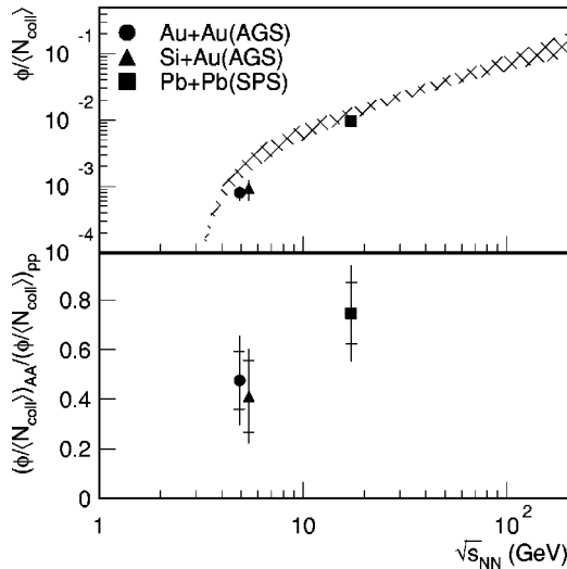
FIG. 13. Same as Fig. 10 for the ratios of \phi/\langle N_{\text{coll}} \rangle , where \langle N_{\text{coll}} \rangle is the number of binary collisions. For the E917 data point, an estimated total \phi yield is plotted as described in the text.
