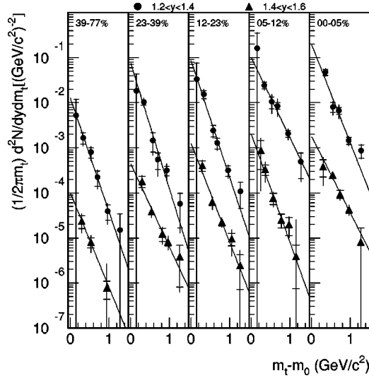
FIG. 4. The invariant yield of \phi 's as a function of transverse mass ( m_t - m_0 ) in five centrality bins labeled by \sigma/\sigma_{\text{tot}} . In each panel, the top set of points (circles) is for 1.2 < y < 1.4 , while the second set of points (triangles) is for 1.4 < y < 1.6 and is divided by 100 for presentation. The total errors are calculated as the quadrature sum of the systematic and statistical errors, while the magnitudes of the latter are indicated by the cross bars. The lines are the results of the exponential fits described in the text.
