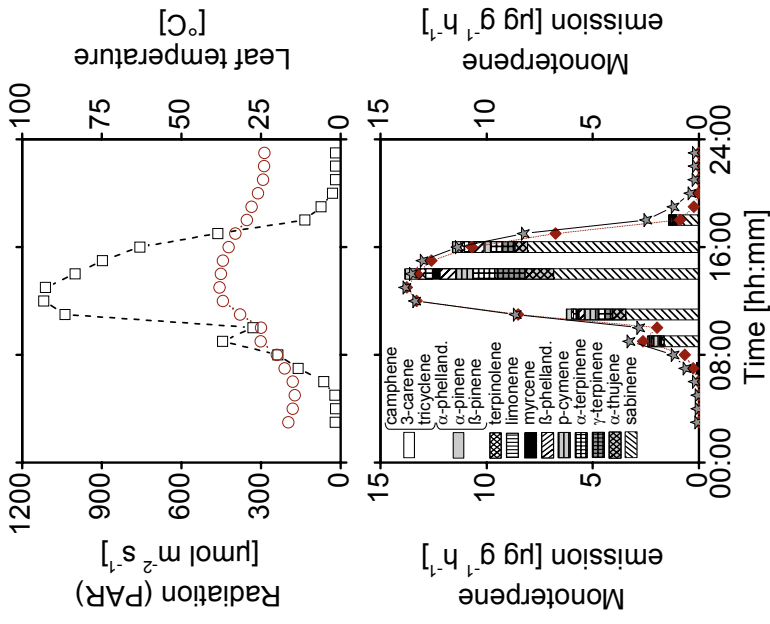
Fig. 6. Course of photosynthetic active radiation (PAR), leaf temperature, and monoterpene emission measured during one single day in August 2003. Top graph: Diurnal course of PAR (black squares plus dashed line) and leaf temperature (red circles plus dotted line). Data show the appropriate 30 min average during that VOC cartridges were collected. Bottom graph: Diurnal course and composition of monoterpene emission. Data show monoterpene emission measured by GC-MS analysis (stacked bars, for caption see graph), the respective emission calculated by the G97 algorithm (grey stars plus solid line), and the S97 algorithm (emission from biosynthesis only, red diamonds plus dotted line).
