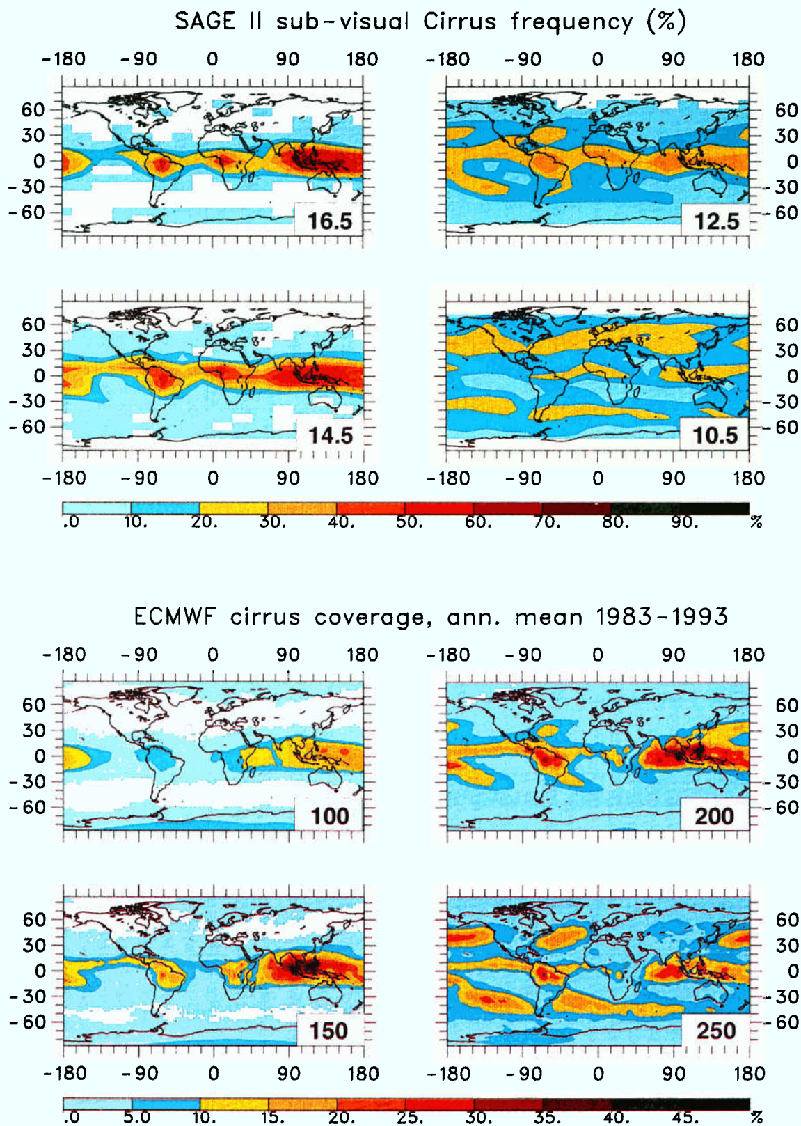
Plate 2. (top) Global distribution of frequency of occurrence of SVC from SAGE II data and (bottom) the ECMWF fractional coverage of cirrus for different altitudes: comparable altitudes are 16.5 km with 100 hPa, 14.5 km with 150 hPa, 12.5 km with 200 hPa, and 10.5 km with 250 hPa.
