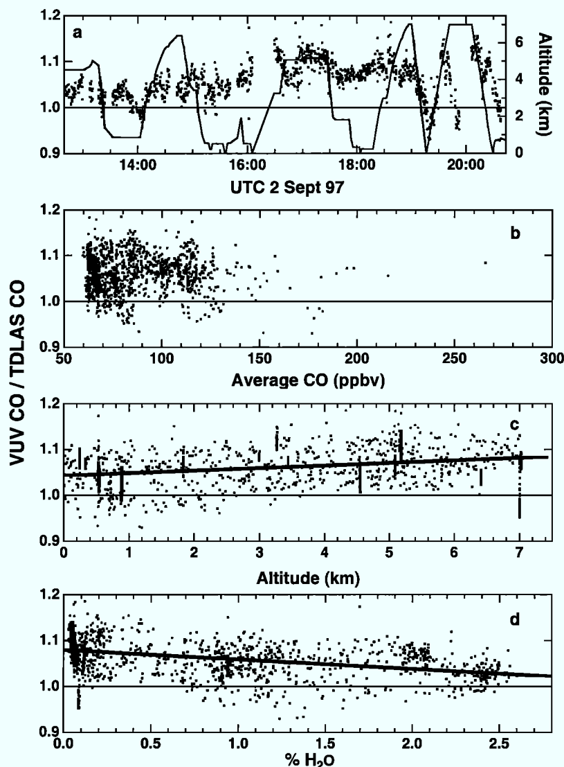
Figure 6. Ratio of coincident 5 s average CO measurements as a function of (a) time, (b) average CO concentration, (c) aircraft altitude, and (d) ambient water vapor. Linear least square fits are shown for the altitude and water vapor plots. The aircraft altitude is included as a solid line in Figure 6a.
