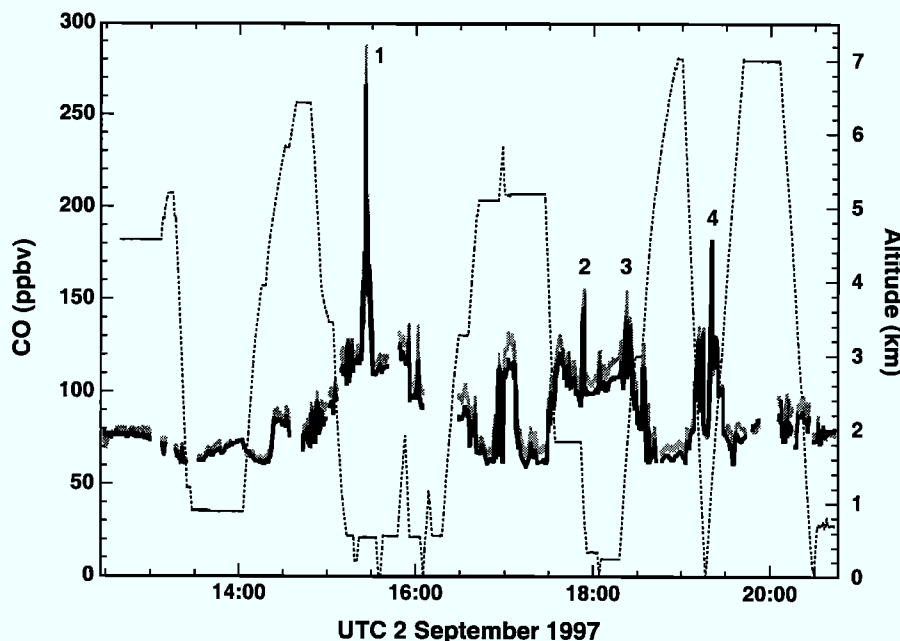
Figure 4. Time series of coincident 5 s average measurements of CO on the NOAA WP-3 transit flight. The solid lines give the TDLAS (darker) and the VUV fluorescence (lighter) results, and the dotted line indicates the aircraft altitude. The features labeled 1 through 4 are intercepted urban plumes.
