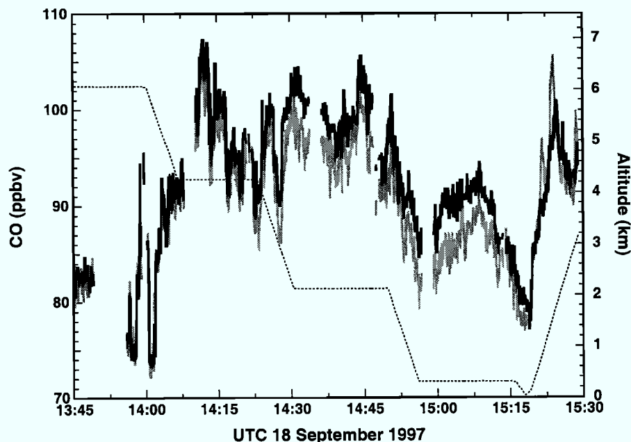
Figure 7. Time series of coincident 5 s average measurements of CO during the VUV instrument intercomparison. The solid lines give the C-130 (darker) and the WP-3 (lighter) results, and the dotted line is the aircraft altitude.
