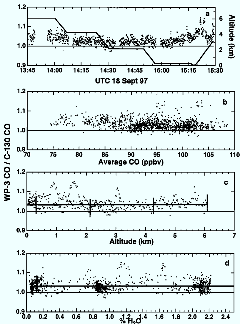
Figure 9. Ratios of coincident 5 s average CO measurements as a function of (a) time, (b) average CO concentration, (c) aircraft altitude and (d) ambient water vapor. Linear least square fits are shown for the altitude and water vapor plots. The aircraft altitude is included as a solid line in Figure 9a. Average values of the CO measurement ratio and water vapor concentration for constant altitude flight legs are indicated by the crosses.
