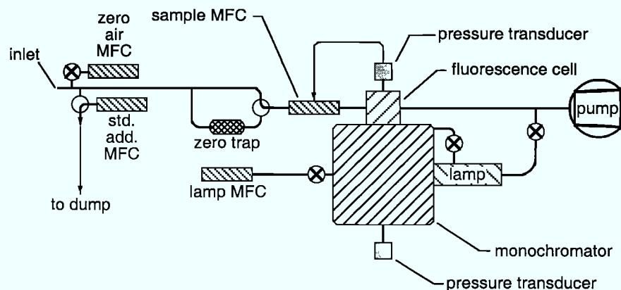
Figure 2. Schematic of the NOAA WP-3 VUV CO fluorescence instrument. MFC represents mass flow controller.
