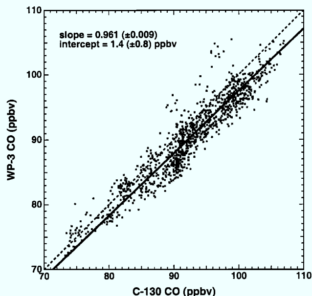
Figure 8. Correlation of the 5 s average measurements from the VUV instrument intercomparison. The dashed line gives the one to one correspondence. The solid line is the bivariate linear regression fit to the data; the parameters of this fit (with 2\sigma confidence limits) are given in the legend.
