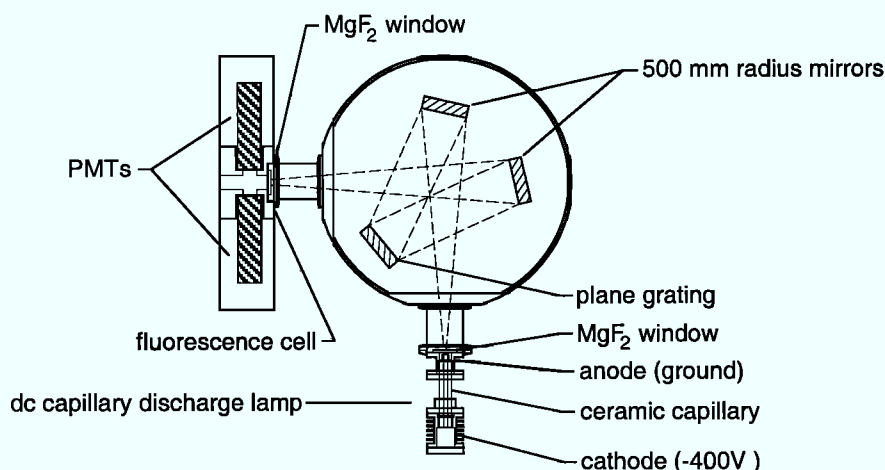
Figure 1. Schematic of the fluorimeter of the NOAA WP-3 VUV CO fluorescence instrument.
