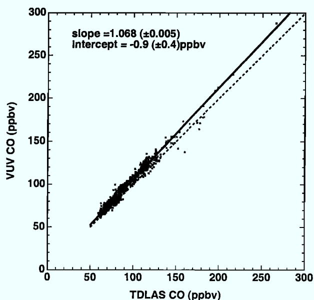
Figure 5. Correlation of the 5 s average measurements from the NOAA WP-3 transit flight. The dashed line gives the one to one correspondence. The solid line is the bivariate linear regression fit to the data; the parameters of this fit (with 2 s confidence limits) are given in the legend.
