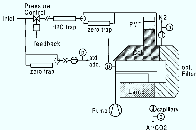
Figure 3. Schematic of Jülich C-130 VUV CO fluorescence instrument.
