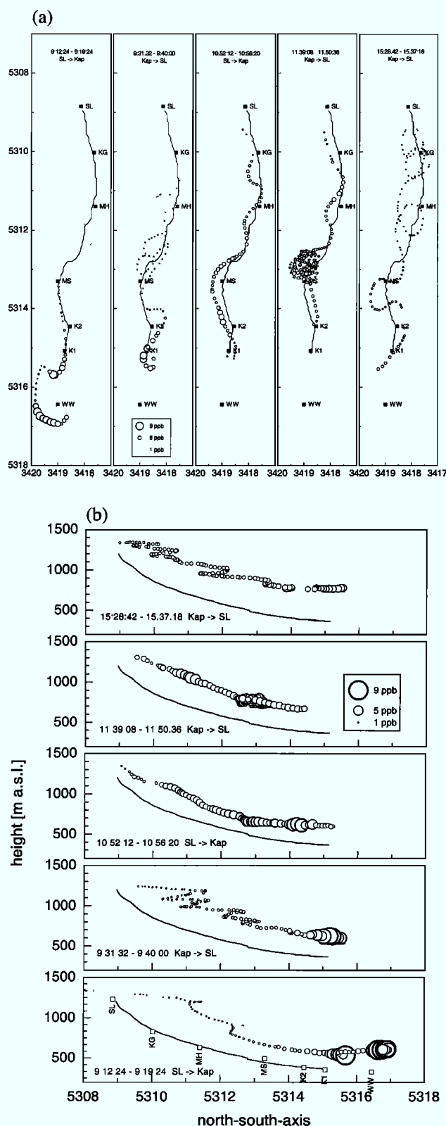
Figure 10. Concentrations of NO 2 on June 5 along the flight pattern of the motor glider: (a) displayed horizontally on a map and (b) displayed as vertical cross section along the valley axis. The diameters of the “bubbles” are proportional to the NO 2 mixing ratio. The ground-based sites are shown according to the notation in Table 1.
