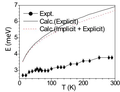
FIG. 7. (Color online) Comparison of the calculated and experimental temperature dependences of M_3 mode in \text{ReO}_3 . At T=0 K the harmonic value of M_3 mode is 2.8 meV.
