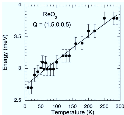
FIG. 2. Temperature dependence of the M_3 phonon mode in \text{ReO}_3 . The continuous curve is a guide to the eye.
