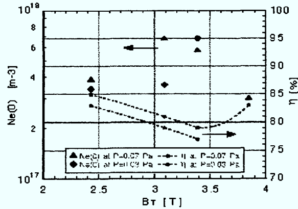
Fig.2. Central line-averaged RF plasma density n_0 and antenna-plasma coupling efficiency \eta versus toroidal magnetic field B_T ( P_{rf}\approx 150 kW, other parameters are mentioned in Fig.1).
