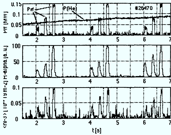
Fig.1. ICRF plasma production in helium: Q5-antenna in 0-phasing, P_{rf}=40\text{--}150 kW, \tau_{rf}\approx 40\text{--}50 ms, f=47.9 MHz, B_T=3.09 T.
