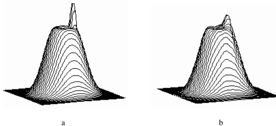
Fig. 3. (a) Exact model of an intensity distribution with a local disturbance (b) Tomogram reconstructed with maximum entropy algorithm for 5 projections, 100 chords in each projection
